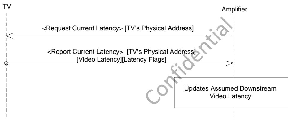
Figure 10-13: TV reports current latency value(s) and flags upon request
