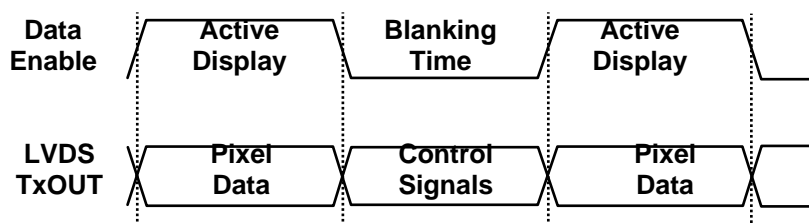
Figure 39 OpenLDI Synchronization
