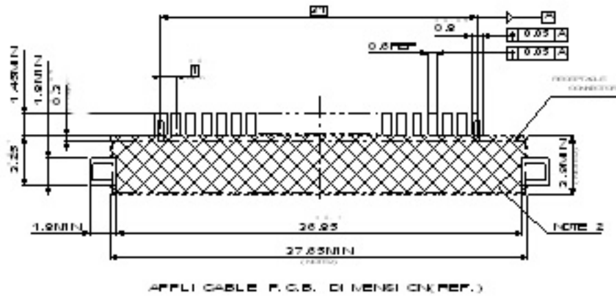
Figure 4-26: PCB Mount Connector Recommended Footprint Layout (in unit of mm)
