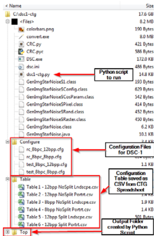
Figure 5-4: DSC CTG Buffer Conformance Tool Python Script Folder Structure
