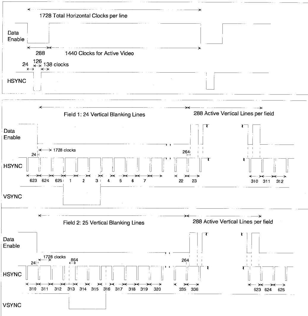
Figure 9 Timing Parameters for 720(1440)x576i @ 50 Hz
