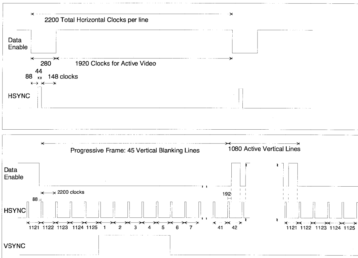
Figure 22 Timing Parameters for 1920x1080p @ 29.97/30 Hz
