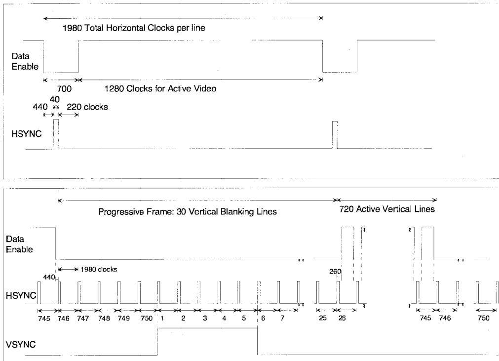
Figure 6 Timing Parameters for 1280x720p @ 50 Hz
