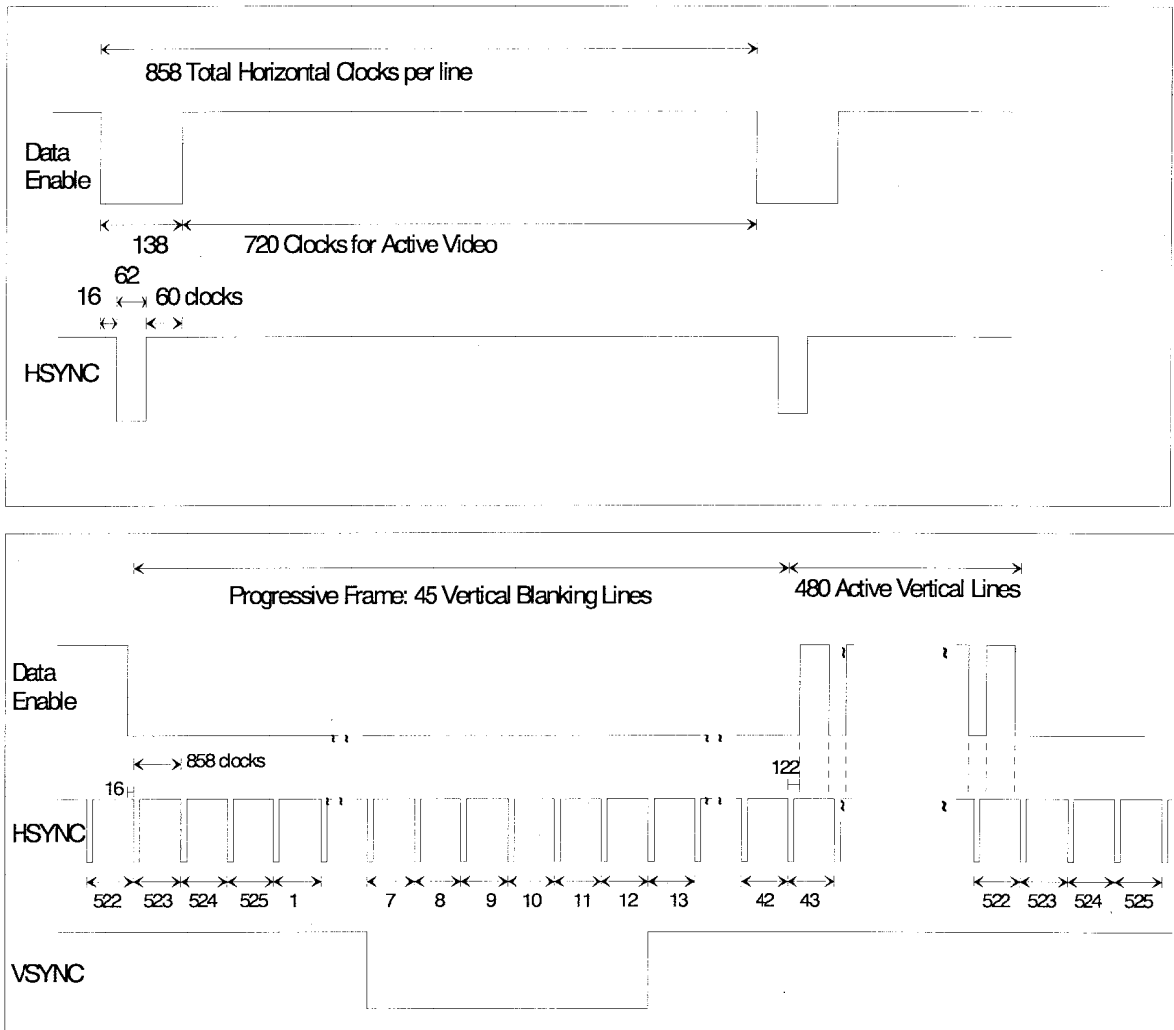
Figure 4 Timing Parameters for 720x480p @ 59.94/60 Hz
