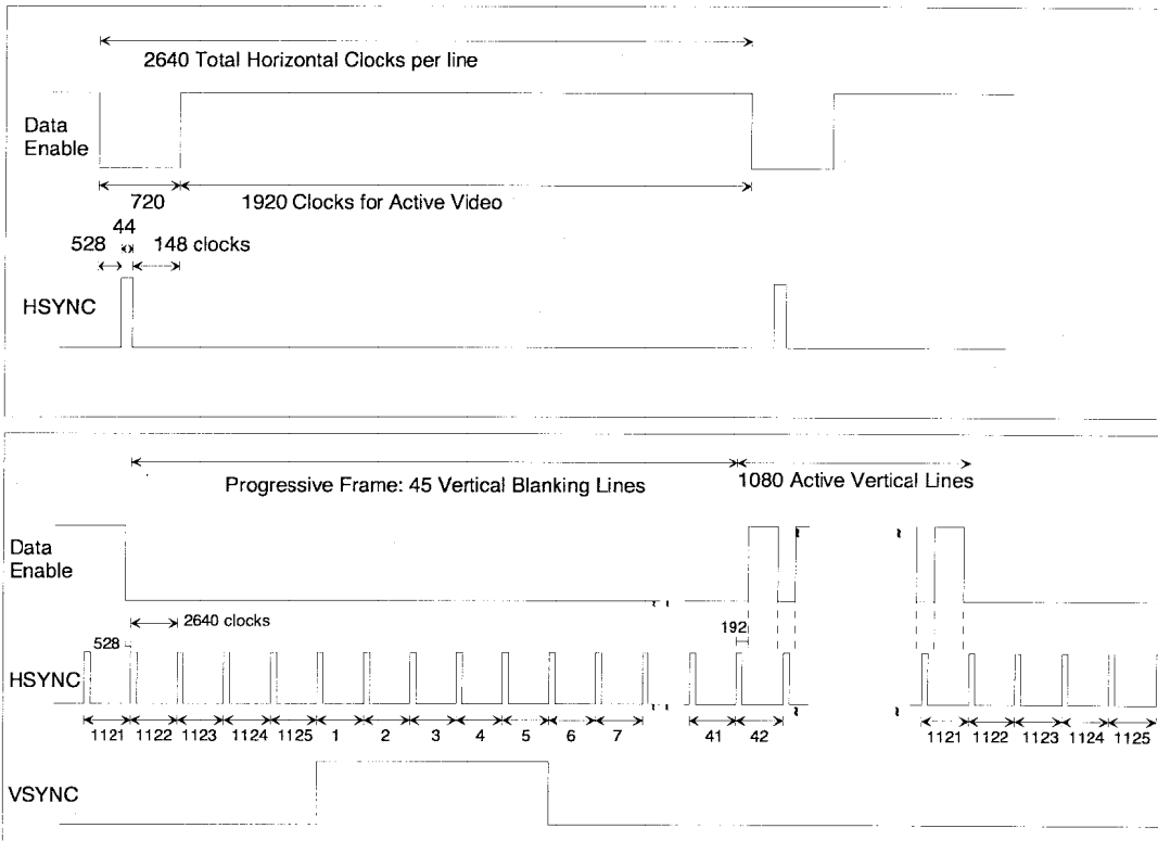
Figure 21 Timing Parameters for 1920x1080p @ 25 Hz
