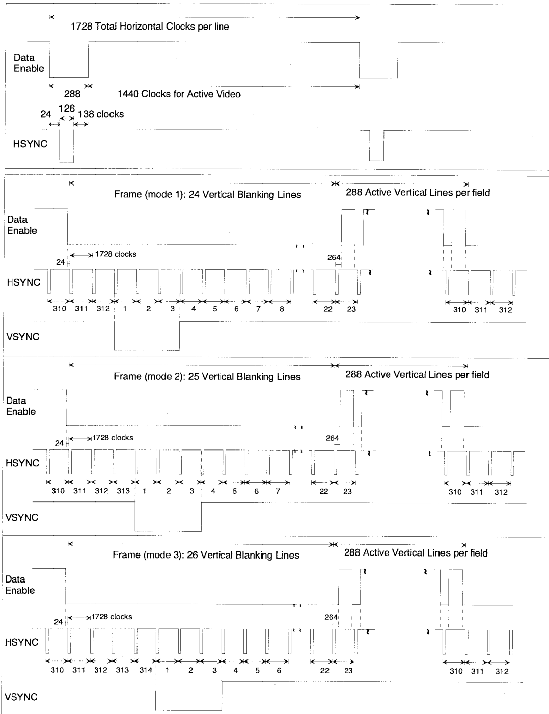
Figure 15 Timing Parameters for 720(1440)x288p @ 50 Hz
