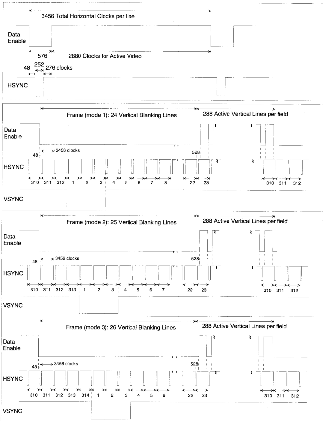
Figure 17 Timing Parameters for (2880)x288p @ 50 Hz
