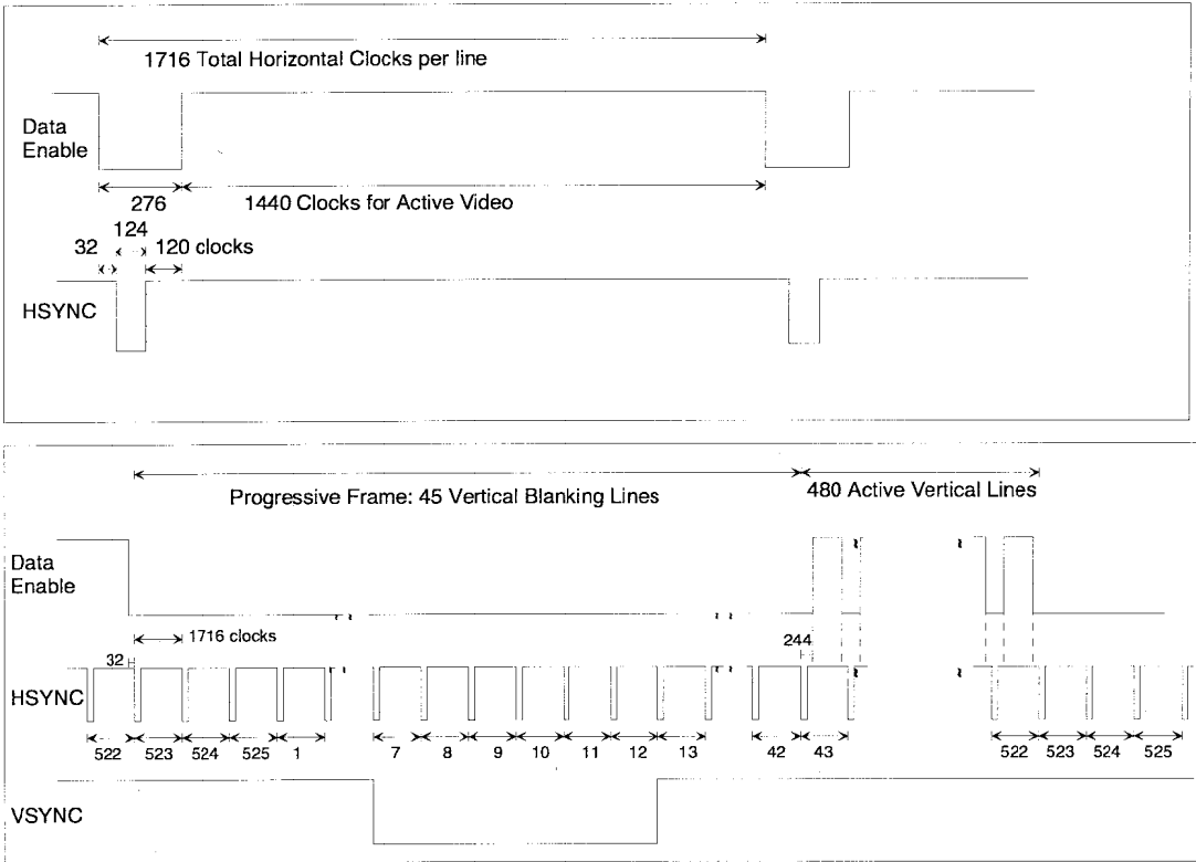
Figure 13 Timing Parameters for 1440x480p @ 59.94/60 Hz
