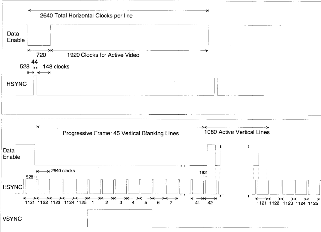
Figure 19 Timing Parameters for 1920x1080p @ 50 Hz
