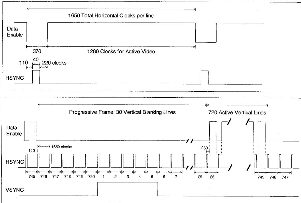
Figure 31 Timing Parameters for 1280x720p @ 119.88/120 Hz
