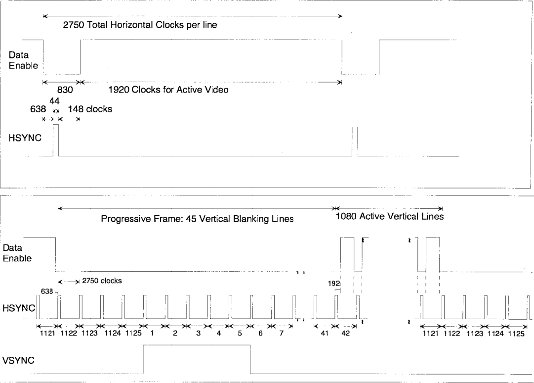
Figure 20 Timing Parameters for 1920x1080p @ 23.98/24 Hz
