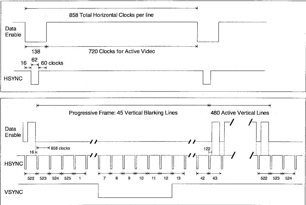
Figure 36 Timing Parameters for 720x480p @ 239.76/240 Hz
