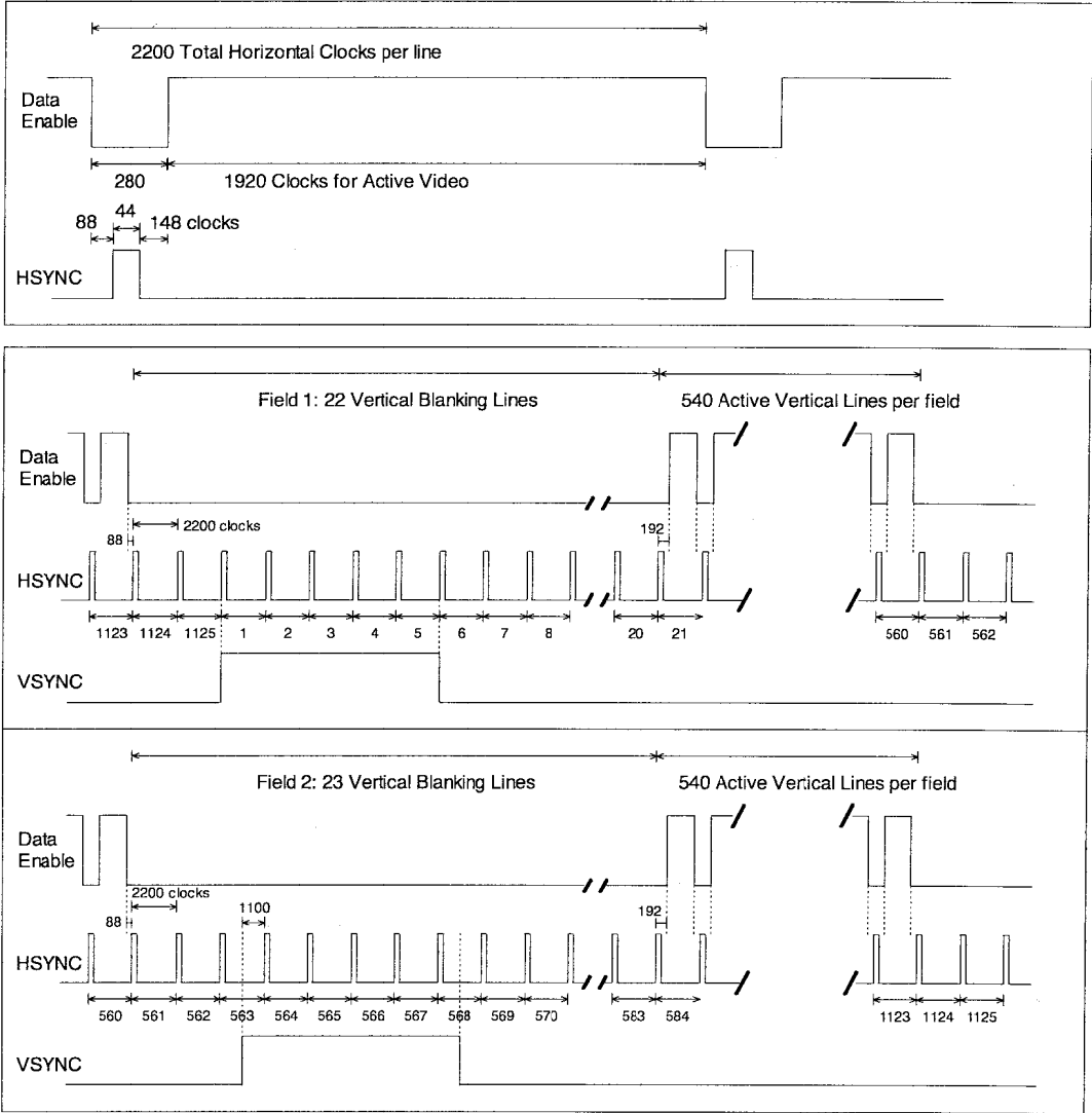
Figure 30 Timing Parameters for 1920x1080i @ 119.88/120 Hz
