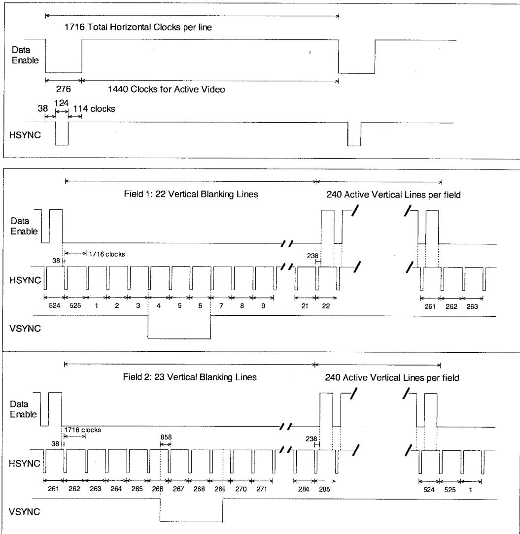
Figure 37 Timing Parameters for 720(1440)x480i @ 239.76/240 Hz
