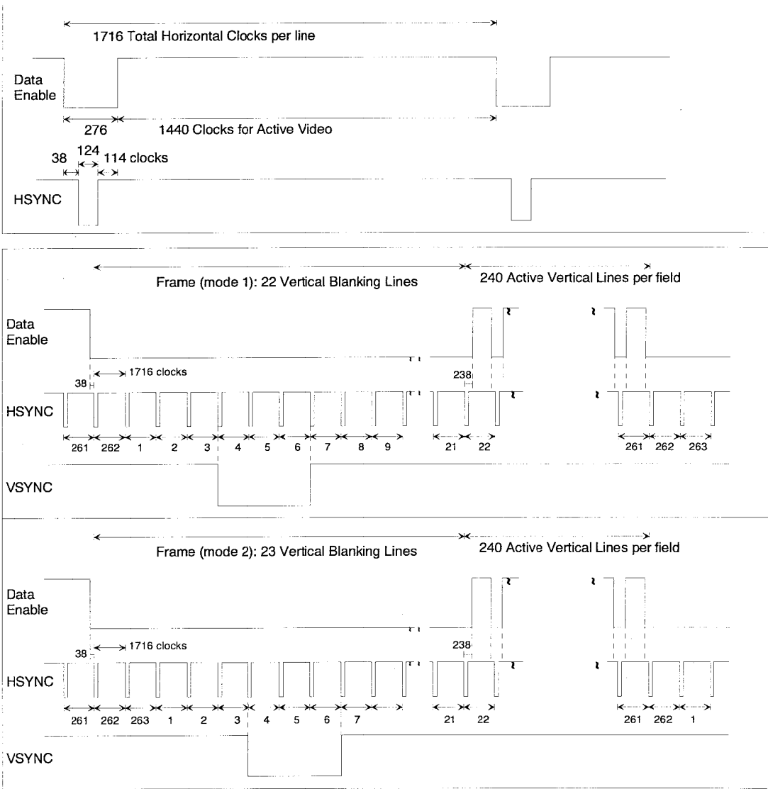
Figure 10 Timing Parameters for 720(1440)x240p @ 59.94/60 Hz
