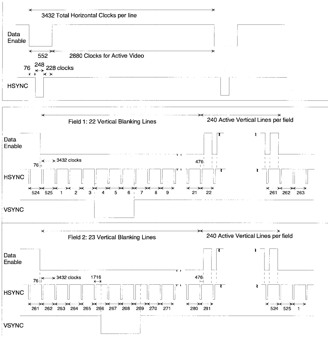
Figure 11 Timing Parameters for (2880)x480i @ 59.94/60 Hz
