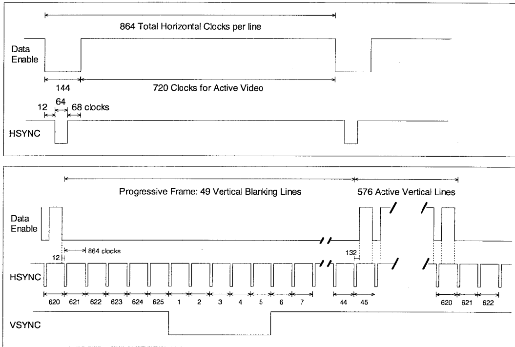
Figure 28 Timing Parameters for 720x576p @ 100 Hz
