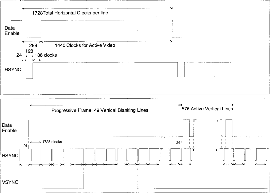
Figure 18 Timing Parameters for 1440x576p @ 50 Hz
