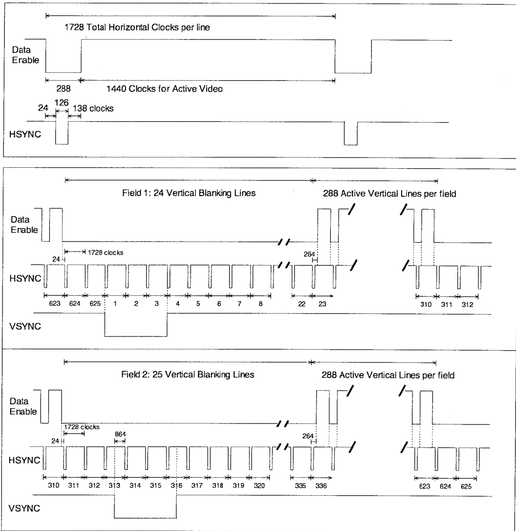
Figure 29 Timing Parameters for 720(1440)x576 @ 100 Hz
