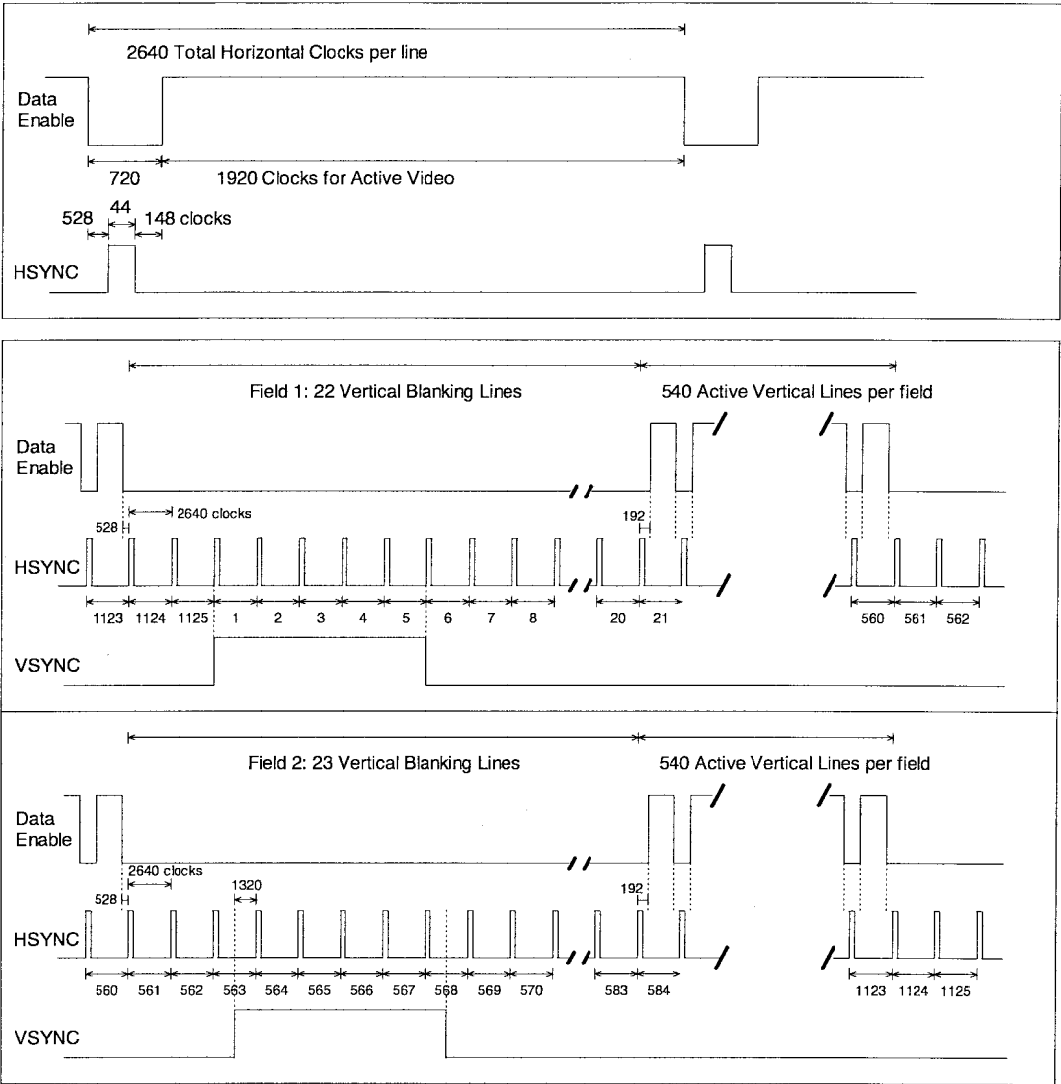
Figure 26 Timing Parameters for 1920x1080i @ 100 Hz
