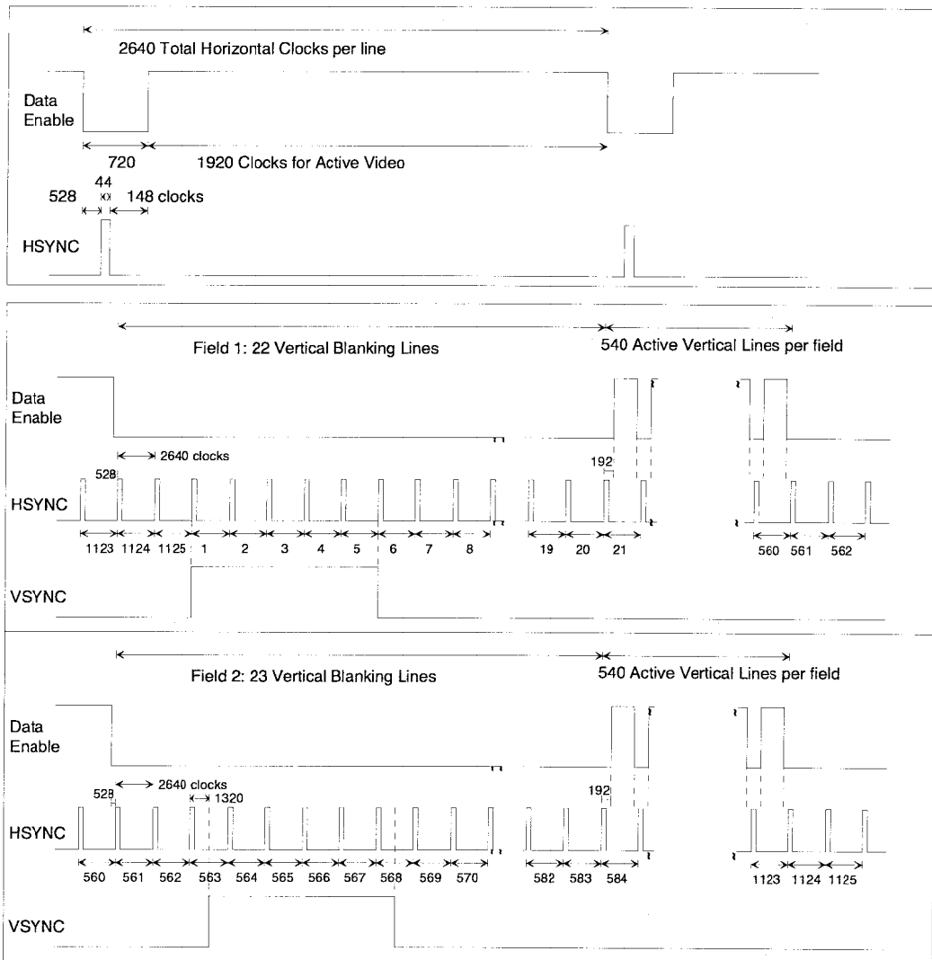
Figure 7 Timing Parameters for 1920x1080i @ 50 Hz
