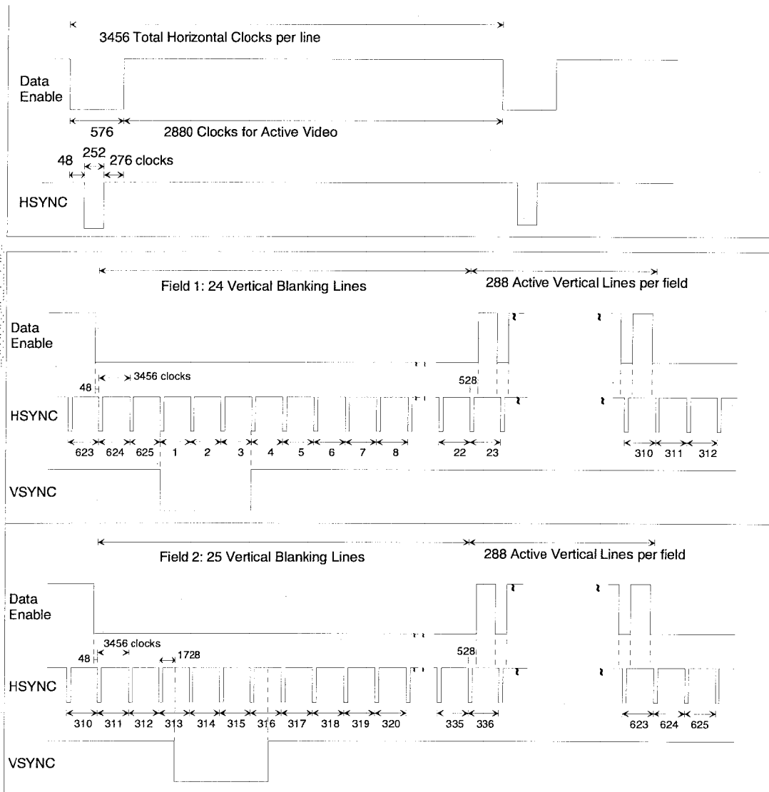
Figure 16 Timing Parameters for (2880)x576i @ 50 Hz
