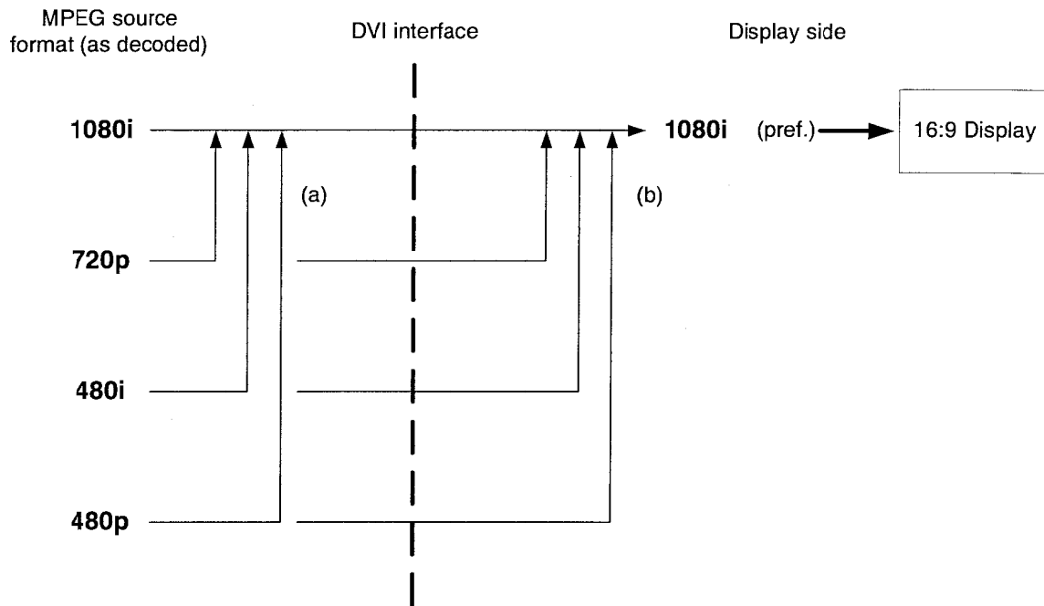
Figure 40 Example of Options for Format Conversion
