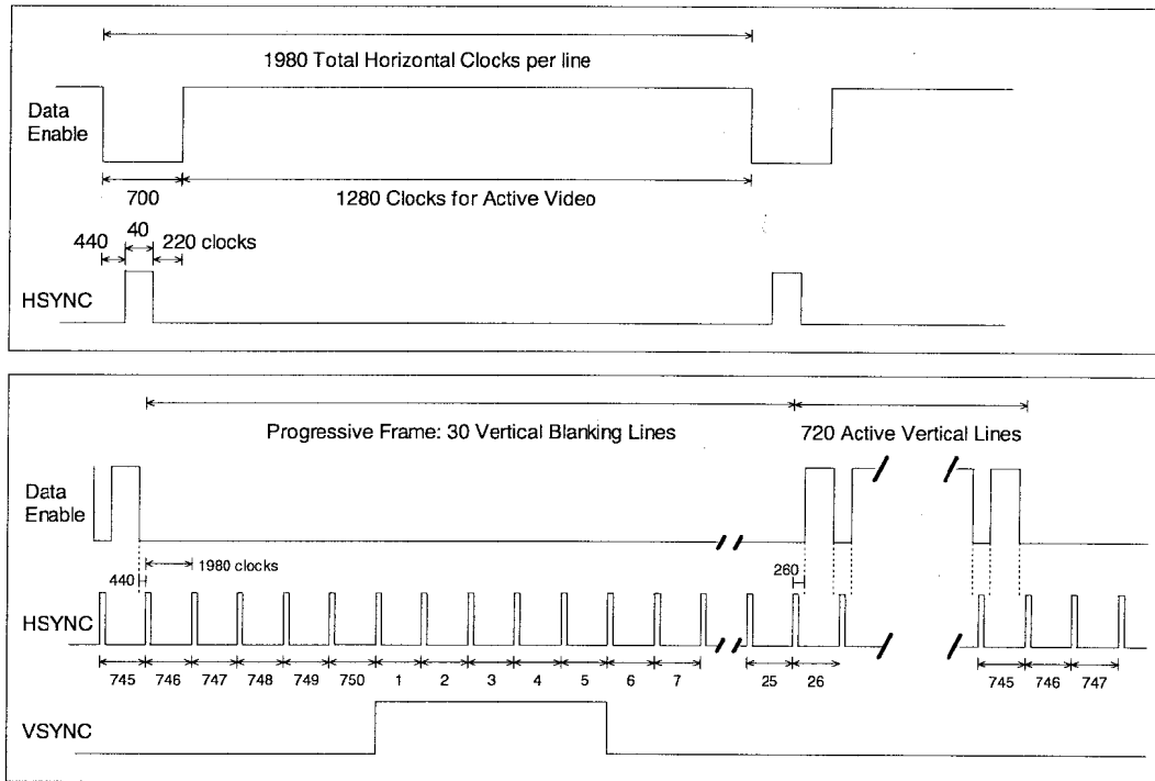
Figure 27 Timing Parameters for 1280x720p @ 100 Hz
