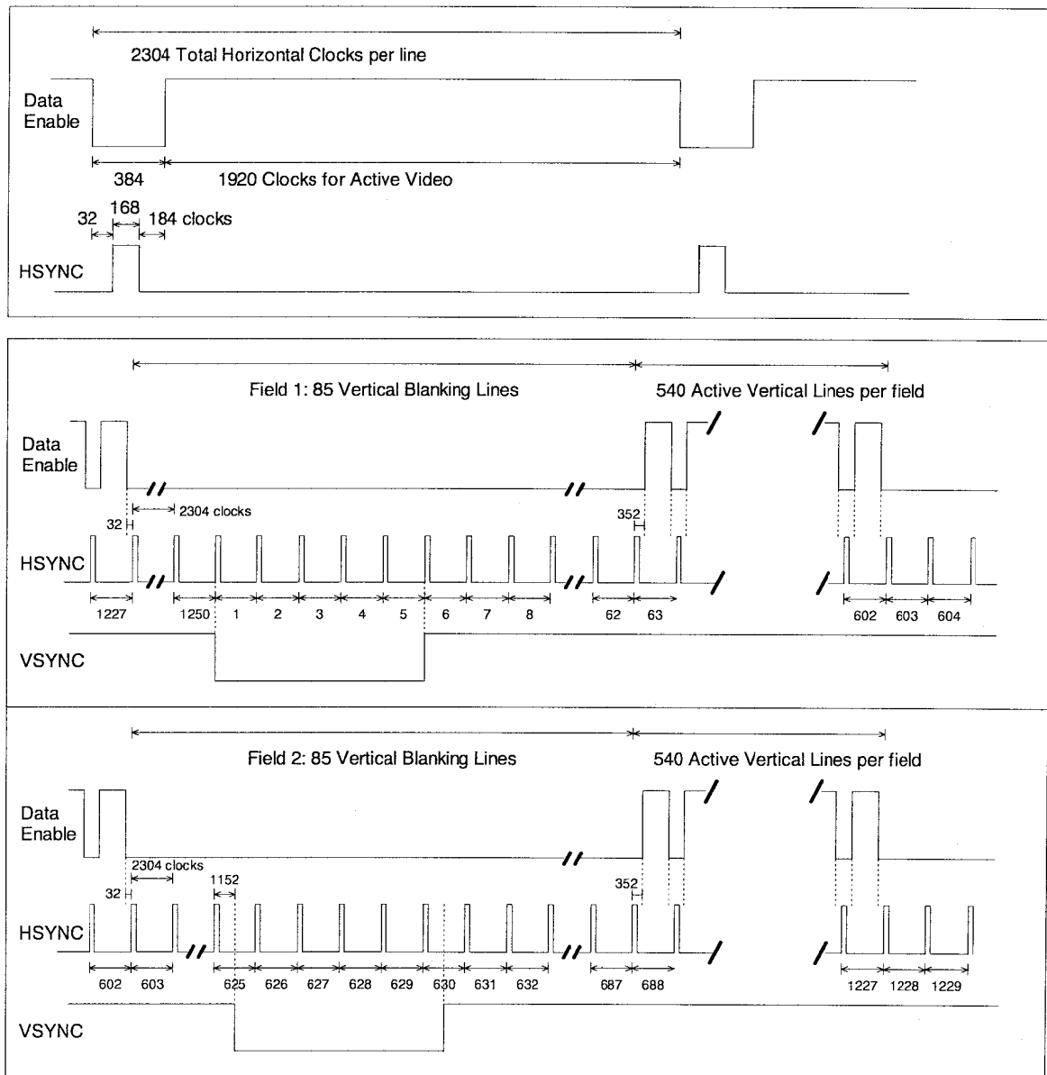
Figure 25 Timing Parameters for 1920x1080i (1250 Total) @ 50 Hz
