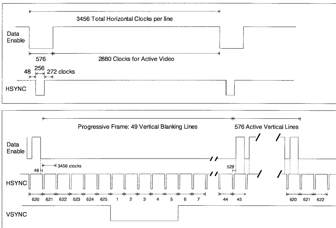
Figure 24 Timing Parameters for 2880x576p @ 50 Hz
