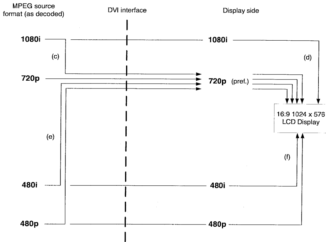
Figure 41 Multiple Conversions Example
