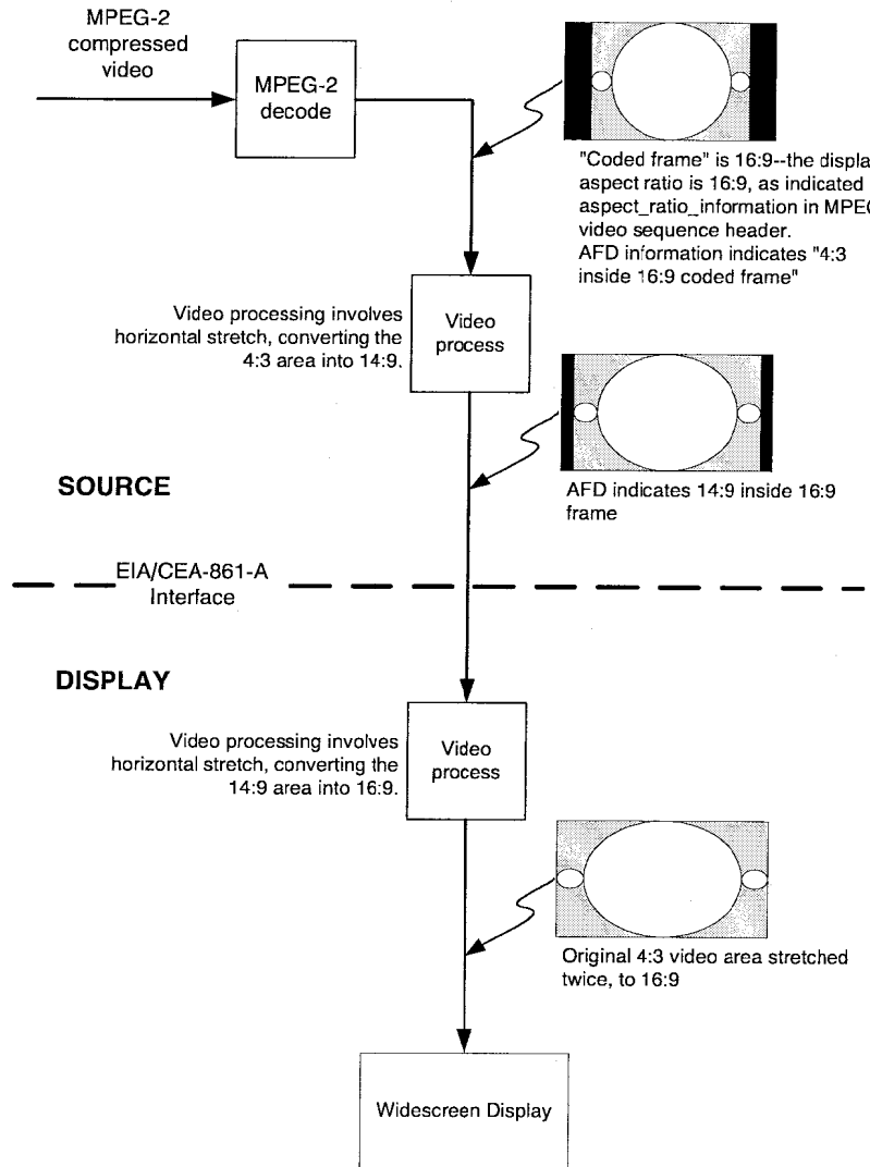
Figure 43 Example of Problem Resulting from Double Stretch
