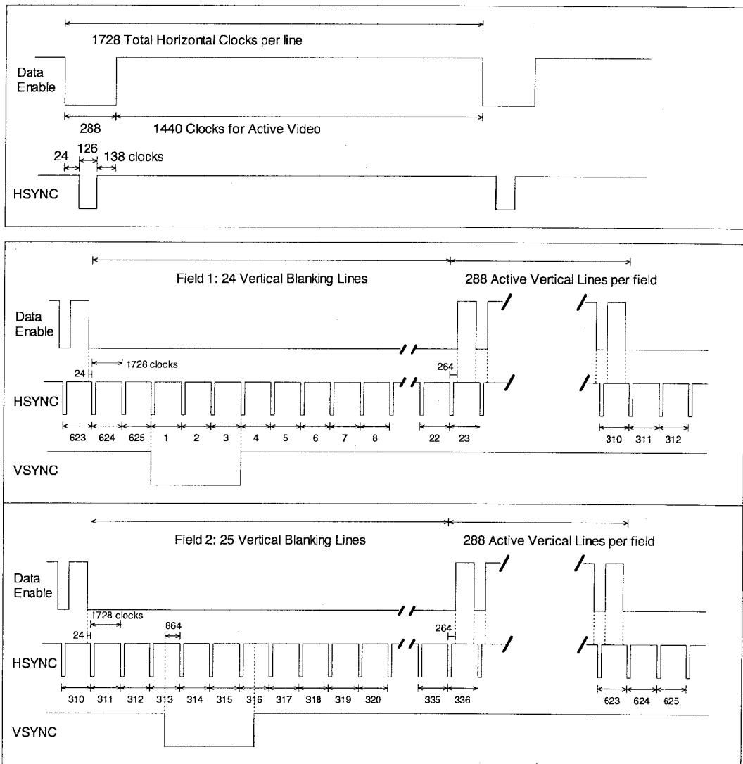
Figure 35 Timing Parameters for 720(1440)x576i @ 200 Hz
