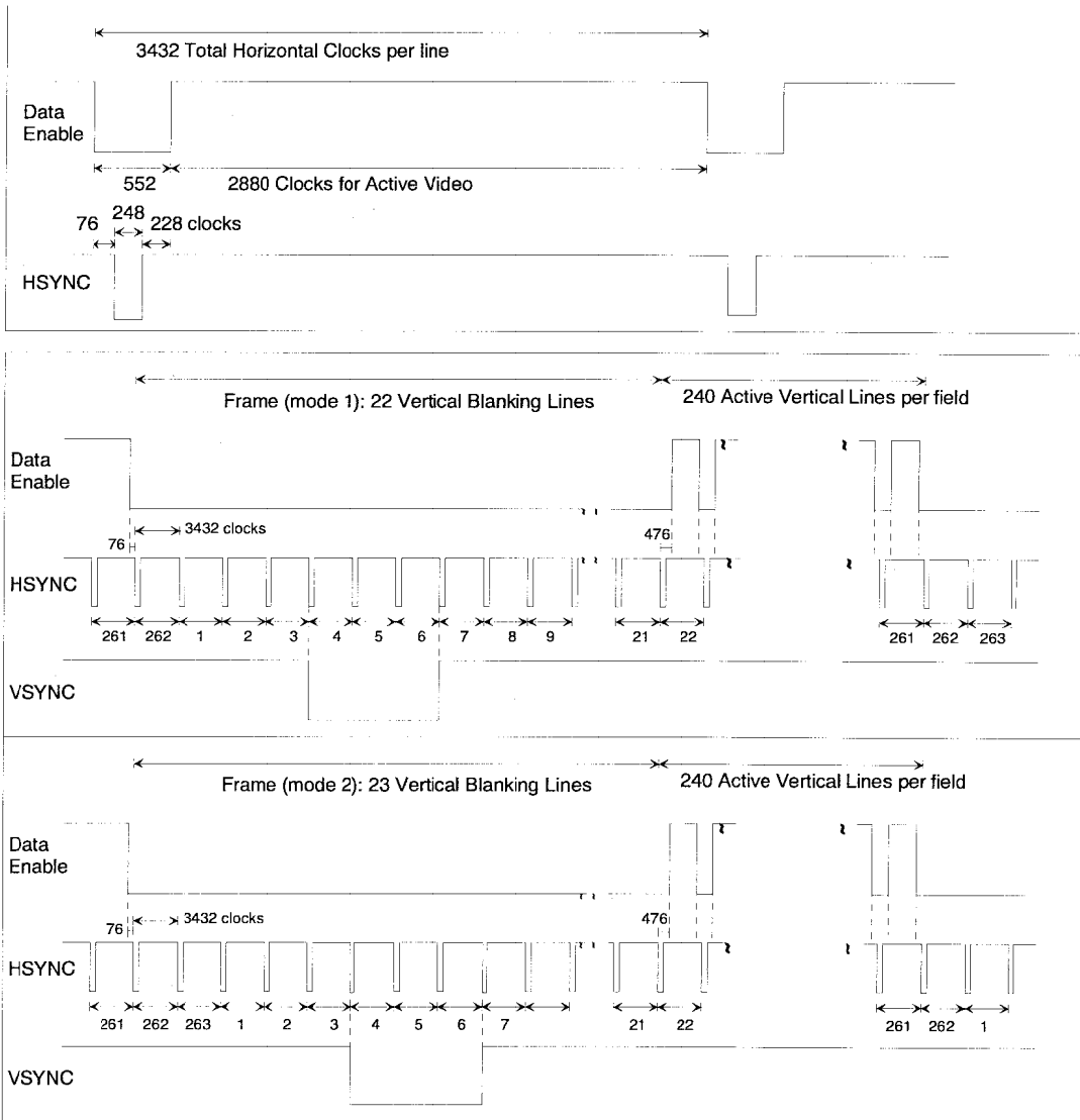
Figure 12 Timing Parameters for (2880)x240p @ 59.94/60 Hz
