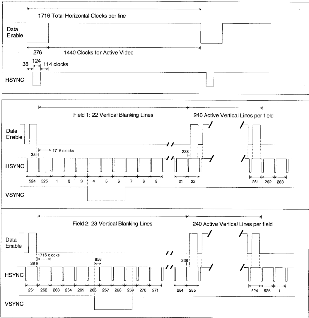
Figure 33 Timing Parameters for 720(1440)x480i @ 119.88/120 Hz
