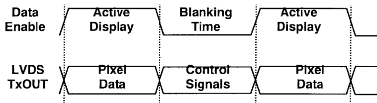
Figure 39 OpenLDI Synchronization
