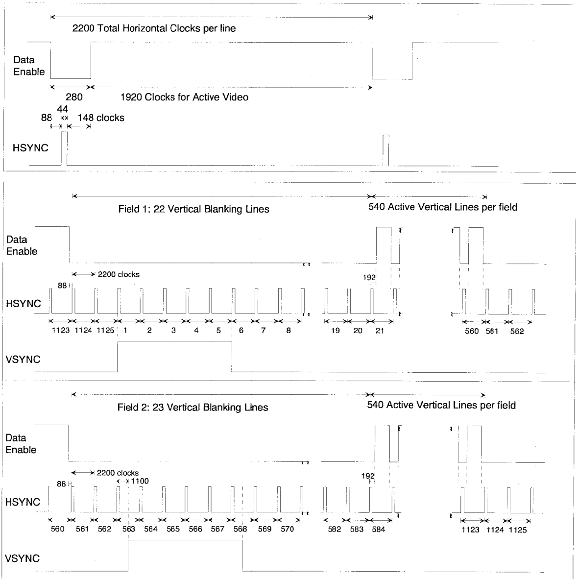
Figure 3 Timing Parameters for 1920x1080i @ 59.94/60 Hz
