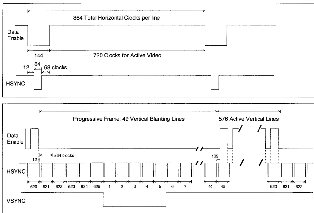
Figure 34 Timing Parameters for 720x576p @ 200 Hz
