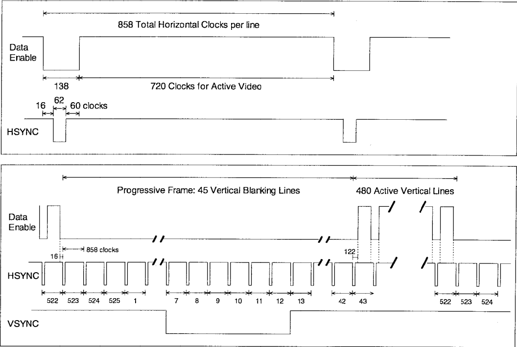
Figure 32 Timing Parameters for 720x480p @ 119.88/120 Hz
