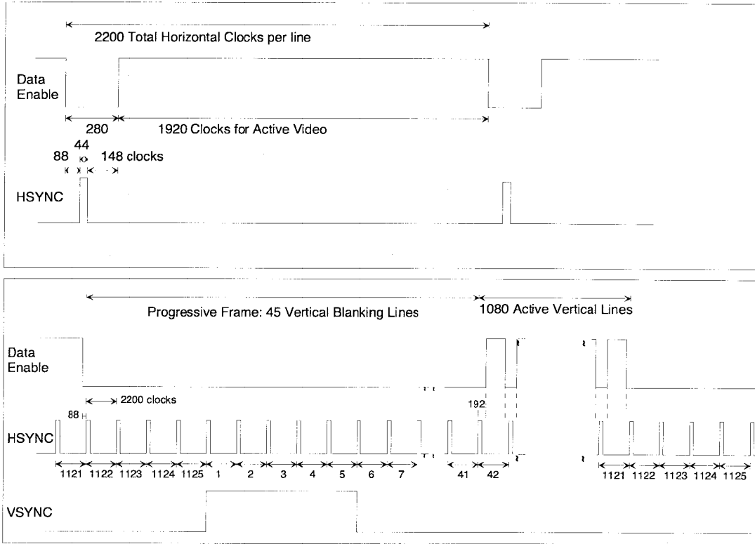
Figure 14 Timing Parameters for 1920x1080p @ 59.94/60 Hz
