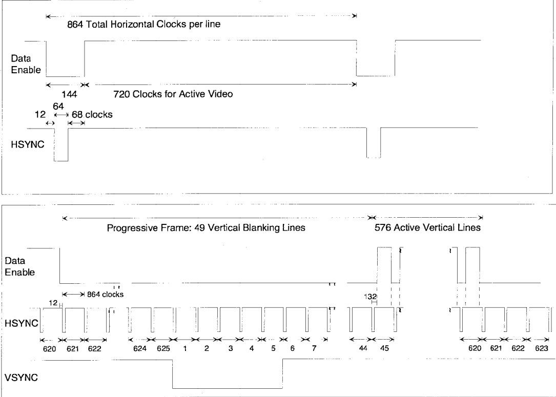
Figure 8 Timing Parameters for 720x576p @ 50 Hz
