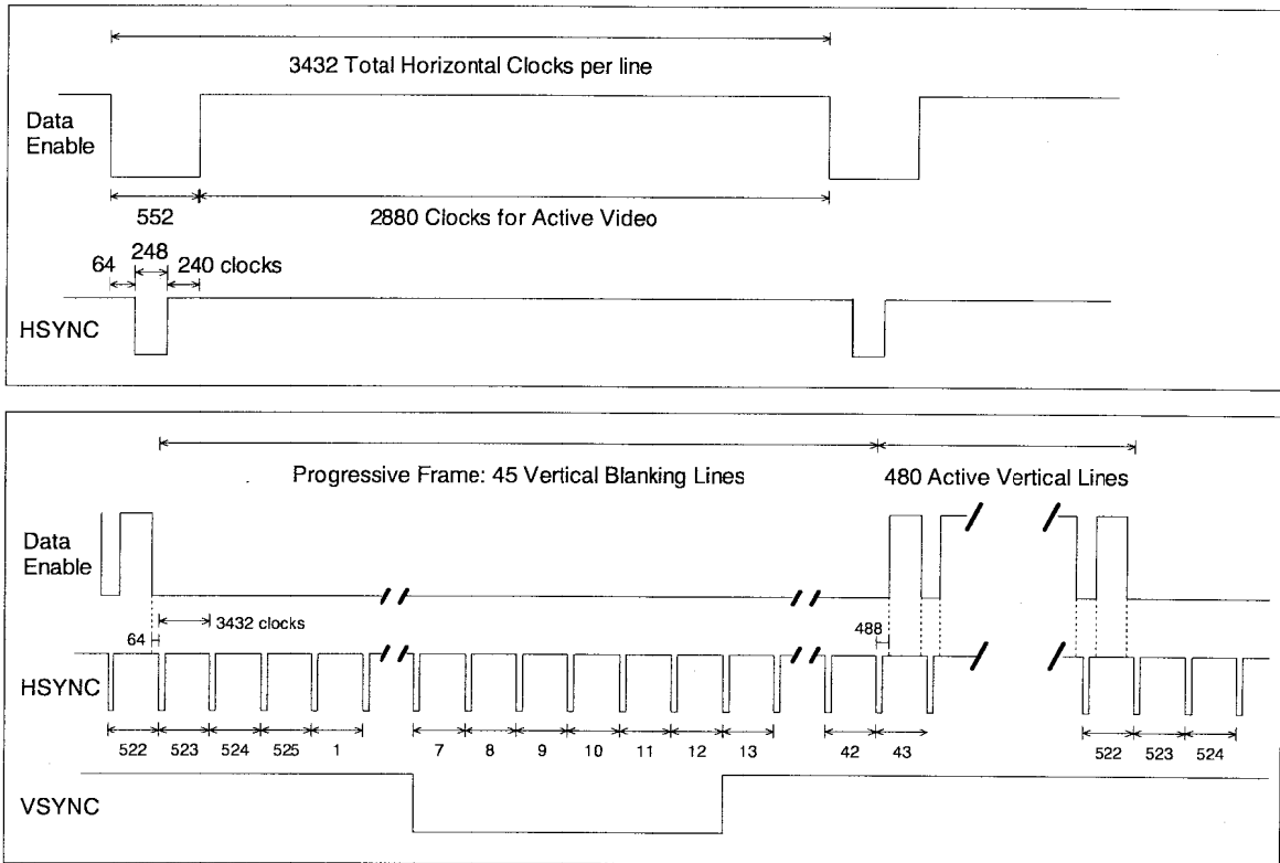
Figure 23 Timing Parameters for 2880x480p @ 59.94/60 Hz
