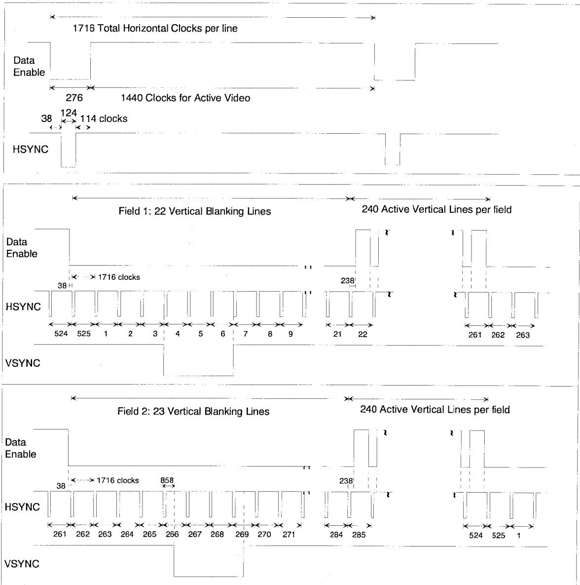
Figure 5 Timing Parameters for 720(1440)x480i @ 59.94/60 Hz
