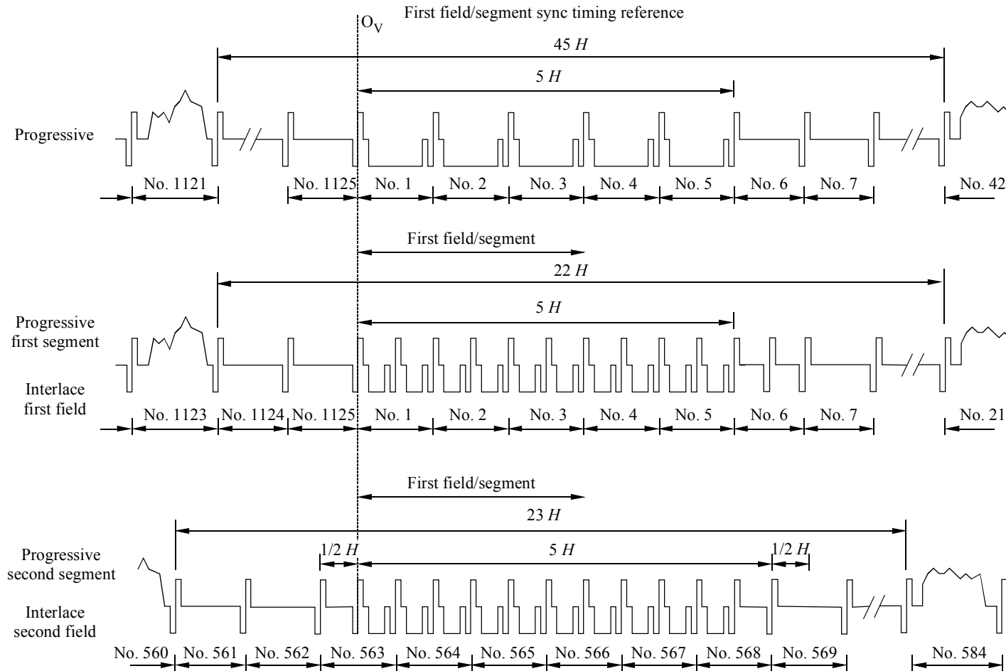
FIGURE 12A Field/frame/segment synchronizing signal waveform
