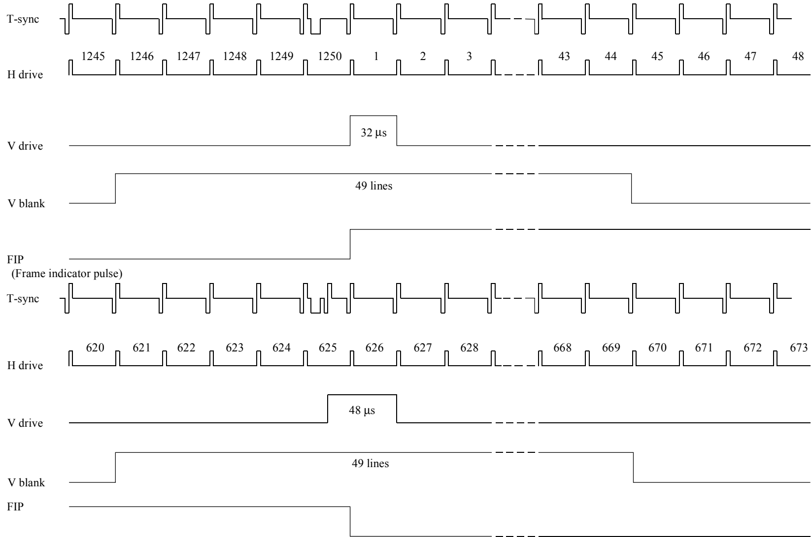
Timing of signals during the field-blanking interval for the 1250/50/2:1 system
