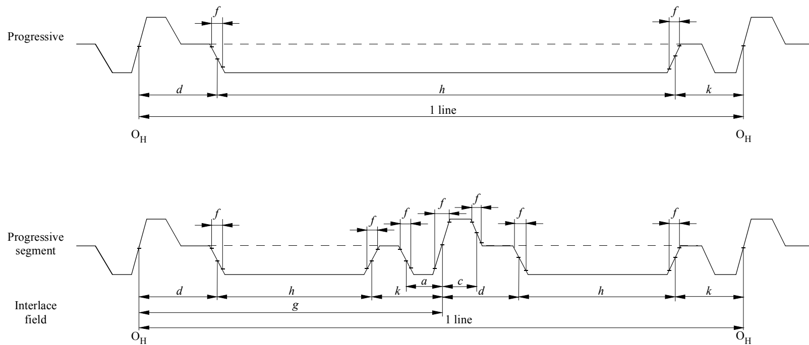
FIGURE 12B Detail of field/frame/segment synchronizing signal waveform
