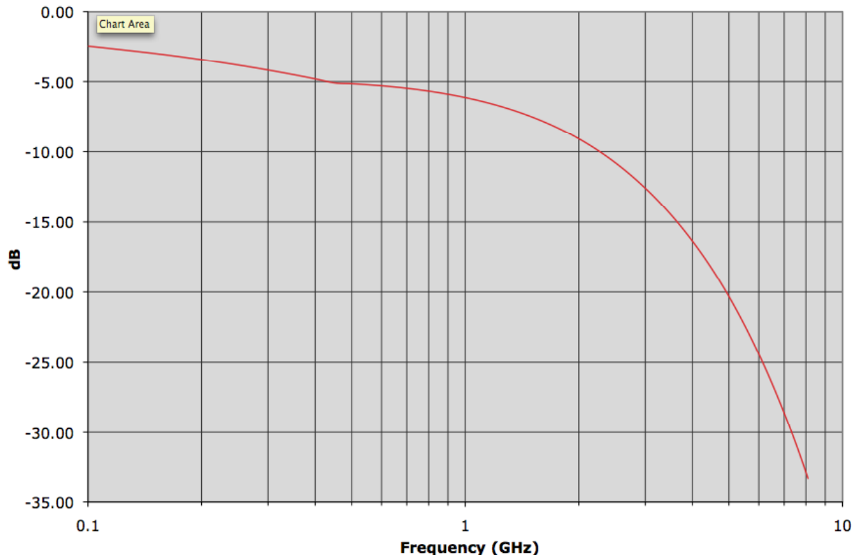
Figure 4-10: Mixed Mode Differential Insertion Loss for HBR Cable Assembly Type C1, C2 and C3
