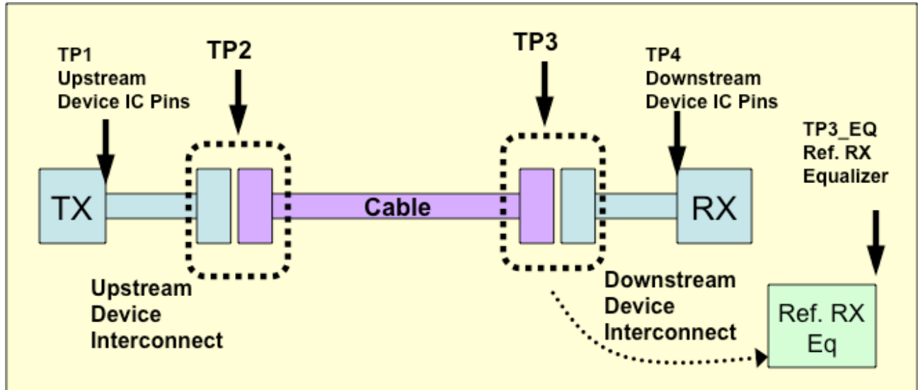
Figure 3-2: Compliance Measurement Points of the Channel
