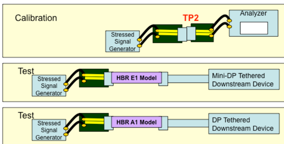
Figure 3-8: HBR Tethered Downstream Device Compliance Test Configuration
