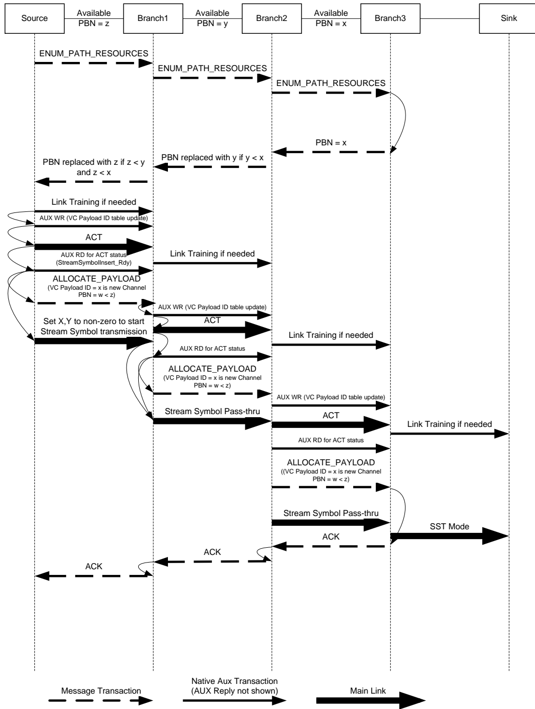
Figure 2-79: Example Time Sequence for Adding a New Payload
