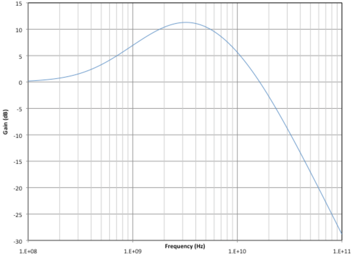
Figure 3-41: Reference HBR2 Receiver Equalizer Transfer Function
