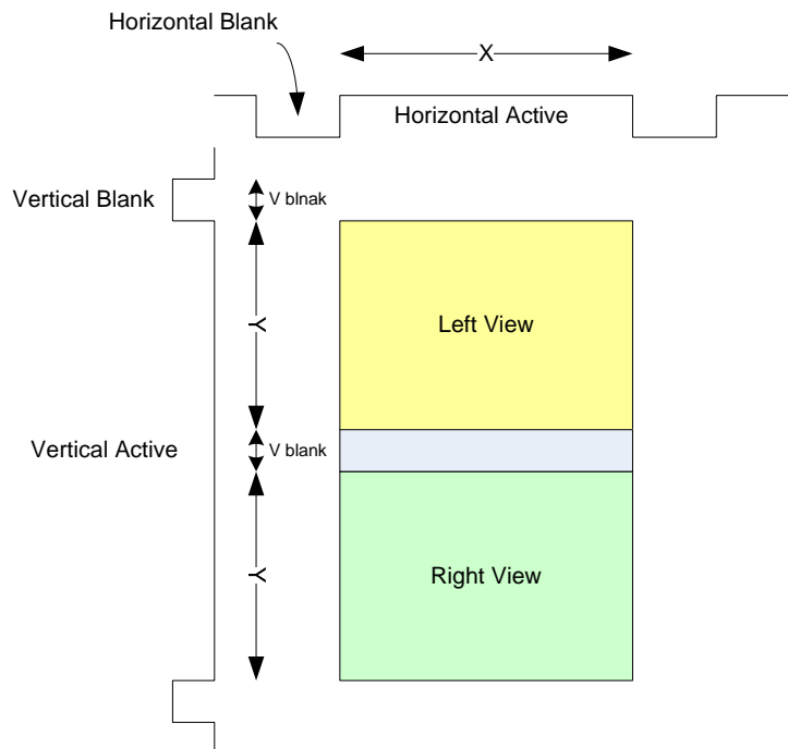
Figure 13-6: Stacked Top, Bottom Stereo Format with Left View on Top and Right View on Bottom
