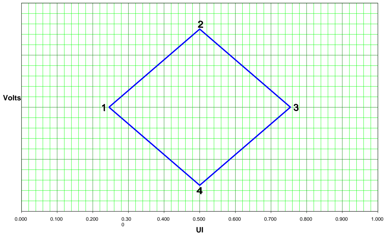
Figure 3-39: Downstream Device Mask at TP3 (RBR) or TP3_EQ (HBR)
