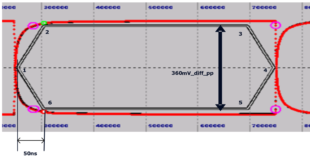
Figure 3-30: AUX CH EYE Mask for Manchester Transactions at Connector Pins of Receiving Device
