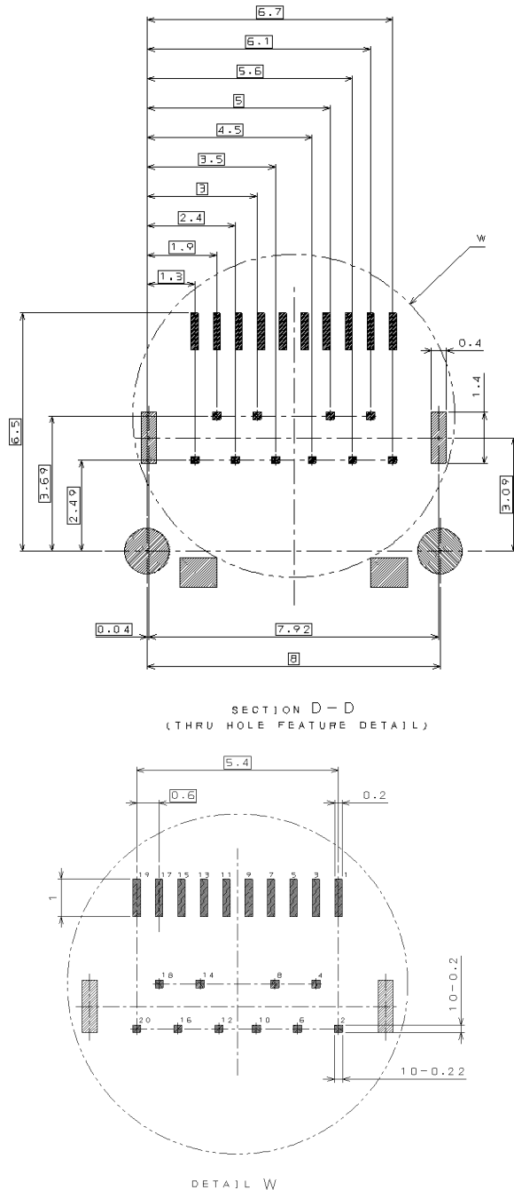
Figure 4-44: Recommended Mini DisplayPort Connector PCB Contacts and Mounting
