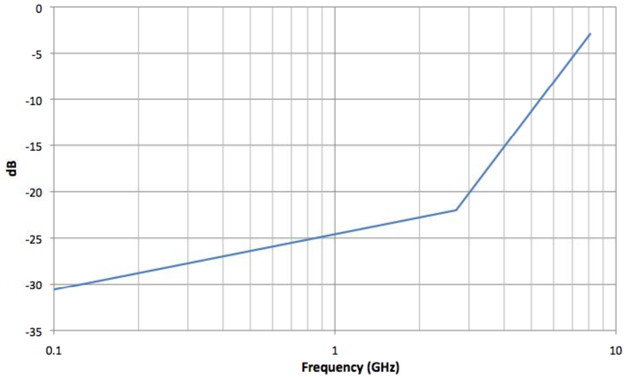
Figure 4-16: Power Sum Equal Level Far-End Total Noise (peak) for High Bit Rate Cable Assembly
