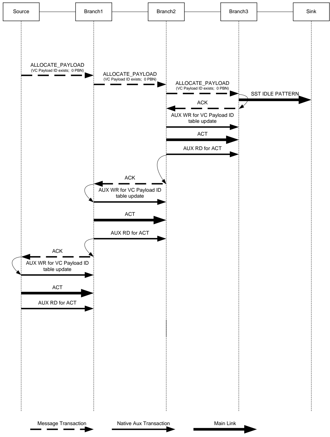
Figure 2-81: Timing Sequence for Deleting a Payload
