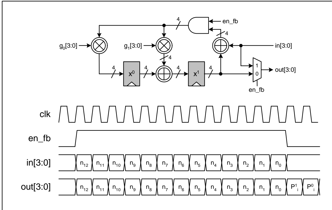
Figure 2-36: Block Diagram of a RS (15:13) Encoder
