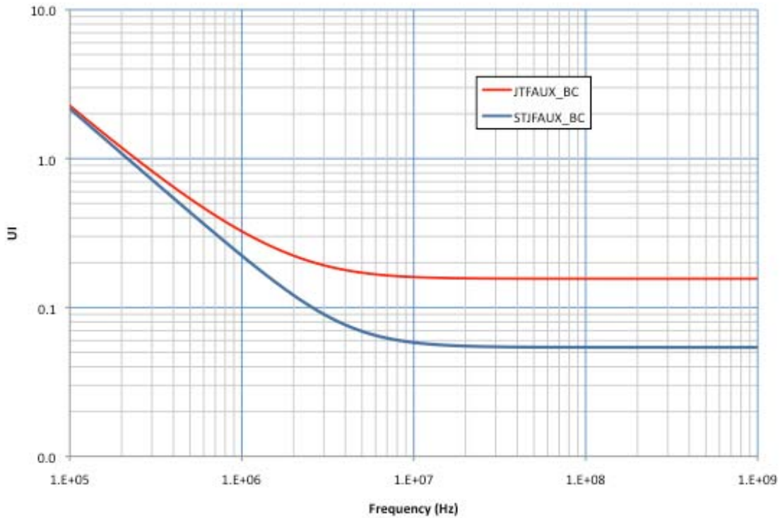
Figure 3-28: FAUX Back Channel Receiver Jitter Output/Input Tolerance Mask
