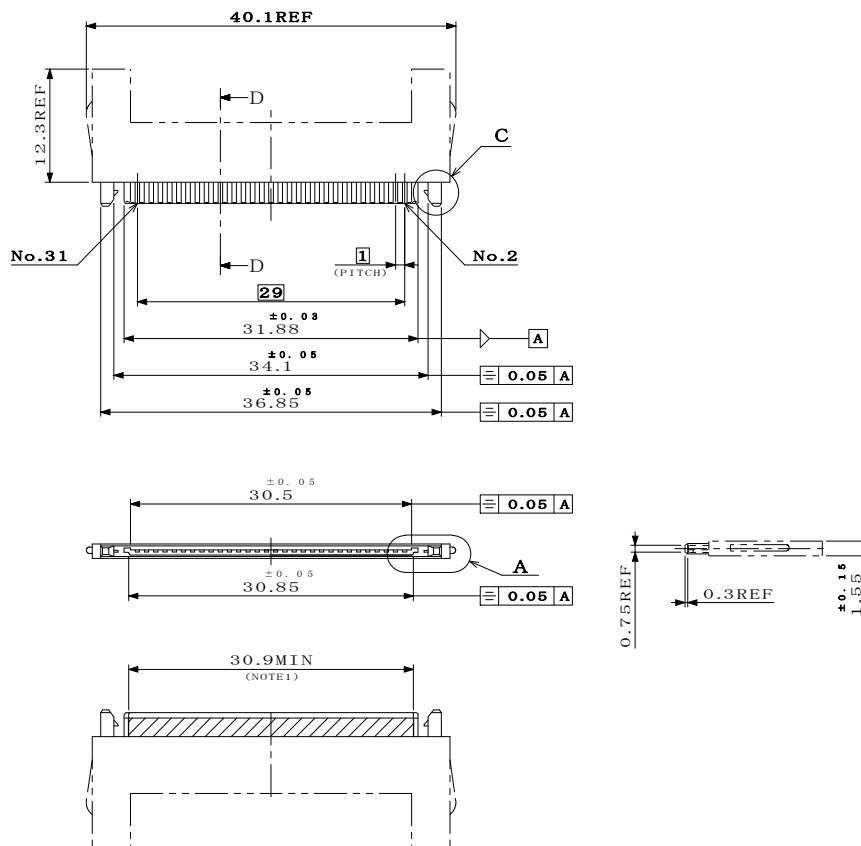
Figure 4-50: Panel-side Internal Cable Plug Connector (in unit of mm)
