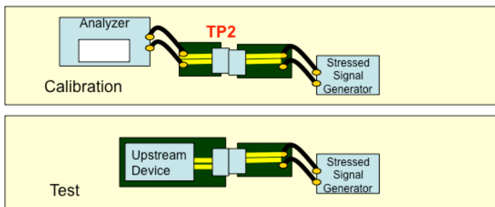
Figure 3-16: FAUX Back Channel Receiver Compliance Test Configuration
