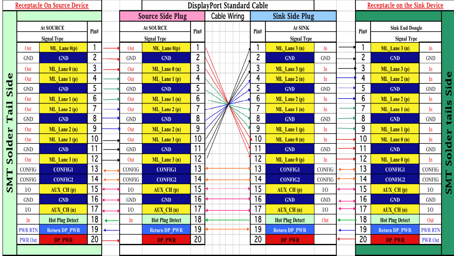
Figure 4-23: External Cable Connector Assembly Wiring
