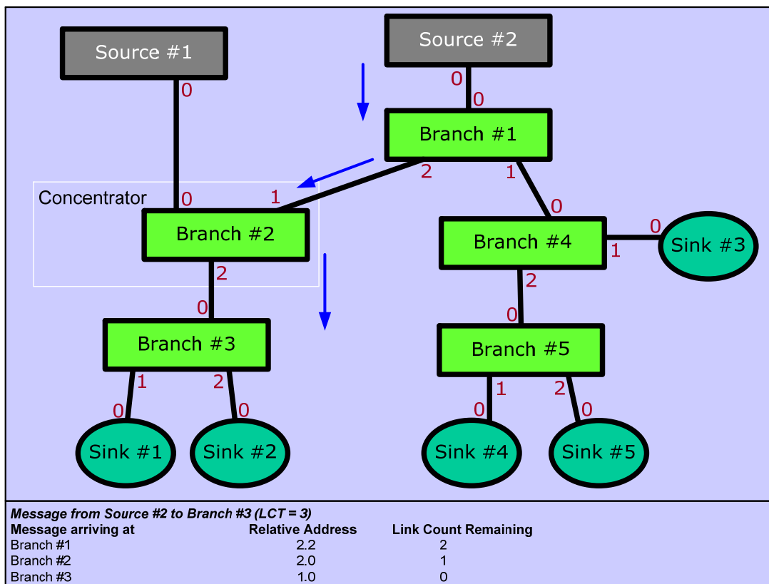
Figure 2-95: RAD Update Along the Path Using Example Topology
