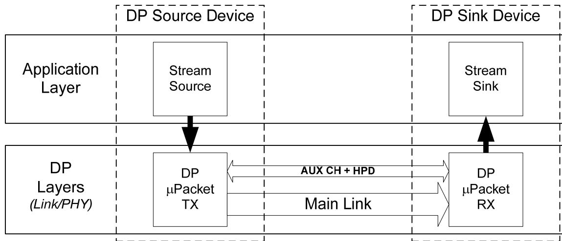
Figure 2-45: DisplayPort Data Transport Channels
