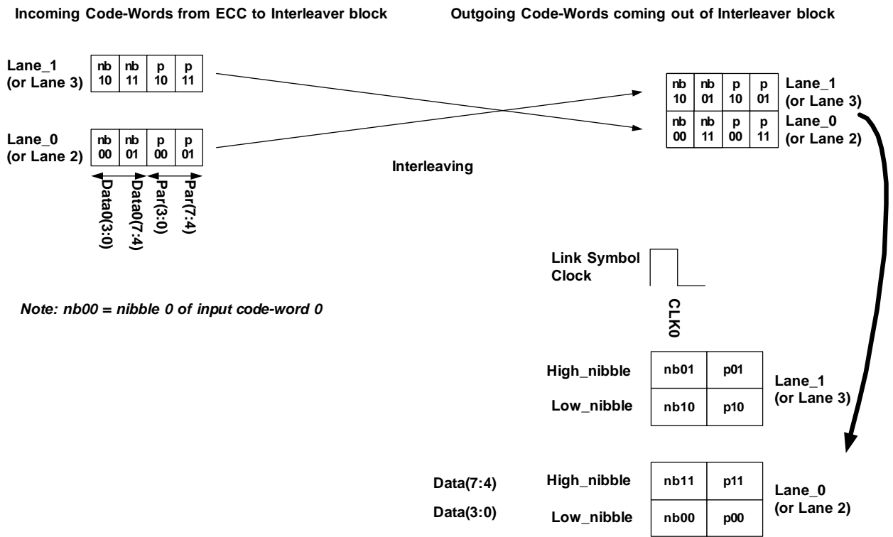
Figure 2-39: ECC Block Nibble-Interleaving for 2- and 4-Lane Main Links (Header)
