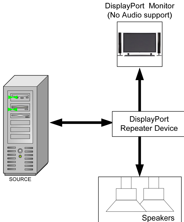
Figure 2-99: DisplayPort Monitor Connected Through a Repeater Device
