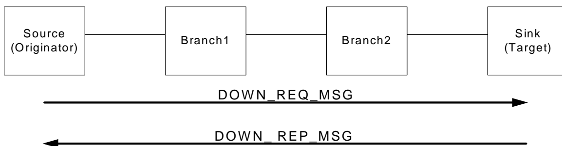
Figure 2-92: Down Request Message and Down Reply Message
