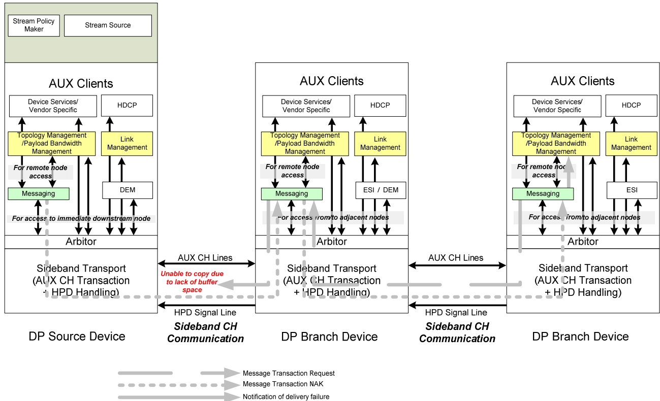
Figure 2-97: AUX CH Error While Delivering an Up Req Message
