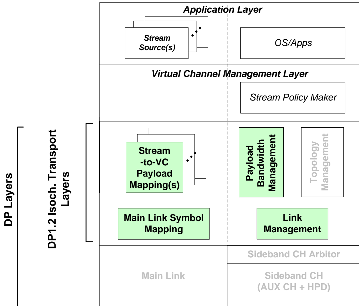
Figure 2-60: Layers Covered in this Section
