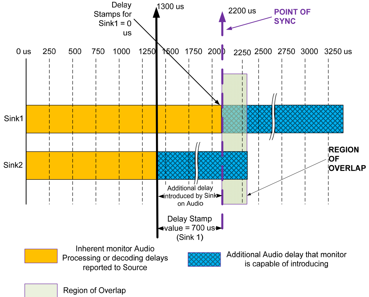
Figure 2-103: Delay Compensation for Audio-to-Audio Sync
