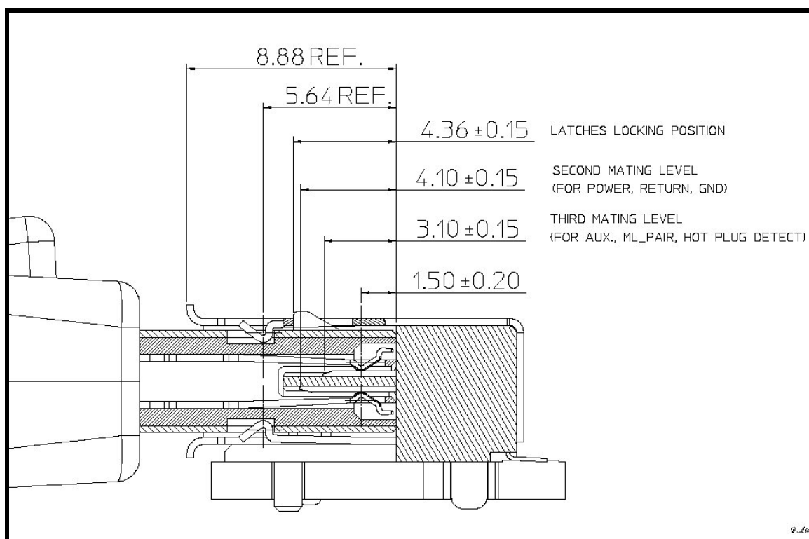
Figure 4-24: Connector Mating Levels
