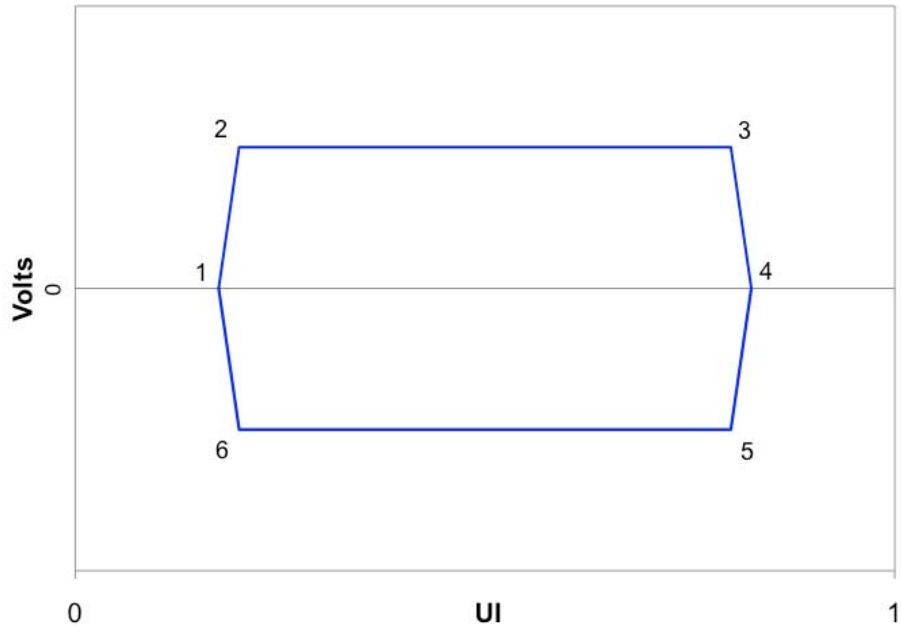
Figure 3-31: EYE Mask for FAUX Transactions
