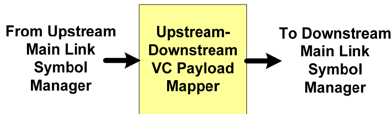
Figure 2-74: Pass-through DP Branch Device VC Payload Mapping Logical Block Diagram
