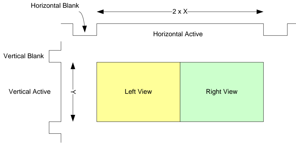
Figure 2-31: Interleave Pattern Corresponding to a Checkerboard Pattern with Alternating Left and Right Image Pixels
