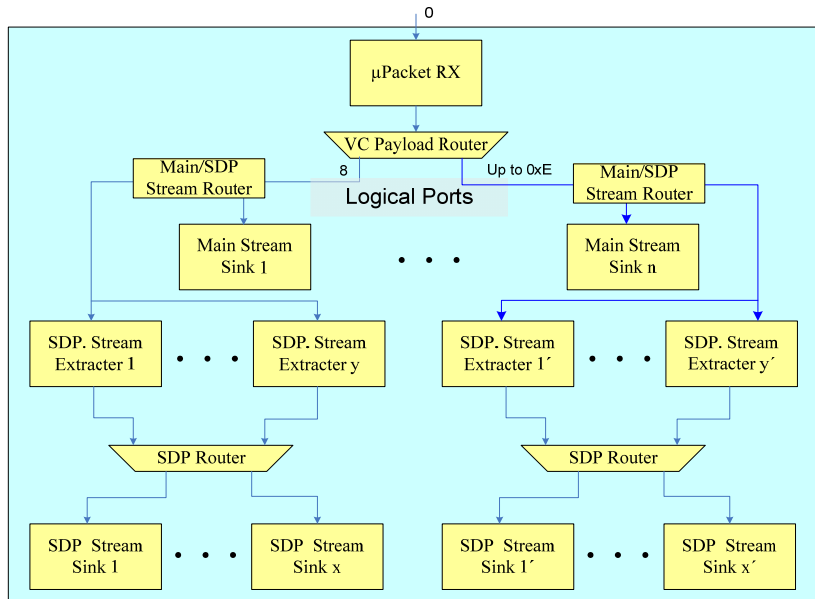
Figure 2-54: MST Multi-sink Device with Multiple Main Stream Sinks and SDP Sinks
