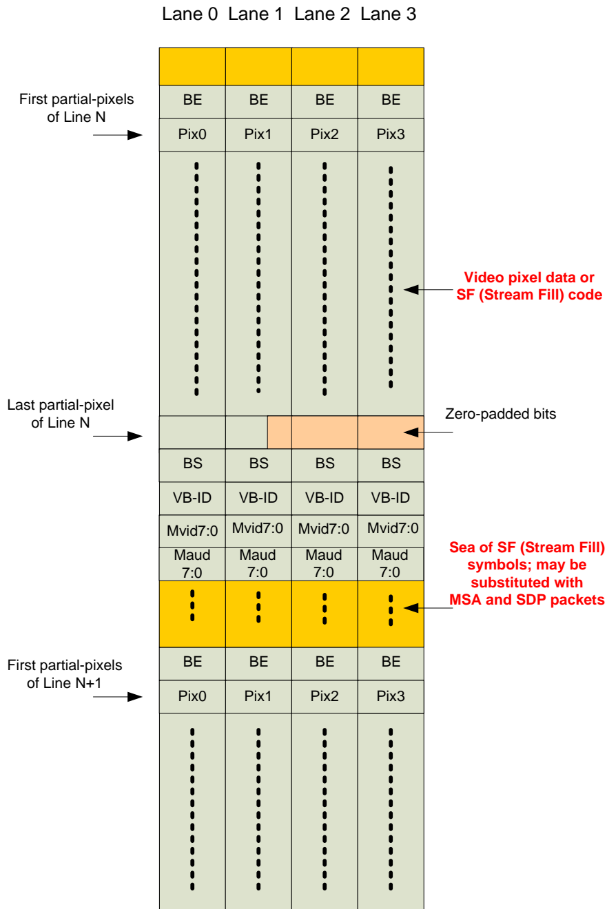
Figure 2-71: AV Stream Mapping in MST Mode After VC Payloads for a Given Main Video Stream are Concatenated and VC Payload Fill (VCPF) Symbol Sequences Removed
