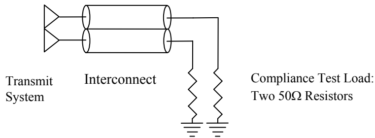
Figure 3-3: Compliance Test Load
