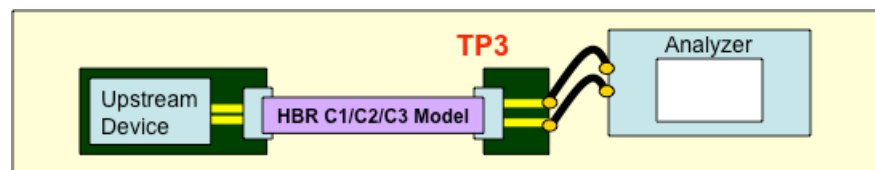
Figure 3-12: FAUX Forward Channel Transmitter Compliance Test Configuration
