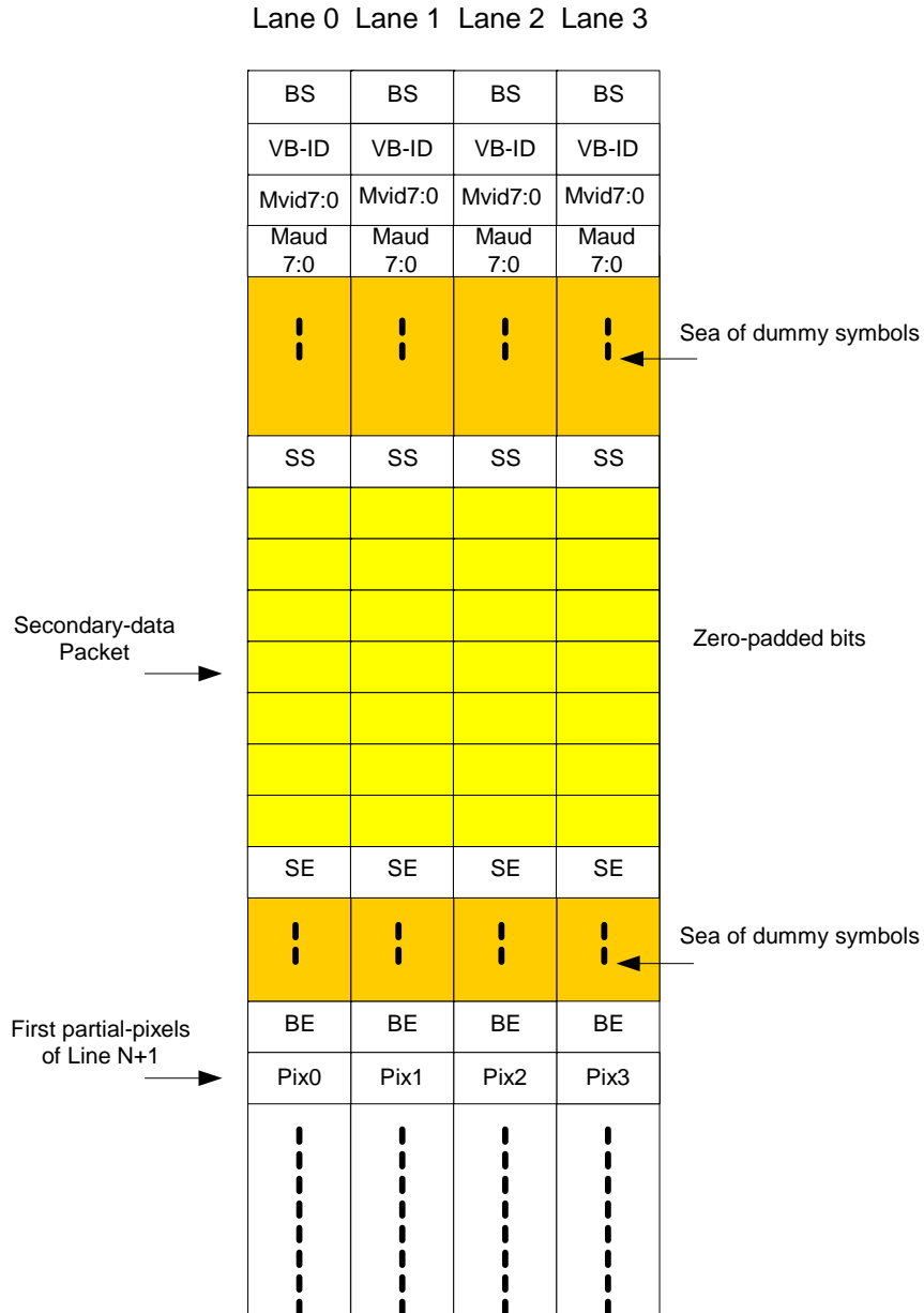
Figure 2-14: Secondary-Data Insertion
