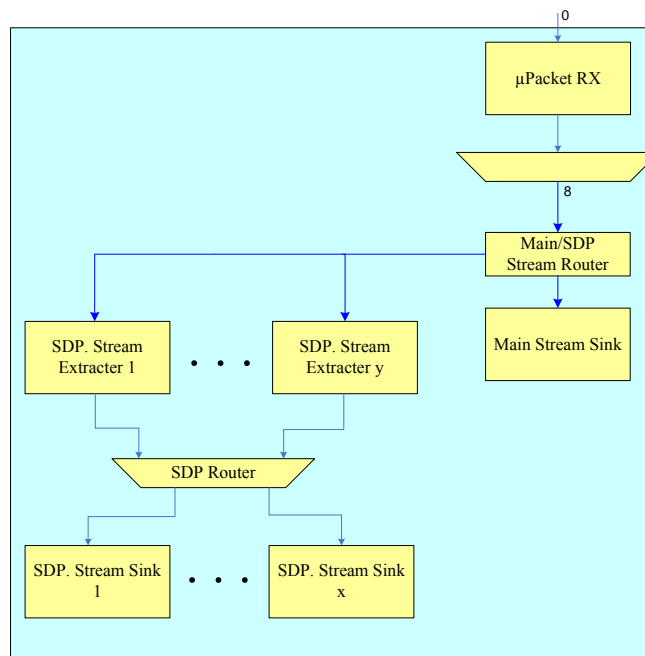
Figure 2-55: MST Sink Device with Single Main Stream Sink and Multiple SDP Sinks
