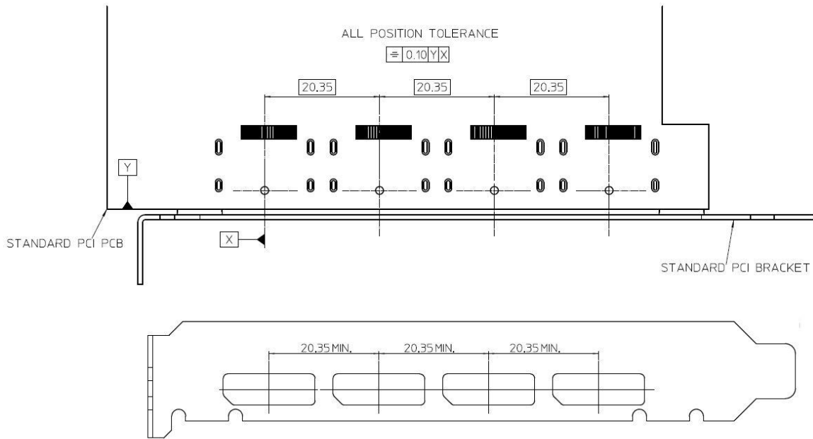
Figure 4-31: Reference Design for Four DisplayPort External Connectors on a PCI Card
