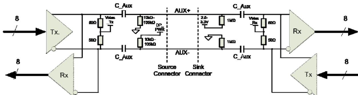
Figure 3-22: AUX CH Differential Pair
