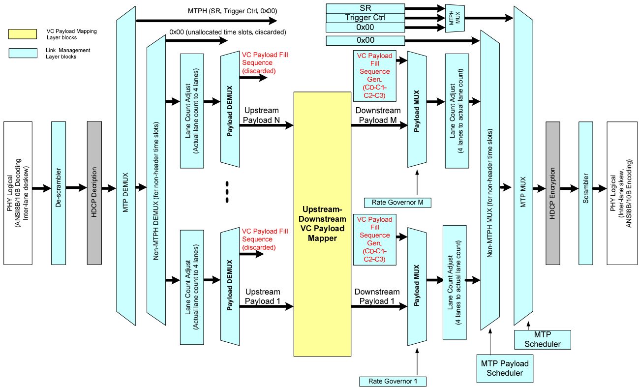
Figure 2-63: Logical Block Diagram of MST DP Branch Device
