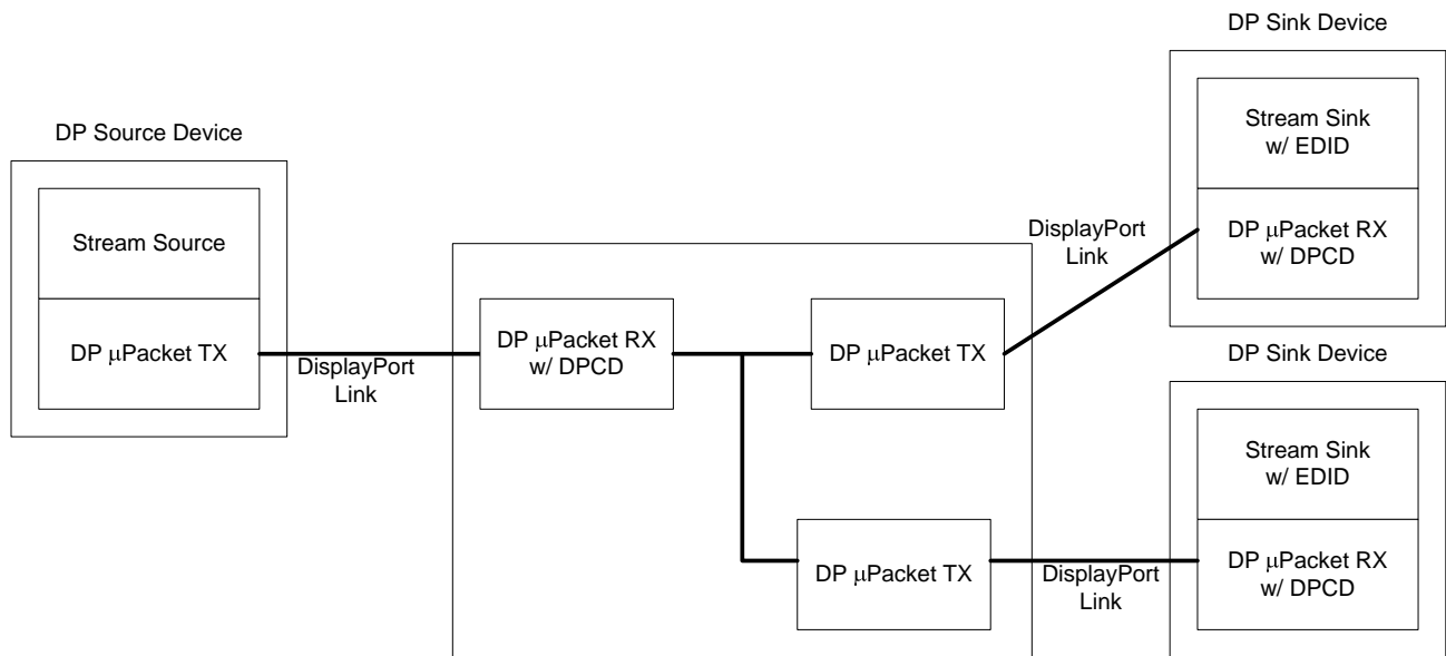
Figure 2-7: A DisplayPort Source Device to Multiple DisplayPort Sink Devices via a Replicator
