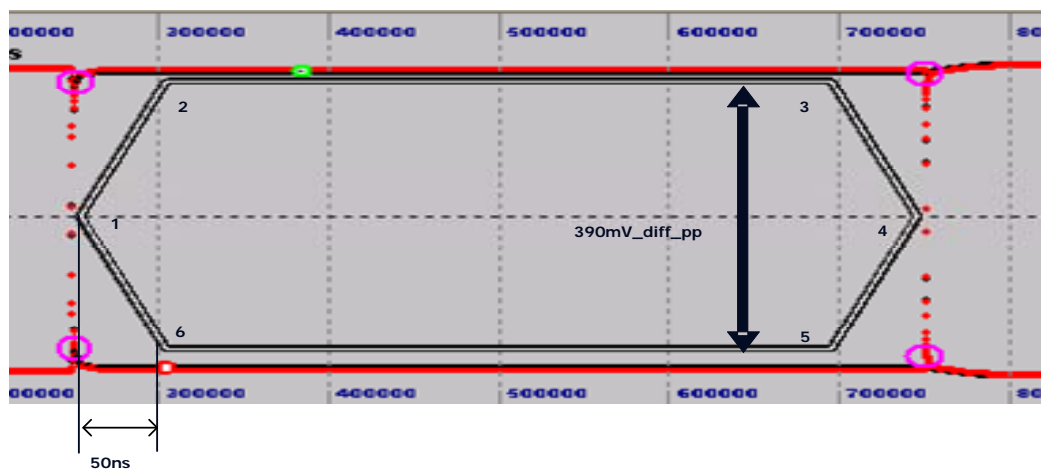
Figure 3-29: AUX CH EYE Mask for Manchester Transactions at Connector Pins of Transmitting Device
