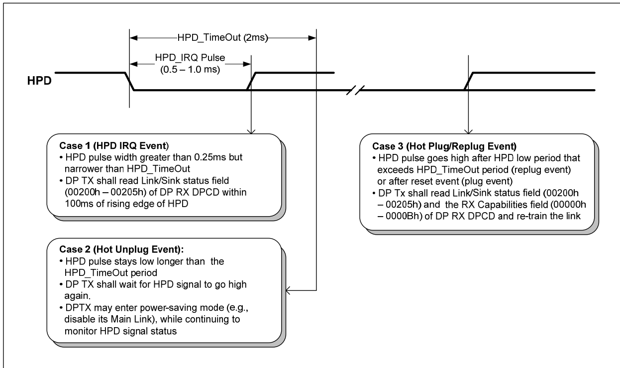
Figure 5-1: HPD Events
