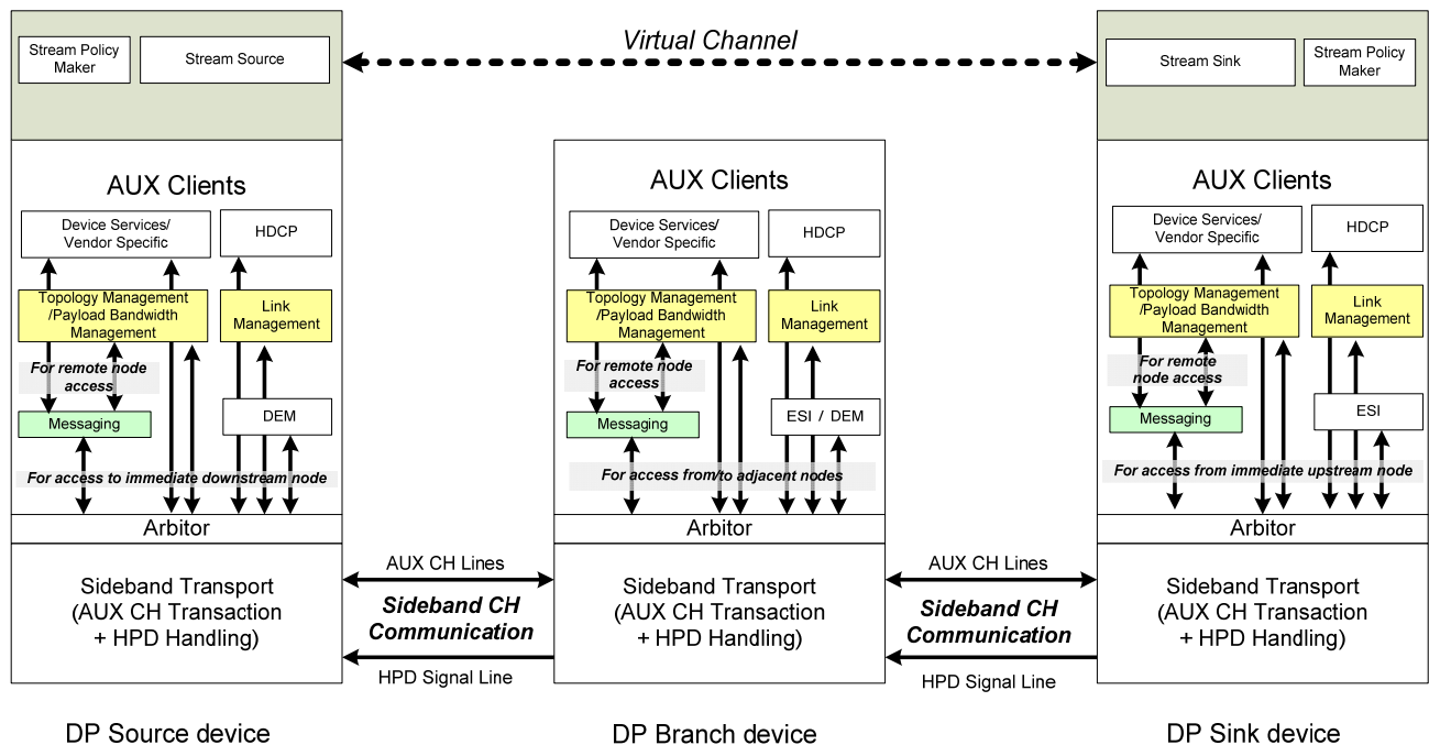
Figure 2-90: Messaging AUX Client in DP Nodes
