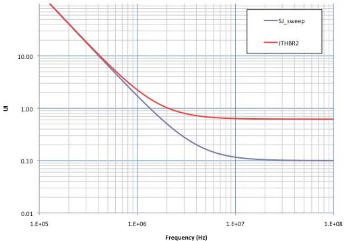
Figure 3-35: HBR2 Receiver Jitter Output/Input Tolerance Mask
