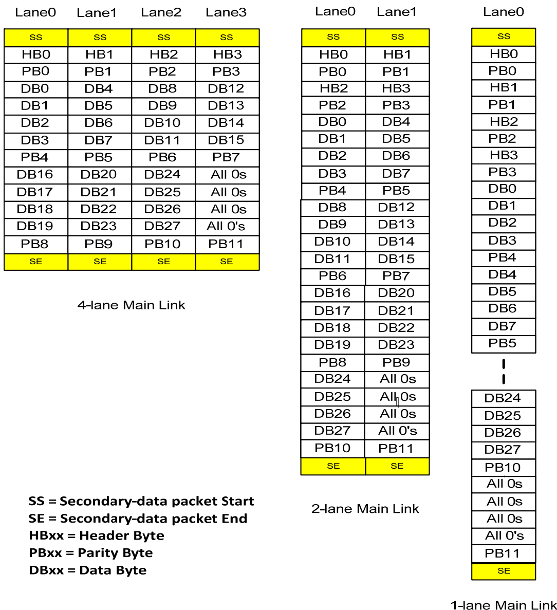
Figure 2-21: InfoFrame Packet
