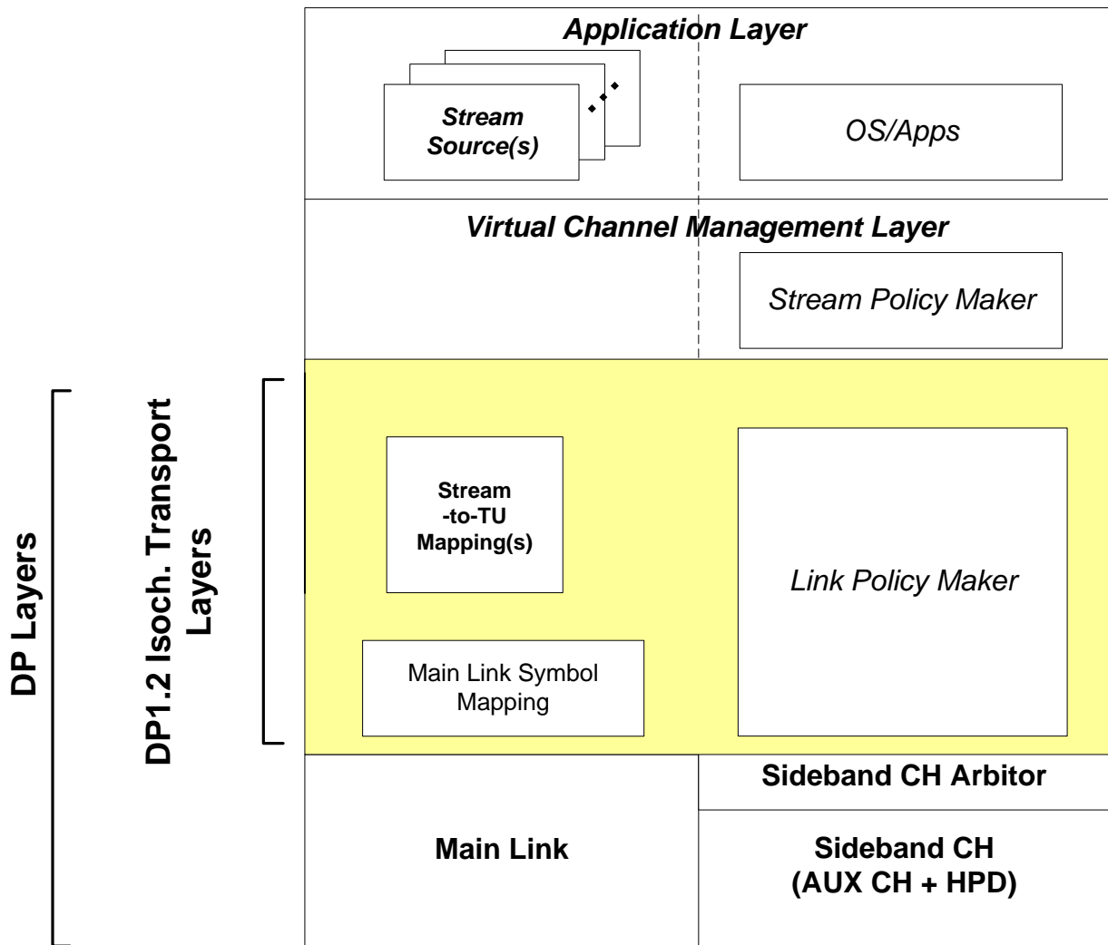
Figure 2-50: SST Isochronous Transport Service Layers
