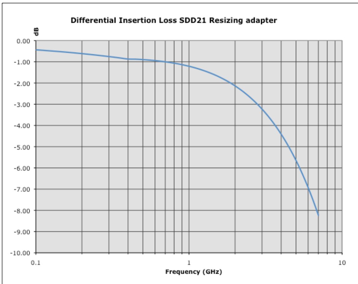
Figure 4-11: Mixed Mode Differential Insertion Loss for HBR Resizing Adaptor
