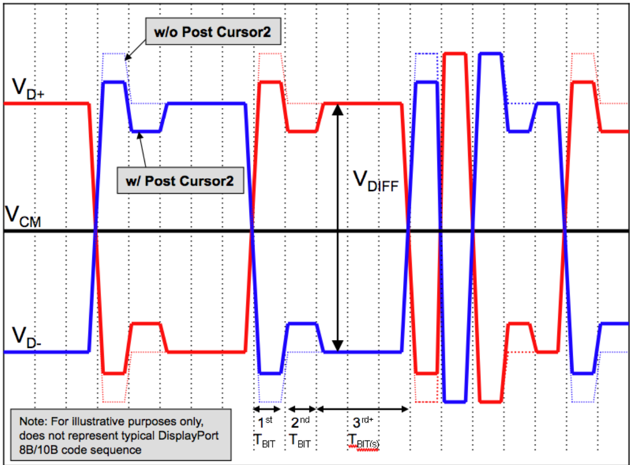
Figure 3-20: Example of Pre-emphasis with Post Cursor2
