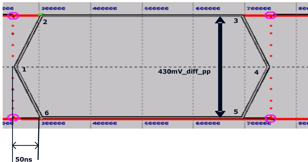
Figure 9-1: AUX CH EYE Mask at Transmitting IC Package Pins (Informative)
