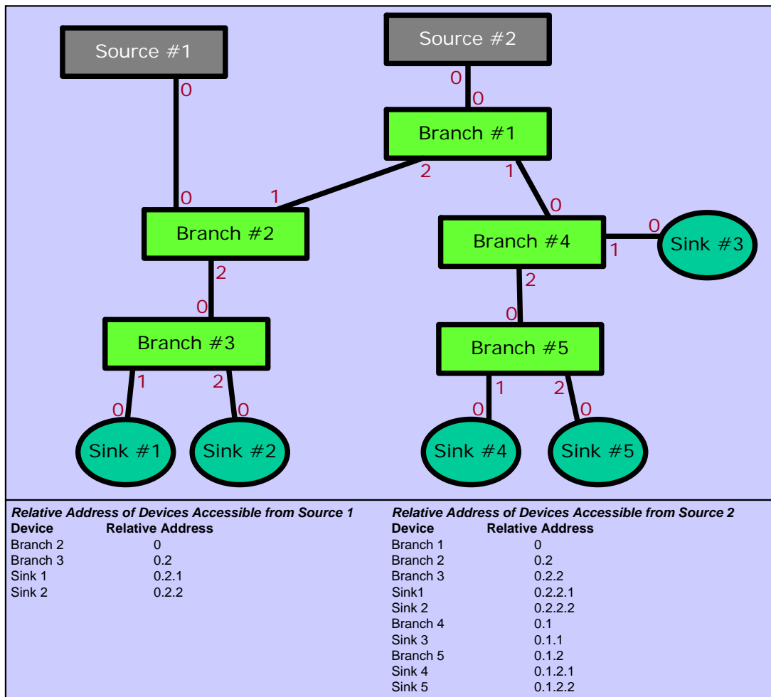
Figure 2-58: Example Topology with RAD of Devices Relative to Source Devices
