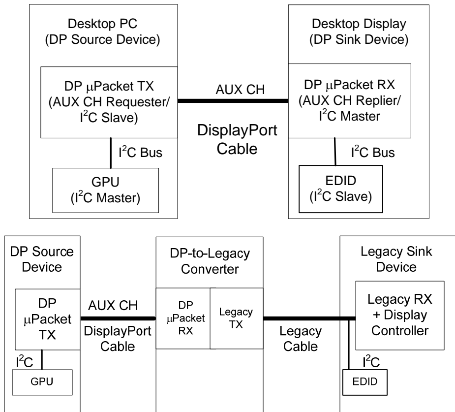
Figure 2-88: Examples of AUX CH Bridging Two I 2 C Buses
