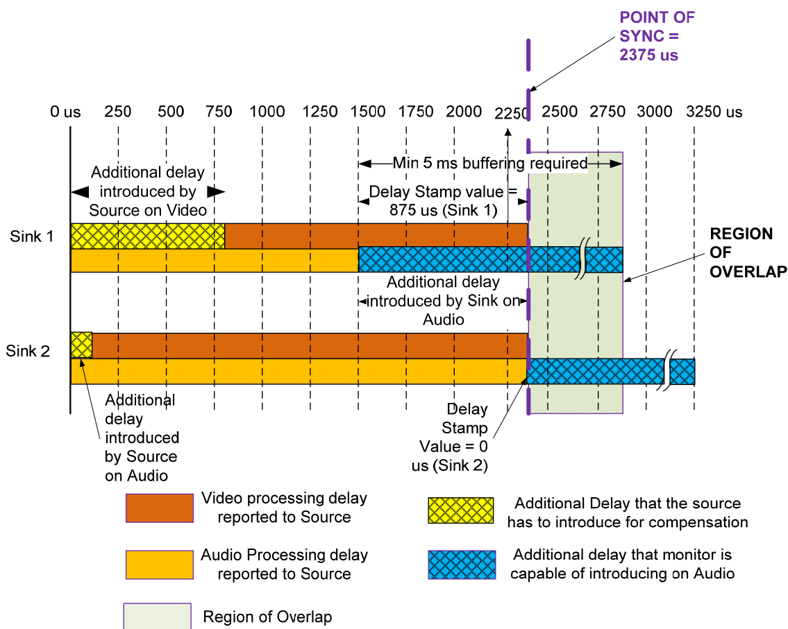
Figure 2-102: Delay Compensation for Audio-to-Video Sync in a Multi-Monitor Configuration
