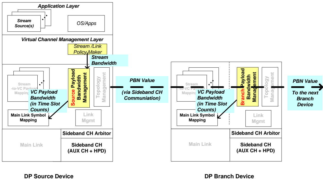
Figure 2-76: Bandwidth Management by Payload Bandwidth Manager
