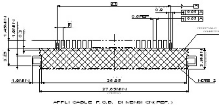
Figure 4-49: PCB Mount Connector Recommended Footprint Layout (in unit of mm)
