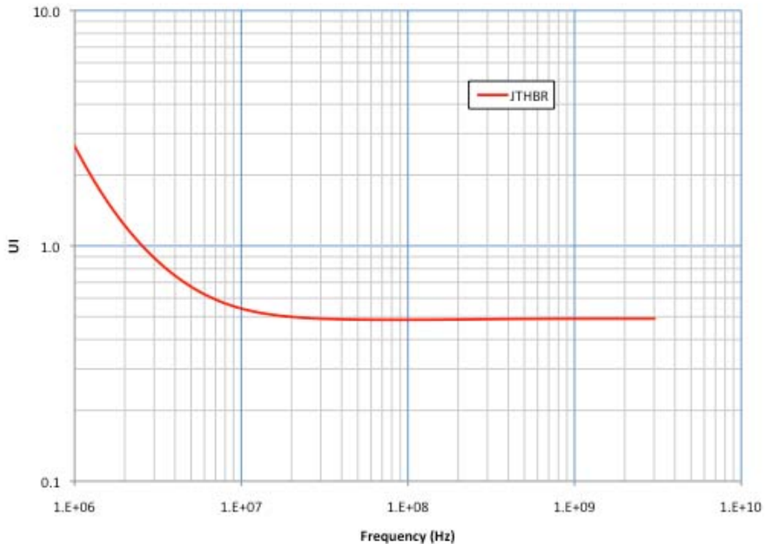
Figure 3-36: High Bit Rate Jitter Output/Input Tolerance Mask
