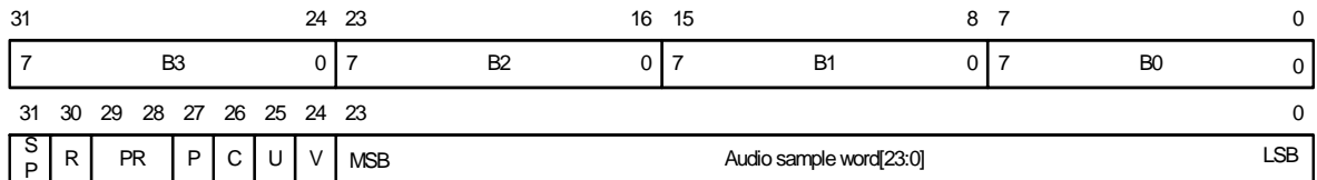
Figure 2-25: Data Mapping Within the 4-Byte Payload of an Audio_Stream Packet
