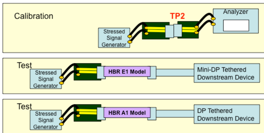
Figure 3-11: RBR Tethered Downstream Device Compliance Test Configuration
