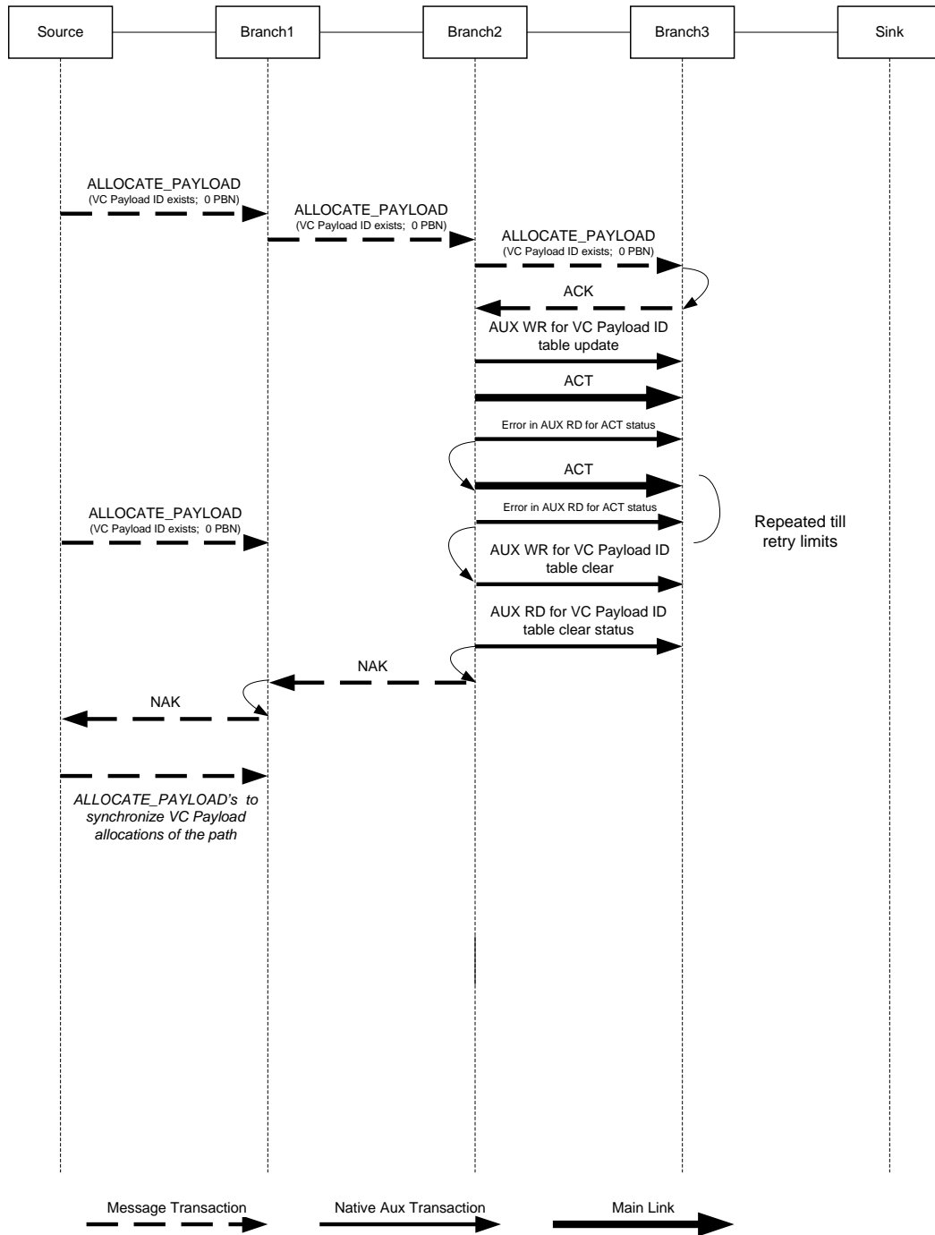
Figure 2-83: Timing Sequence for Deleting a Payload with Locally Unrecoverable Error
