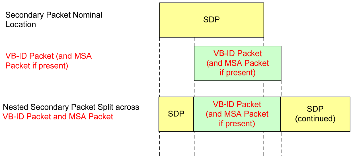
Figure 2-75: SDP Splitting
