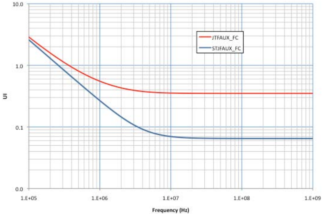
Figure 3-27: FAUX Forward Channel Receiver Jitter Output/Input Tolerance Mask
