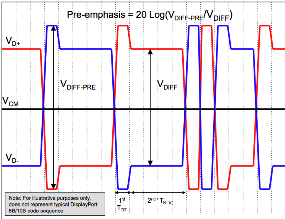
Figure 3-18: Example of Pre-emphasis
