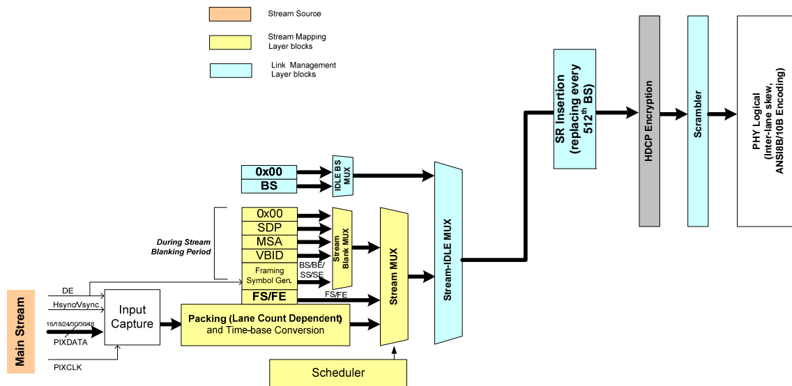
Figure 2-64: Logical Block Diagram of SST DP Source Device
