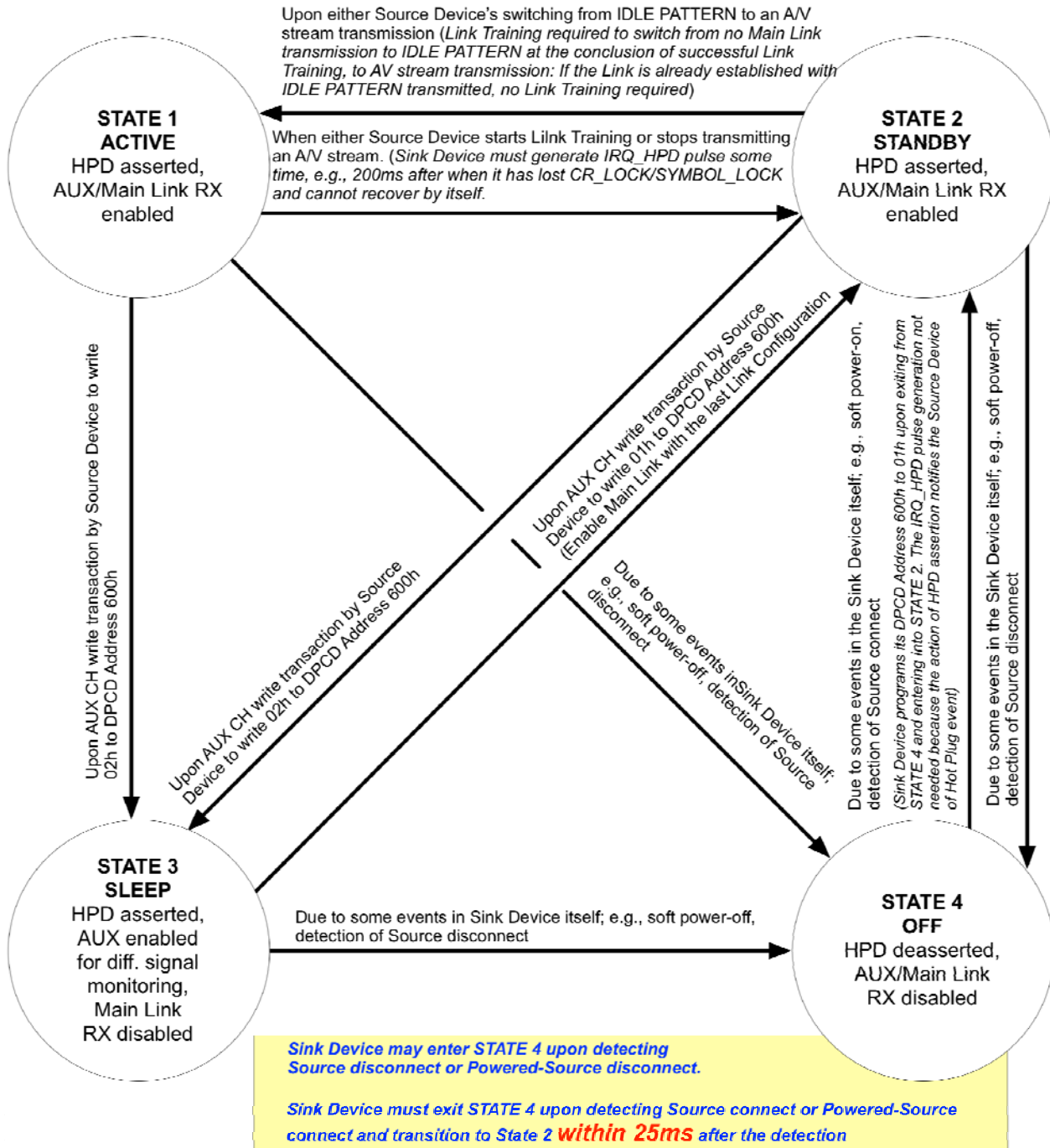
Figure 12-3: Link Quality Management Sink Power State Extension
