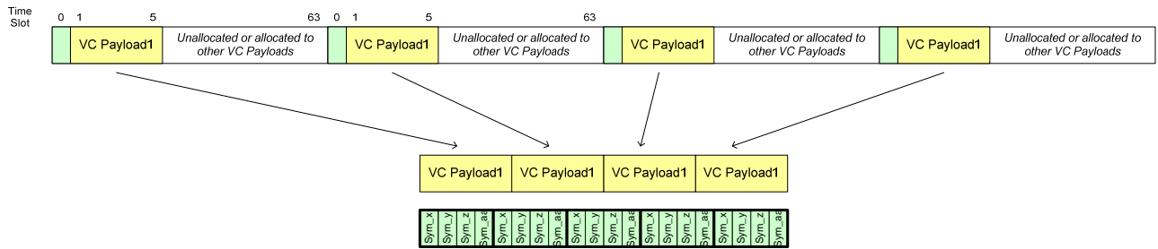
Figure 2-70: Repetition of 4-symbol Sequence Unit Example for 1-lane Main Link
