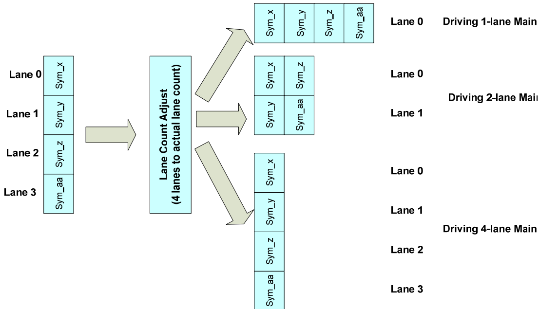
Figure 2-69: 4-symbol Sequence Unit Mapping to Main Link lanes
