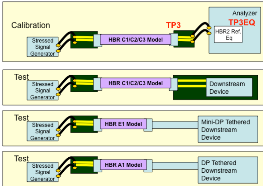
Figure 3-5: HBR2 Downstream Device Compliance Test Configuration
