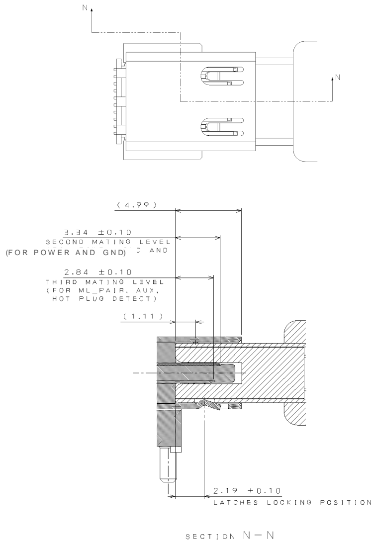
Figure 4-43: Fully-Mated Mini DisplayPort Connector Showing Mating Levels
