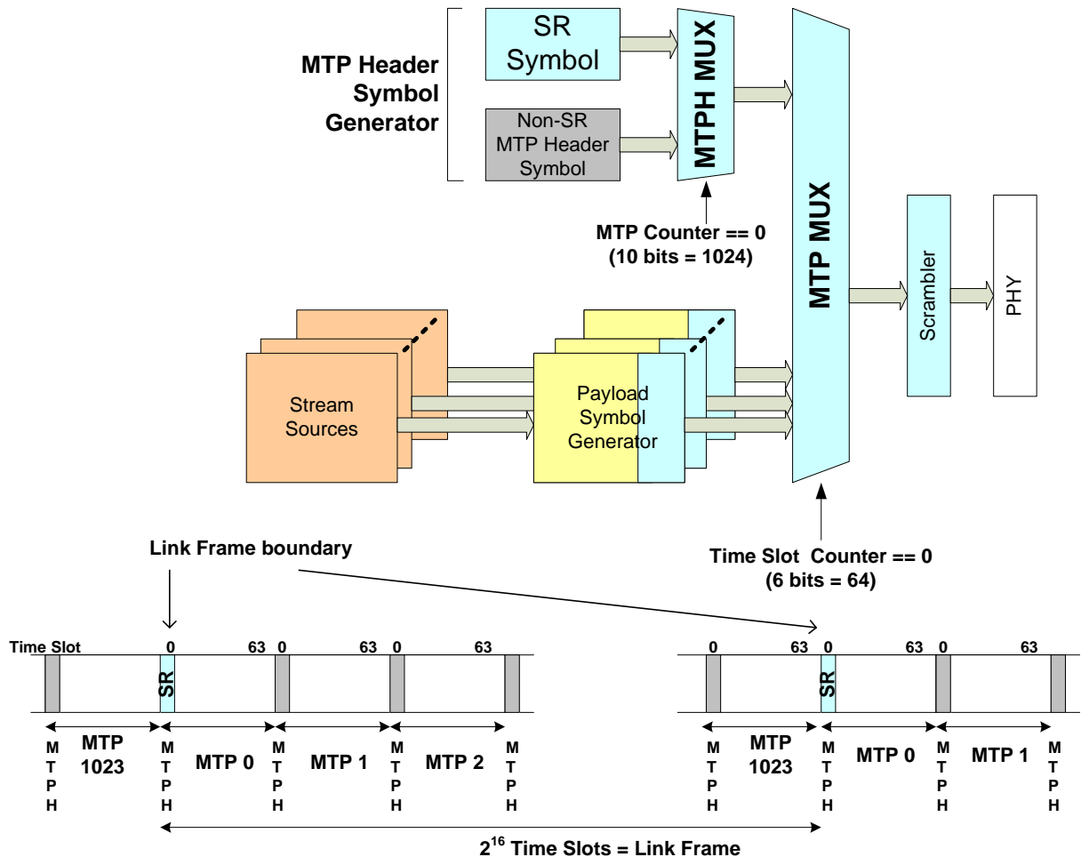
Figure 2-66: Link Timing Generation in MST Mode
