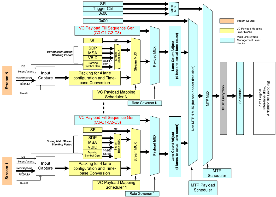
Figure 2-61: Logical Block Diagram of MST DP Source Device
