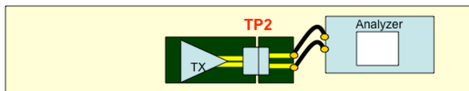
Figure 3-9: RBR Upstream Device Compliance Test Configuration
