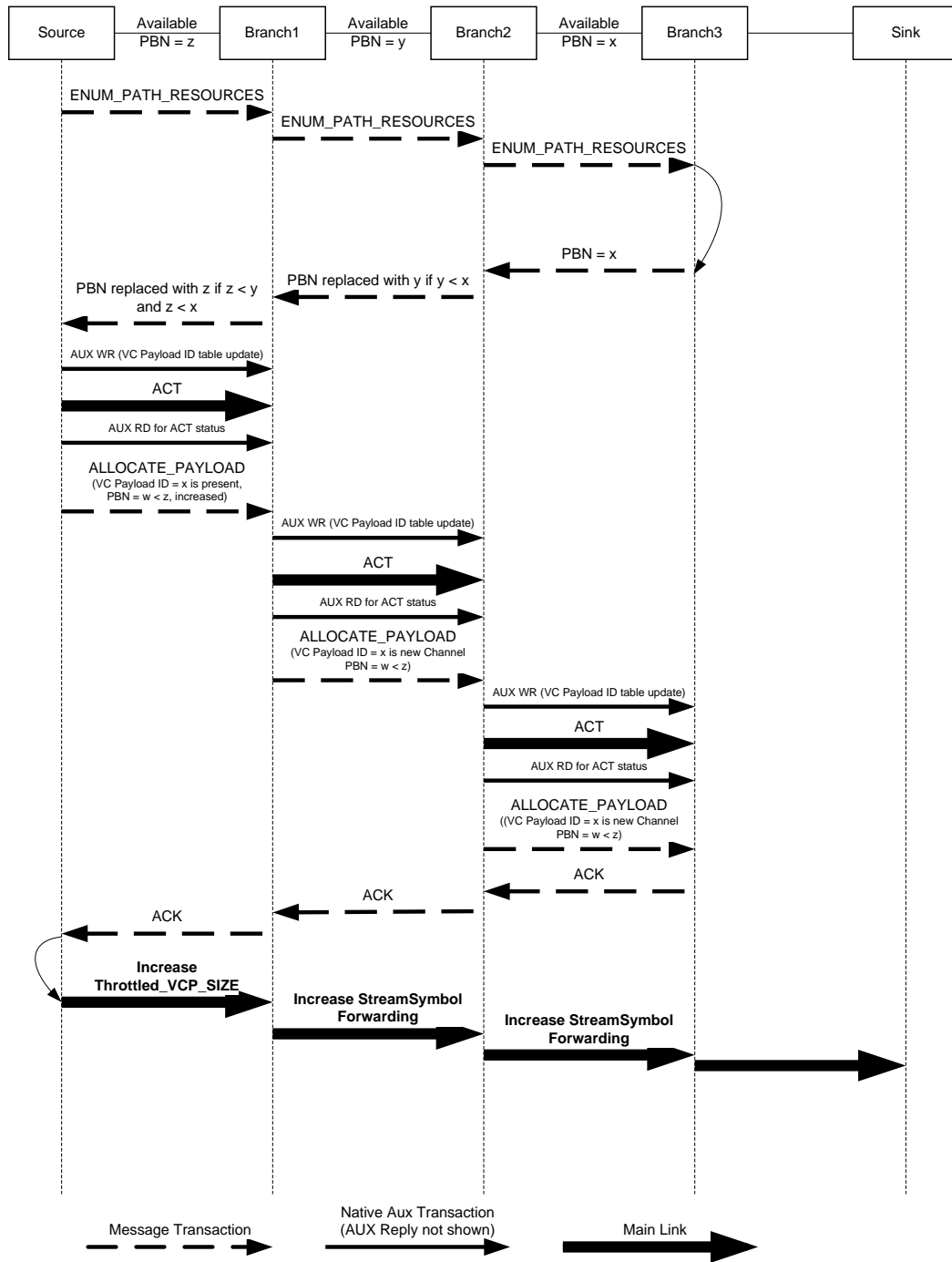
Figure 2-85: Timing Sequence for Increasing the VC Payload Allocation
