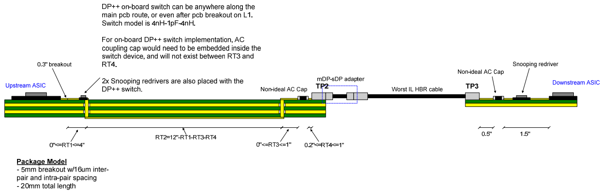
Figure 9-3: FAUX Channel Topology Assumption
