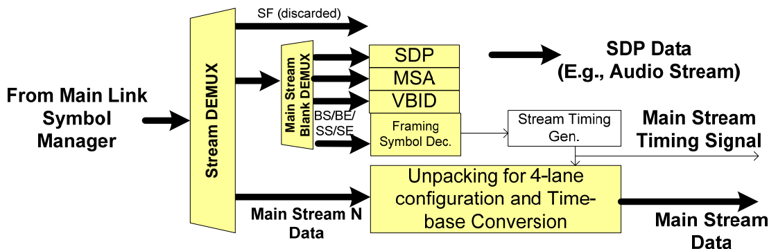
Figure 2-73: DP Sink Device VC Payload Mapping Logical Block Diagram
