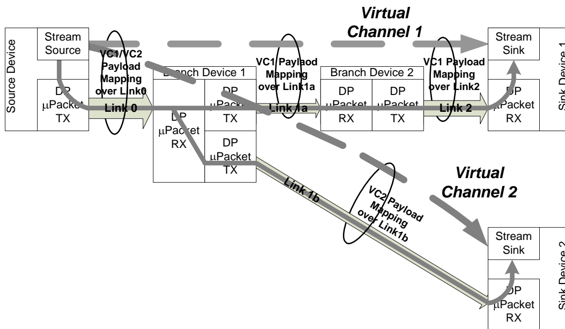
Figure 2-48: Single Stream Source to Two Stream Sinks (“Dual Display Clone”)
