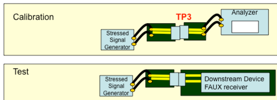
Figure 3-13: FAUX Forward Channel Receiver Compliance Test Configuration
