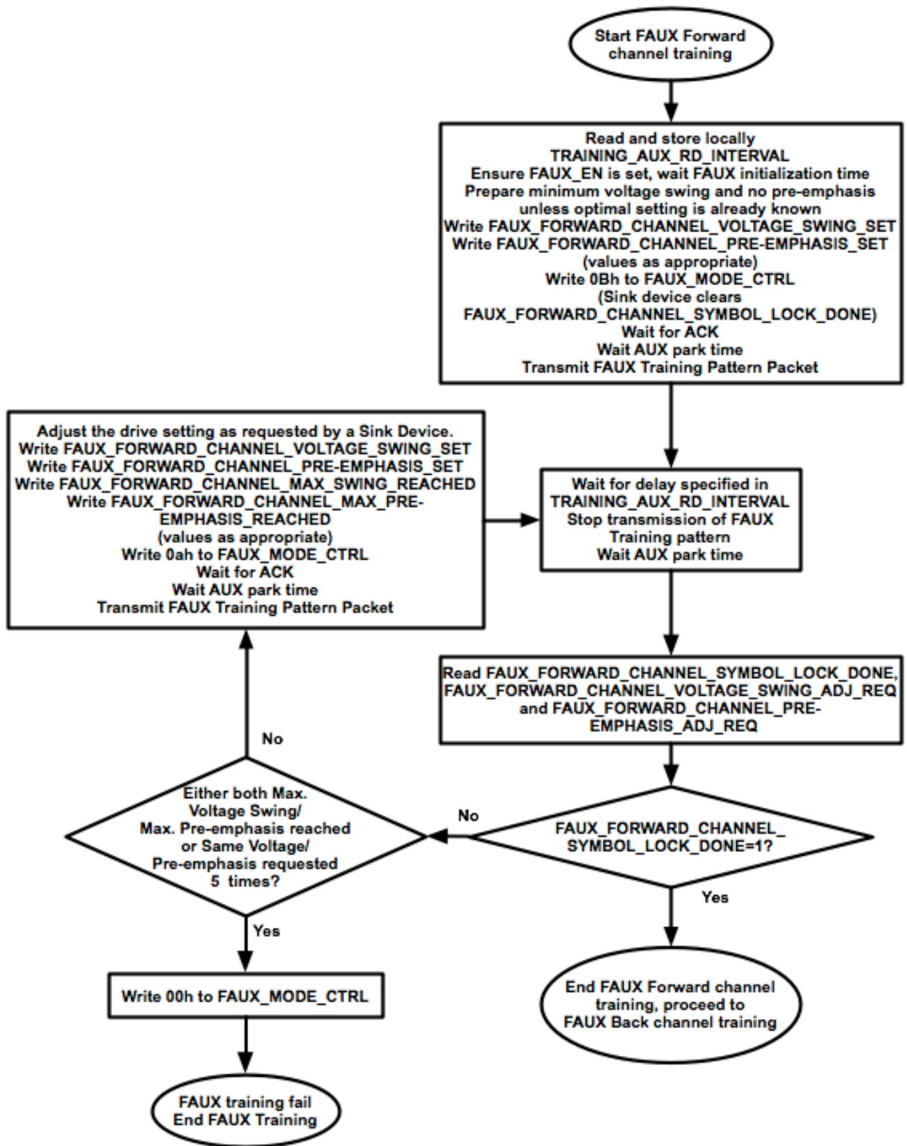
Figure 3-25: FAUX Forward Channel Training
