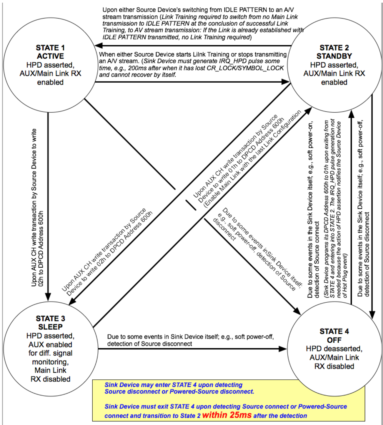
Figure 5-2: Sink Power State Machine
