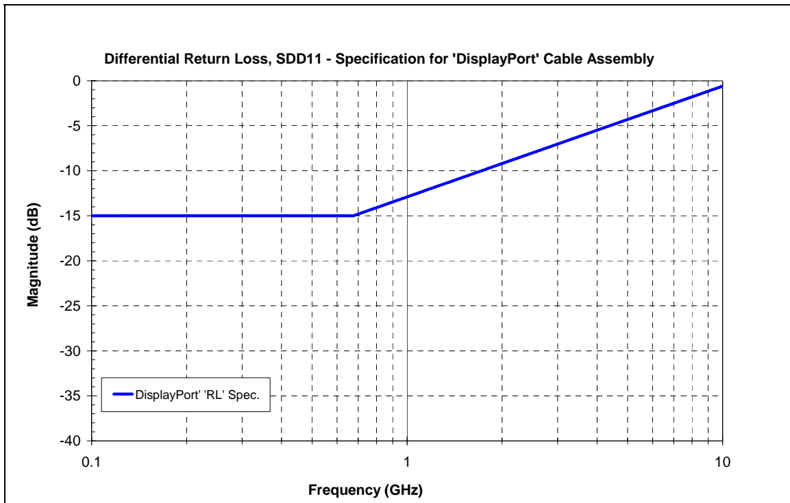
Figure 4-13: Mixed Mode Differential RL for HBR Cable Assembly/Adaptor (DP Connector)
