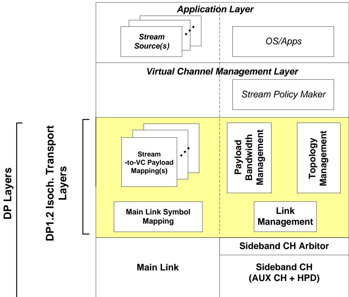
Figure 2-51: MST Isochronous Transport Service Layers
