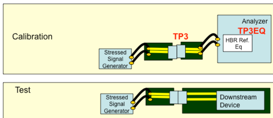
Figure 3-7: HBR Downstream Device Compliance Test Configuration
