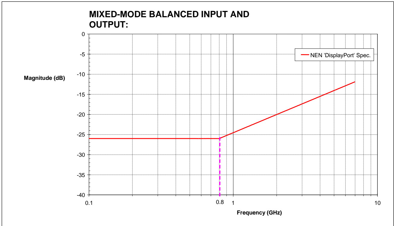
Figure 4-21: Near-End Total Noise (peak) for Reduced Bit Rate Cable Assembly
