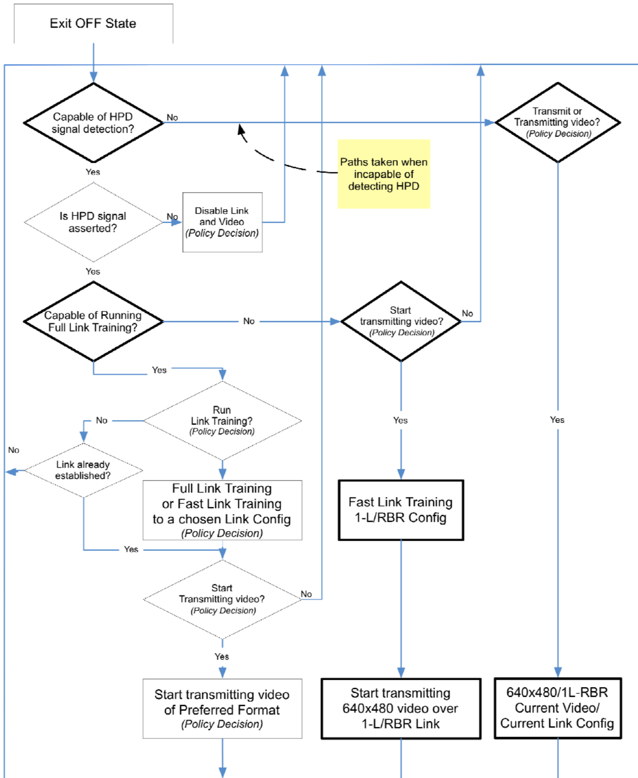
Figure 12-2: Link Quality Management Source Safe Mode
