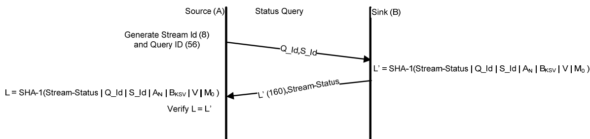
Figure 14-1: QUERY_STREAM_ENCRYPTION_STATUS Message Transaction Execution when a Source Device is Directly Connected to an MST Sink Device
