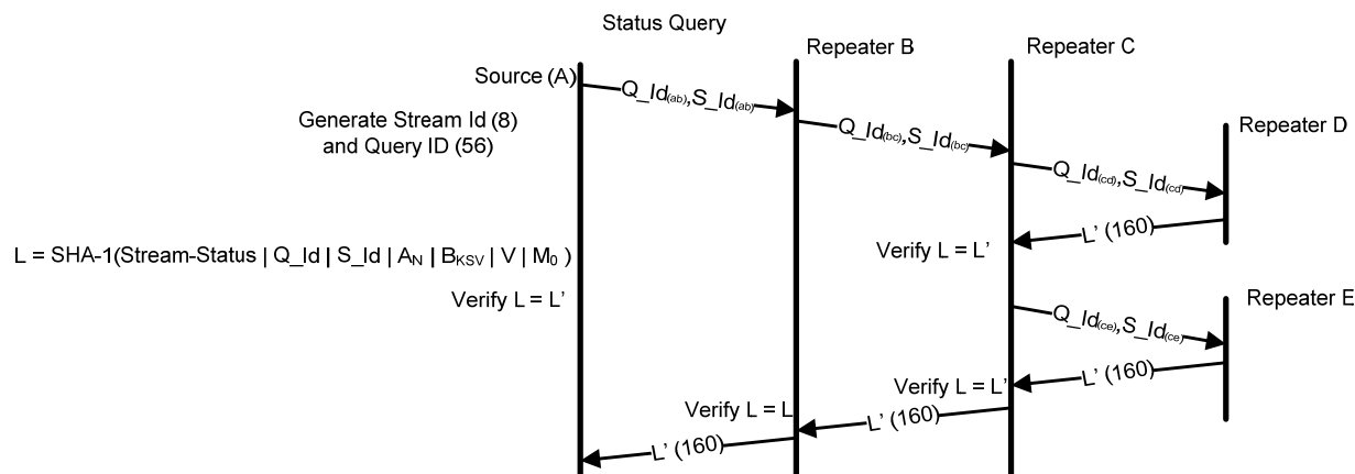
Figure 14-2: QUERY_STREAM_ENCRYPTION_STATUS Message Transaction Forwarding and Execution when a Source Device is Connected to a Sink Device via MST Branch Devices
