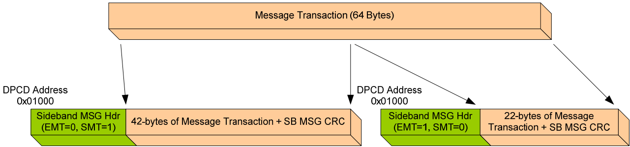
Figure 2-94: Mapping Message Transaction to Multiple Sideband MSGs (SB MSG CRC is the Sideband_MSG_Data_CRC field.)
