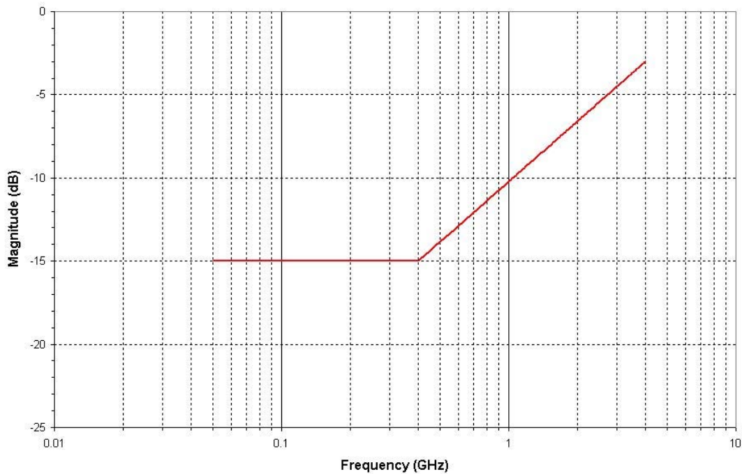
Figure 4-20: Mixed Mode Differential Return Loss (SDD11) of Reduced Bit Rate Cable
