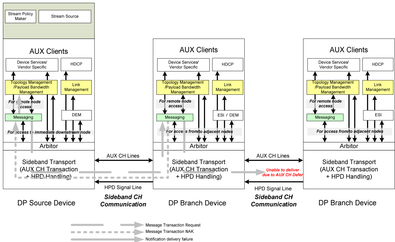
Figure 2-96: AUX CH Error While Delivering a Down Req Message
