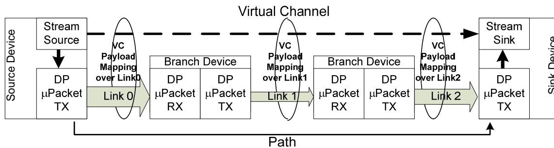
Figure 2-47: Illustration of Link, Path, Virtual Channel
