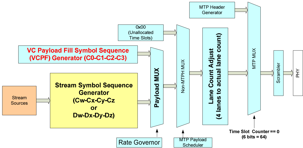
Figure 2-68: VC Payload Symbol Generator of a DP Source Device
