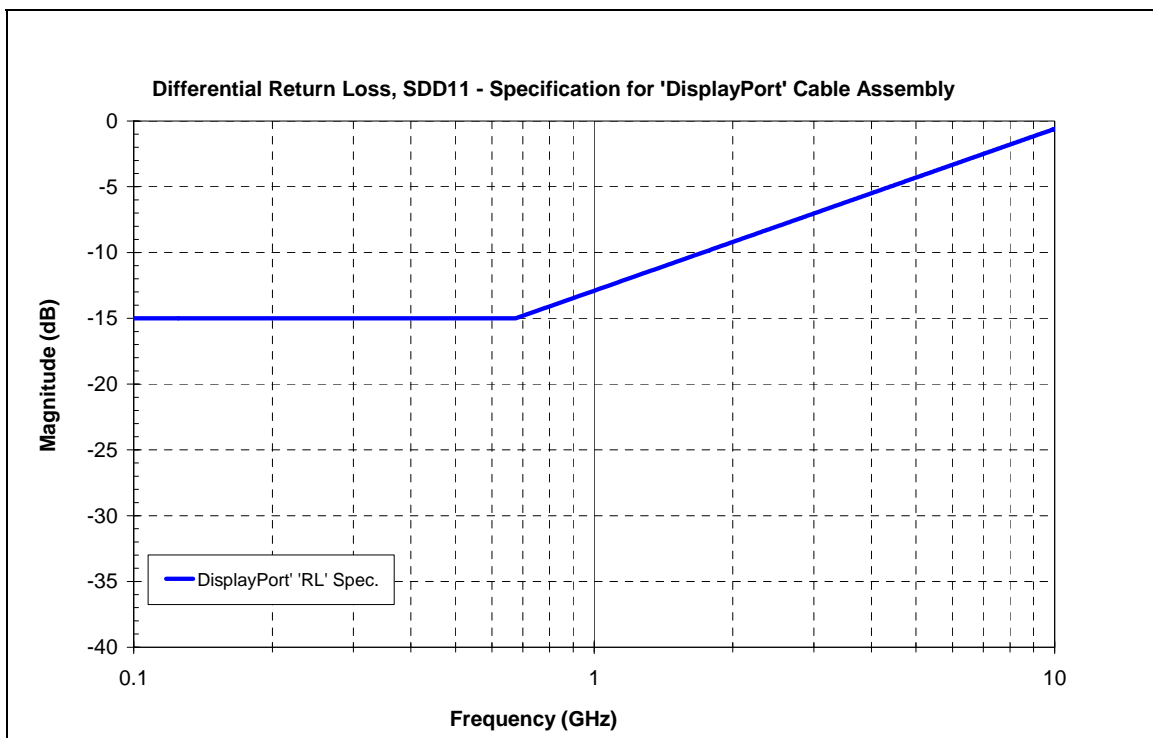
Figure 4-14: Mixed Mode Differential RL for HBR Cable Assembly/Adaptor (mDP Connector)
