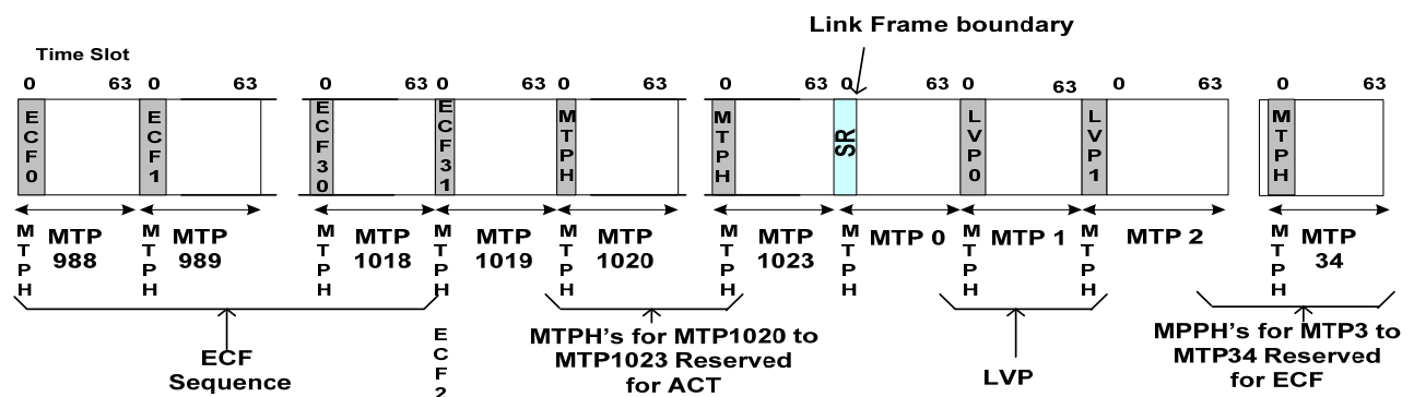
Figure 2-86: MSTM ECF and LVP Signaling at Link Frame Boundary
