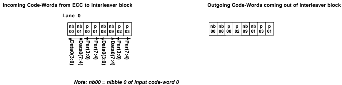
Figure 2-40: ECC Block Nibble-Interleaving for a 1-Lane Main Link (Header)
