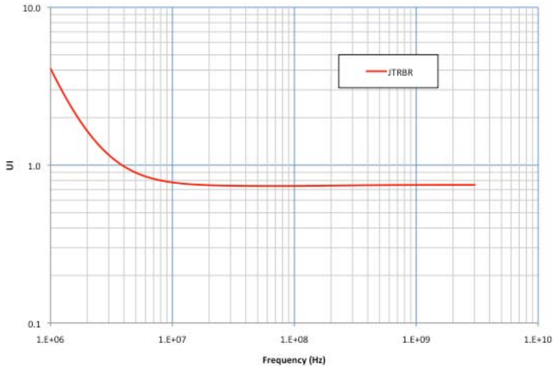
Figure 3-37: Reduced Bit Rate Jitter Output/Input Tolerance Mask
