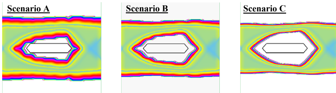
Figure 9-4: Effects on RX Silicon Eye with Different Aggressor Setups
