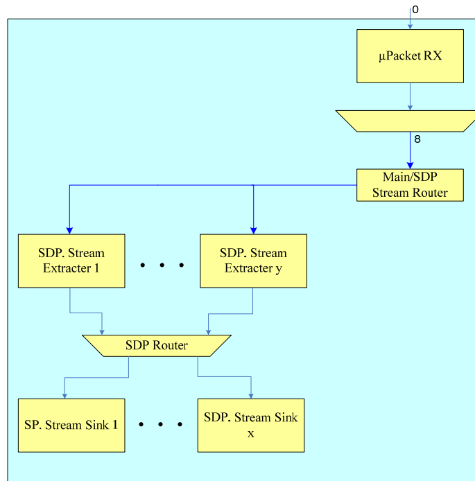
Figure 2-56: MST Audio-only Sink Device with SDP Sinks
