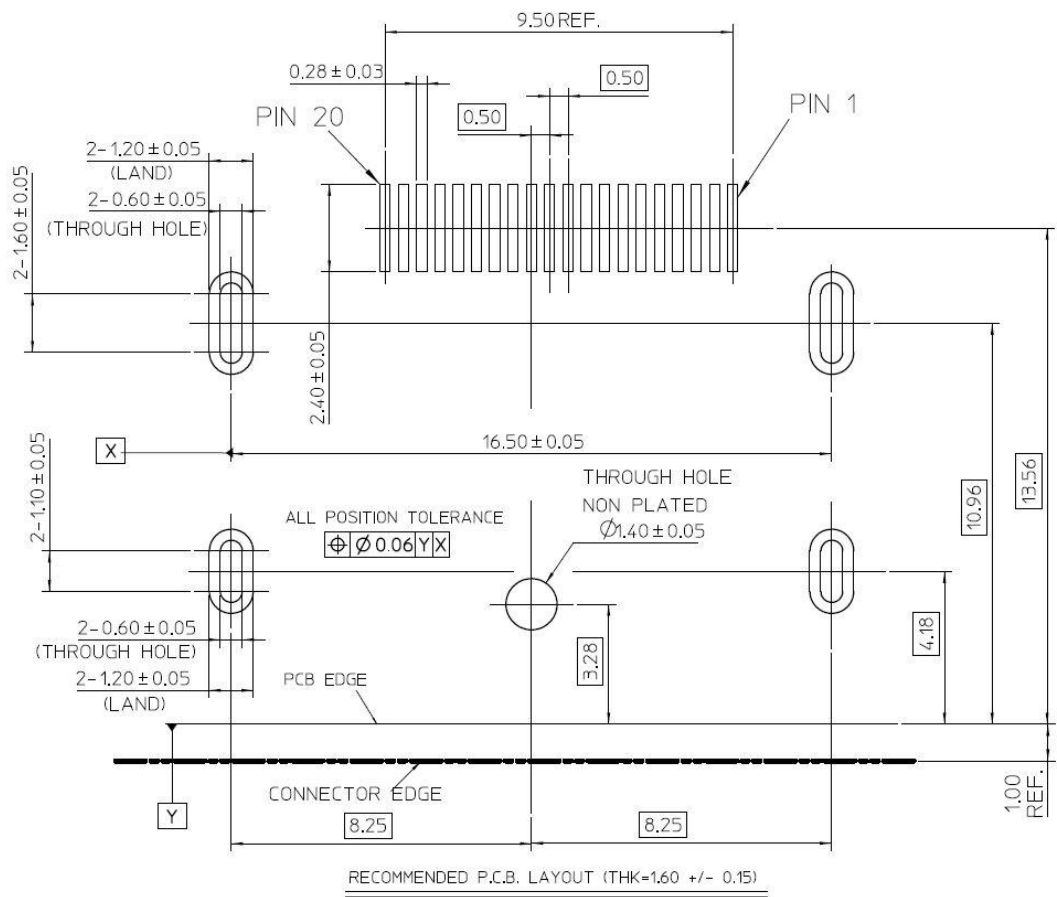
Figure 4-30: Recommended PCB Layout for DisplayPort External Connector
