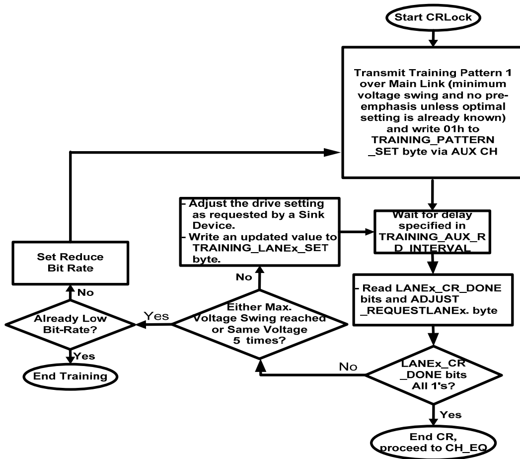
Figure 3-32: Clock Recovery Sequence of Link Training
