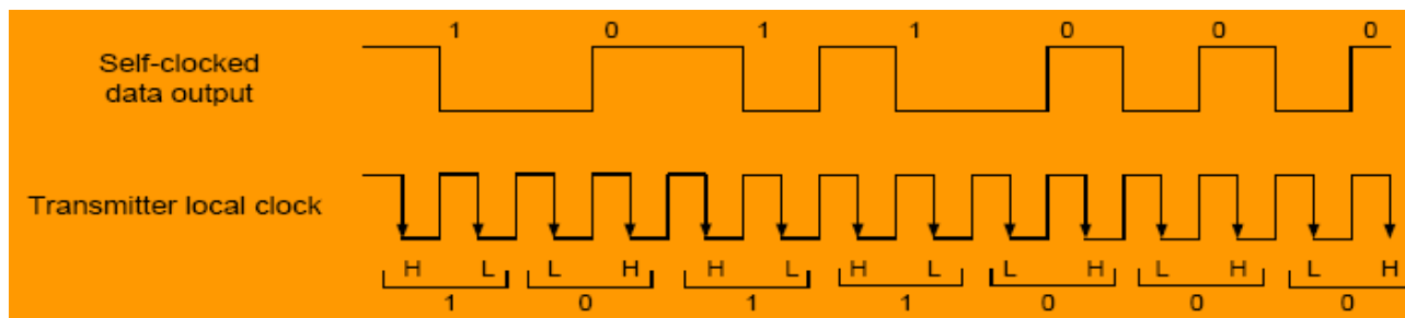
Figure 3-23: Self-clocking with Manchester-II Coding
