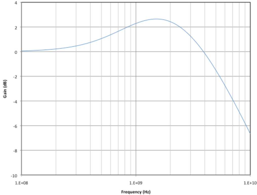
Figure 3-40: Reference HBR Receiver Equalizer Transfer Function
