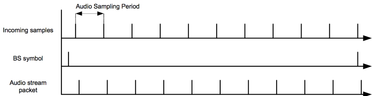
Figure 6-1: Audio Stream Packets Transfer with No Video or During Video Vertical Blanking
