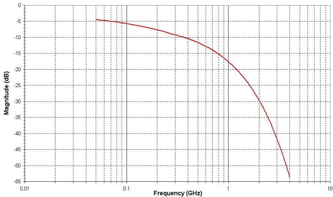
Figure 4-19: Mixed Mode Differential Insertion Loss (SDD21) Mask of Reduced Bit Rate Cable
