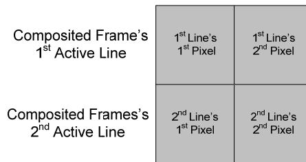
Figure 13-1: Pixel Pattern Representation for Pixel Interleaved Method
