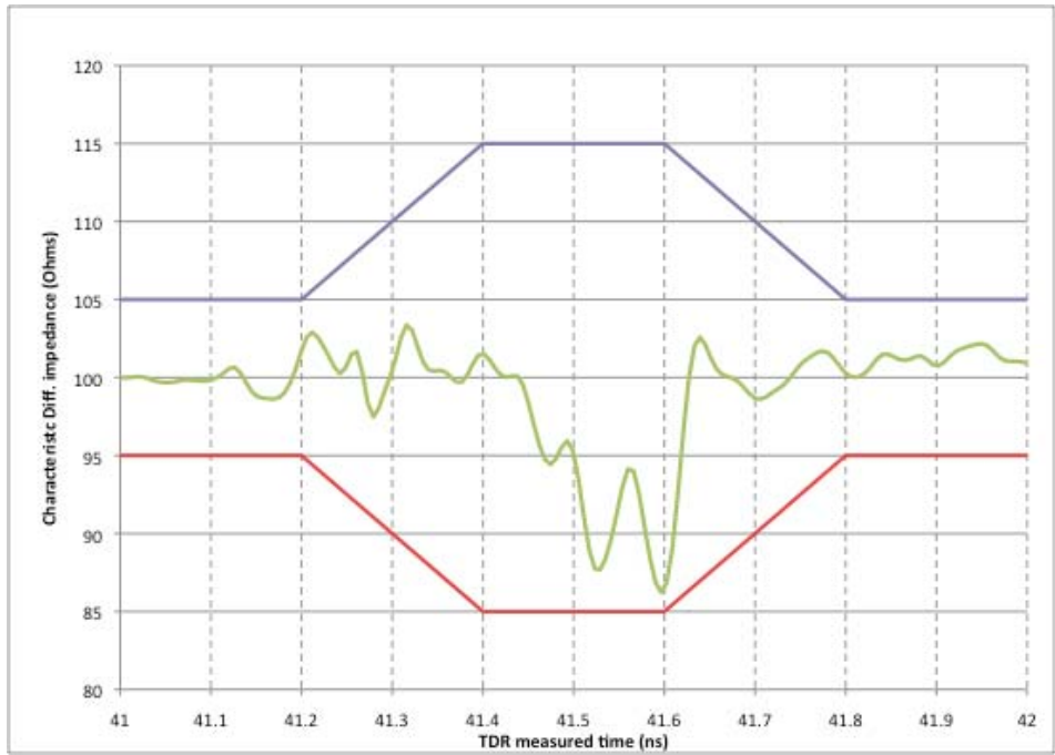
Figure 4-9: Mini DP Differential Impedance Profile Measurement Data Example
