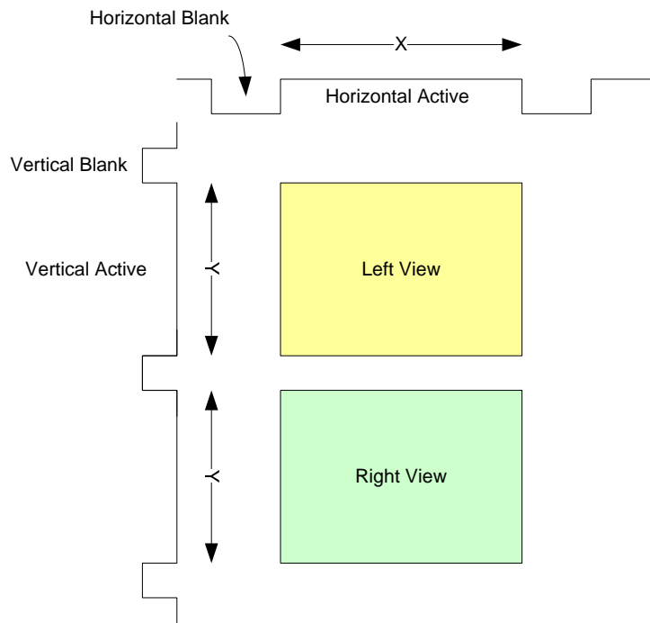
Figure 13-5: Field Sequential Stereo Format with Left View and Right View Indicated via MISC1 Bits 2:1 Field of the MSA
