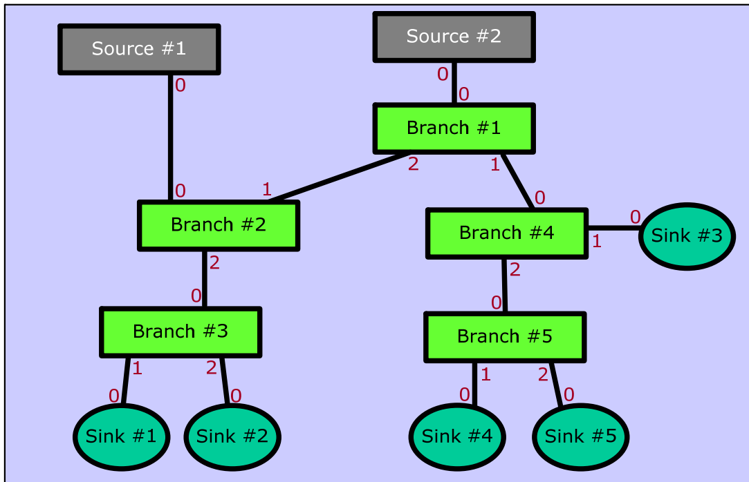
Figure 2-57: Example MST (Multi-stream Transport) Topology
