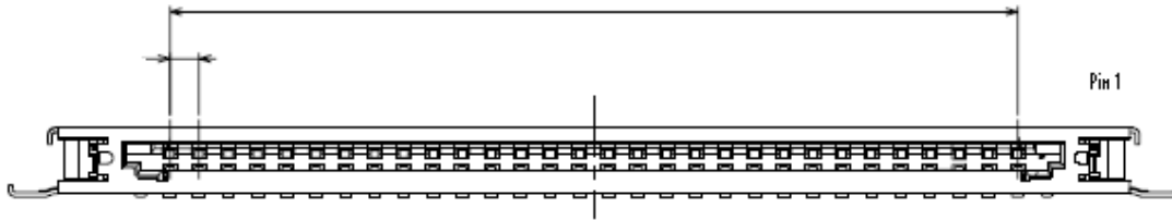
Figure 4-47: Panel-side Internal PCB Mount Receptacle Connector with Pin 1 Shown
