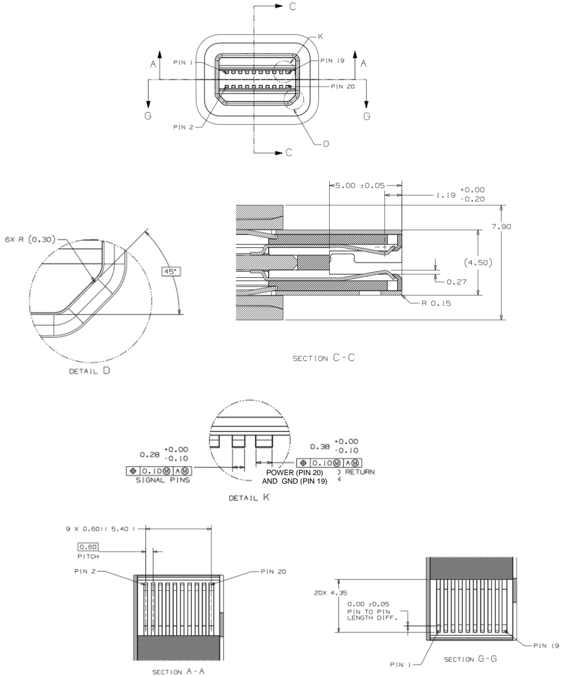
Figure 4-39: Mini DisplayPort Cable-Connector Dimensions – 1
