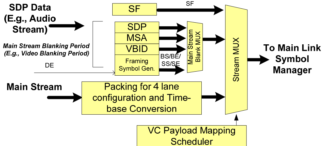
Figure 2-72: DP Source Device VC Payload Mapping Logical Block Diagram
