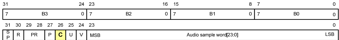
Figure 2-105: Using the C Field of the Audio Sampling Packet for GTC Transmission
