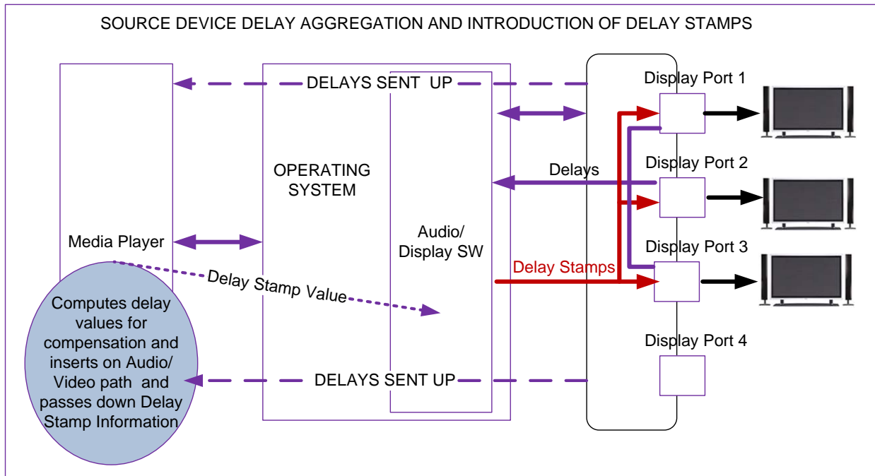
Figure 2-98: Source Device Delay Aggregation and Introduction of Delay Stamps
