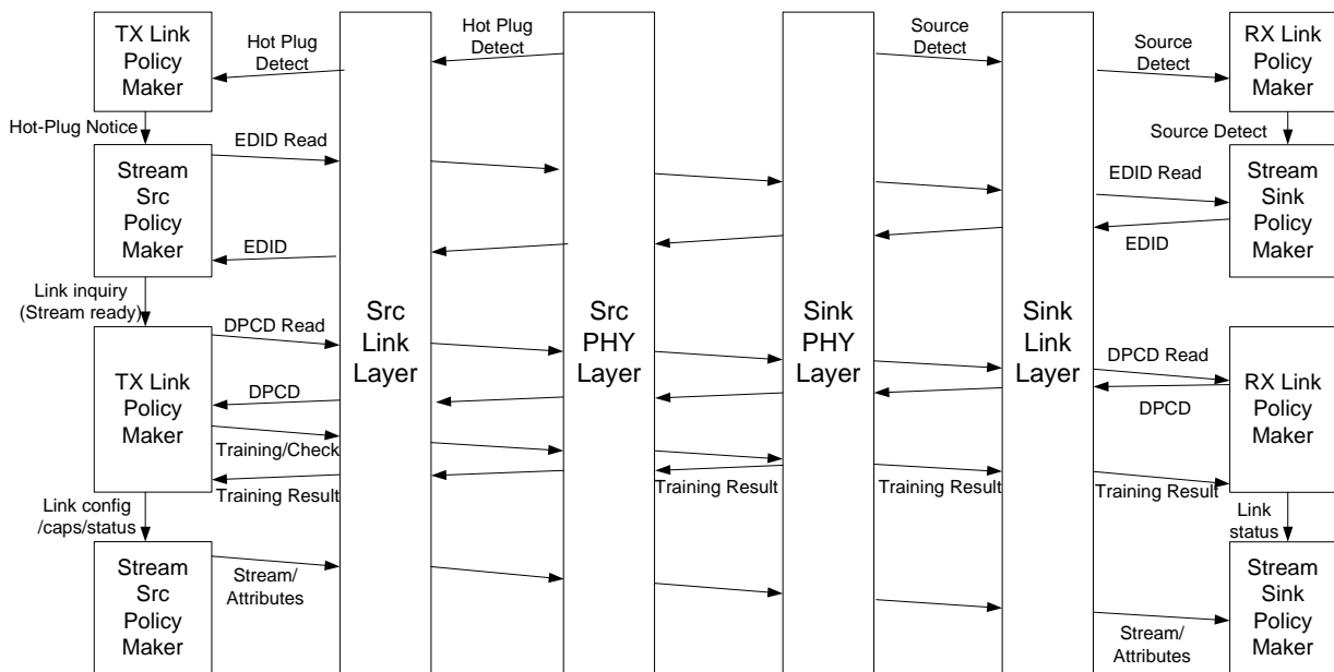
Figure 2-89: Action Flow Sequences of the Source upon HPD Event (Informative)
