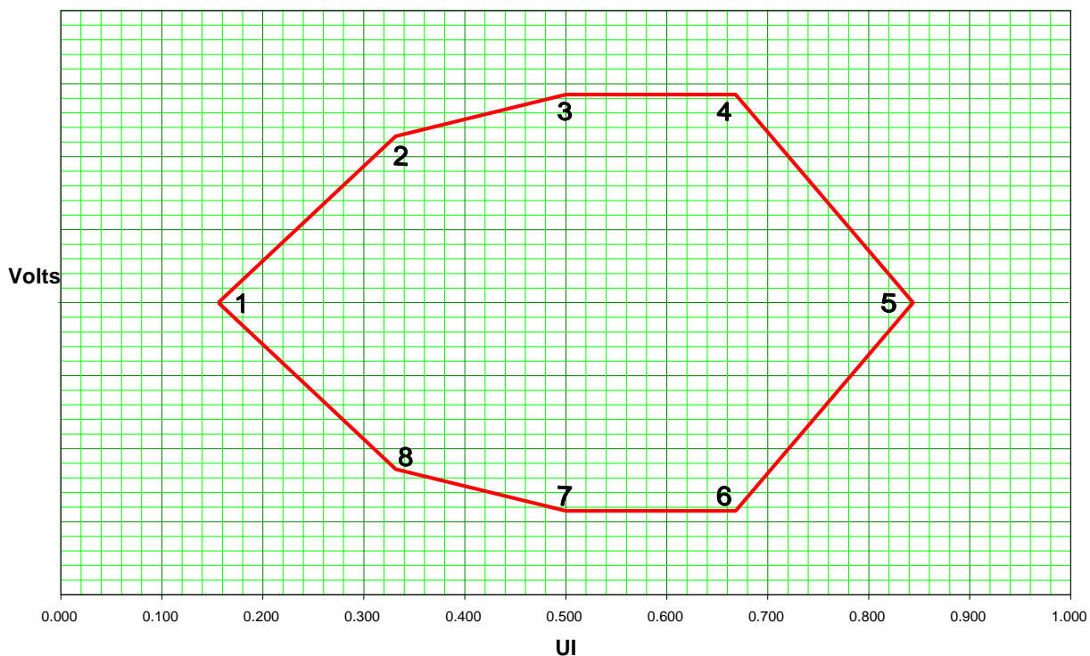
Figure 3-38: EYE Mask at Upstream Device Connector Pins
