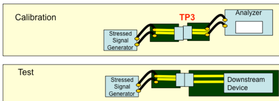
Figure 3-10: RBR Downstream Device Compliance Test Configuration
