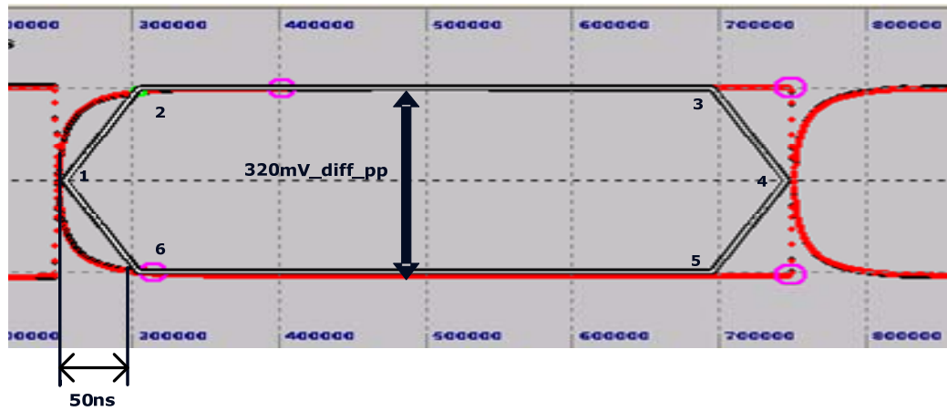
Figure 9-2: AUX CH EYE Mask at Receiving IC Package Pins (Informative)
