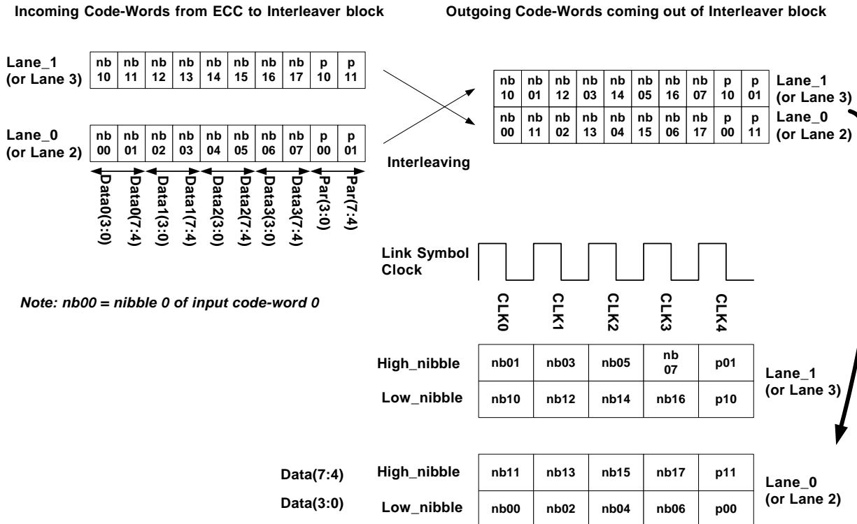
Figure 2-37: ECC Block Nibble-Interleaving for 2- and 4-Lane Main Links
