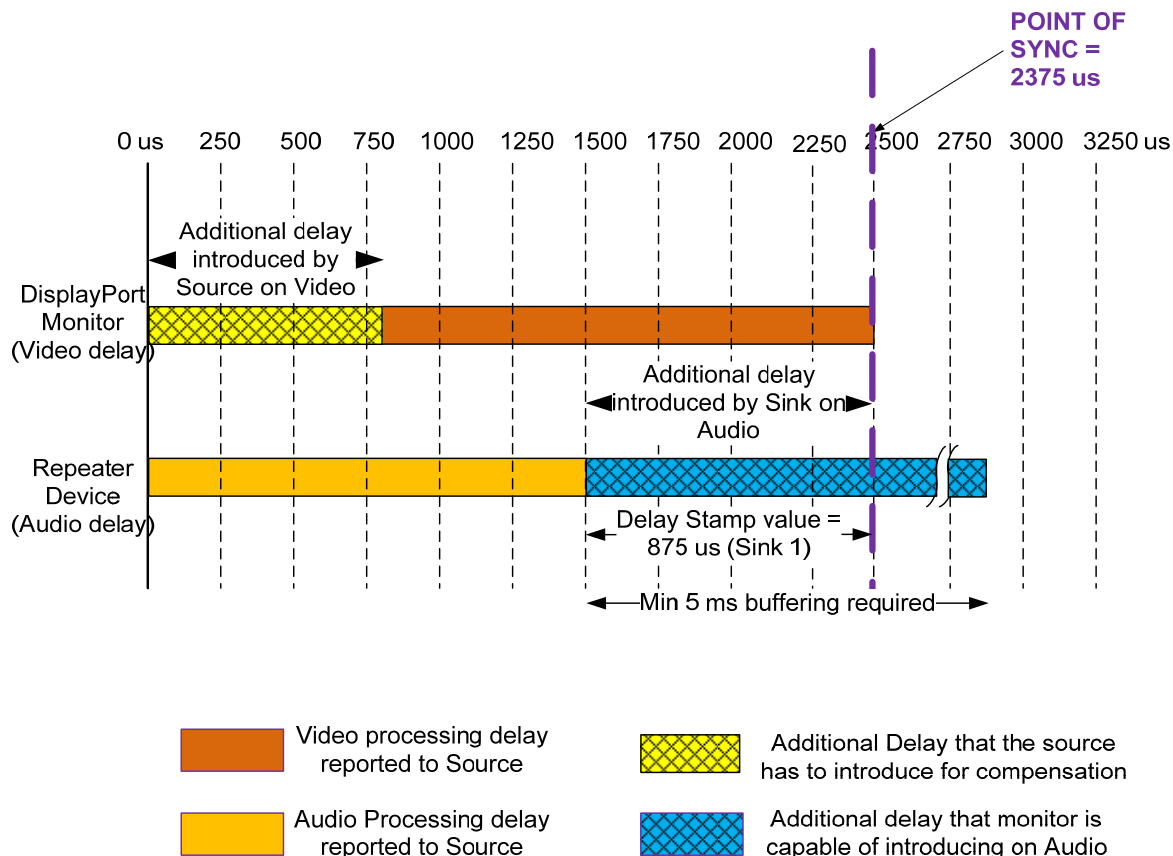
Figure 2-100: Delay Compensation for Audio-to-Video Synchronization
