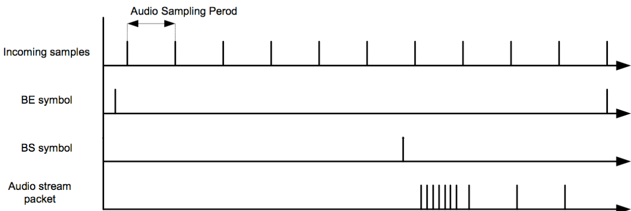
Figure 6-2: Audio Stream Packets Transfer with Video during Video Vertical Active Period
