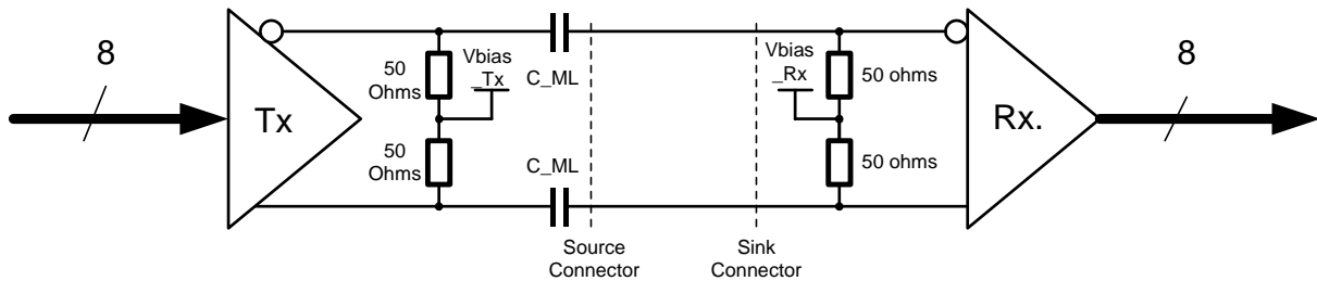
Figure 3-34: Main Link Differential Pair
