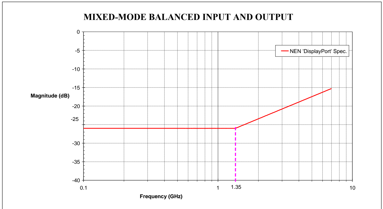
Figure 4-15: Near-End Total Noise (peak) for High Bit Rate Cable Assembly
