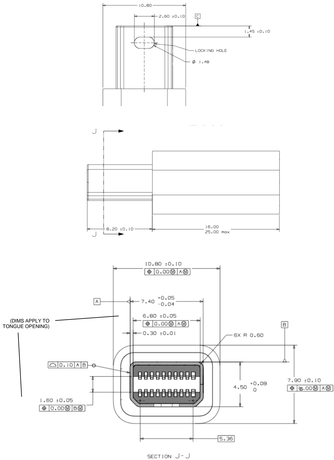
Figure 4-40: Mini DisplayPort Cable-Connector Dimensions – 2
