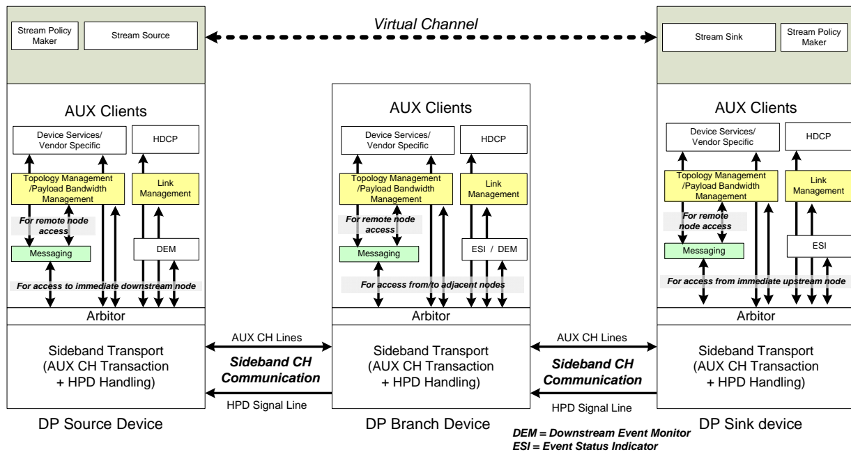
Figure 2-52: Sideband CH Communication Layers
