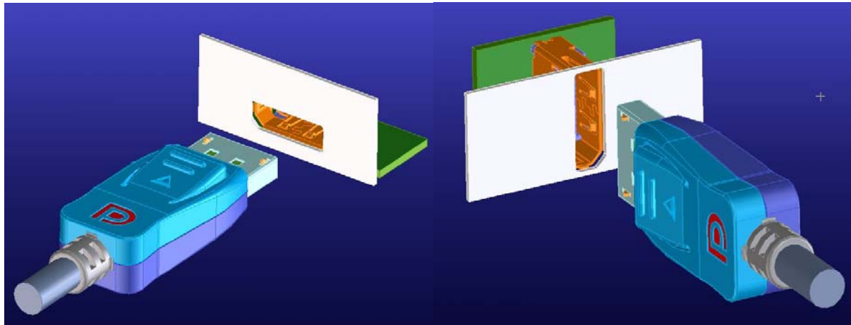
Figure 4-27: Recommended Orientation of External Connector
