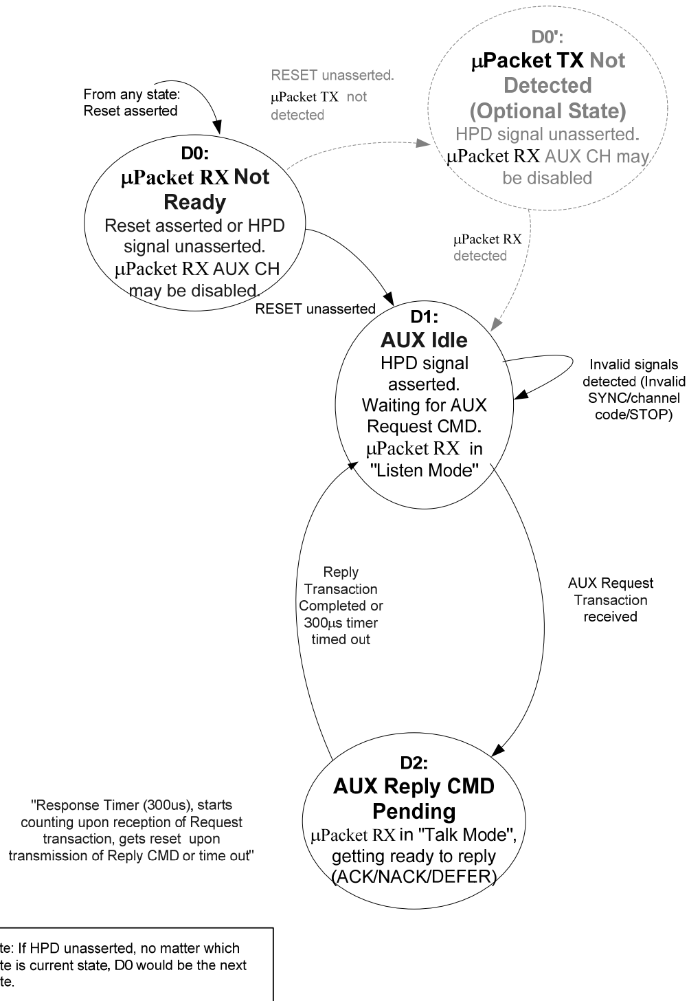
Figure 2-44: AUX CH uPacket RX State Diagram
