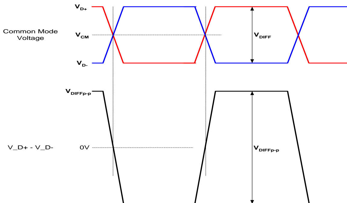
Figure 3-17: Definition of Differential Voltage and Differential Voltage Peak-to-Peak
