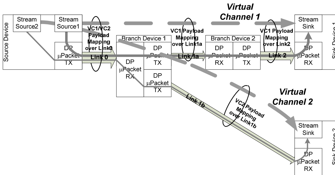
Figure 2-49: Two Stream Sources to Two Stream Sinks (“Extended Desktop”)
