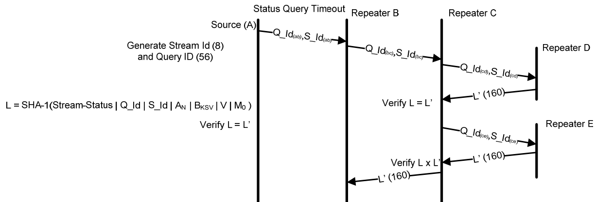
Figure 14-3: QUERY_STREAM_ENCRYPTION_STATUS Message Transaction Forwarding and Execution when L-to-L' Verification Error Present
