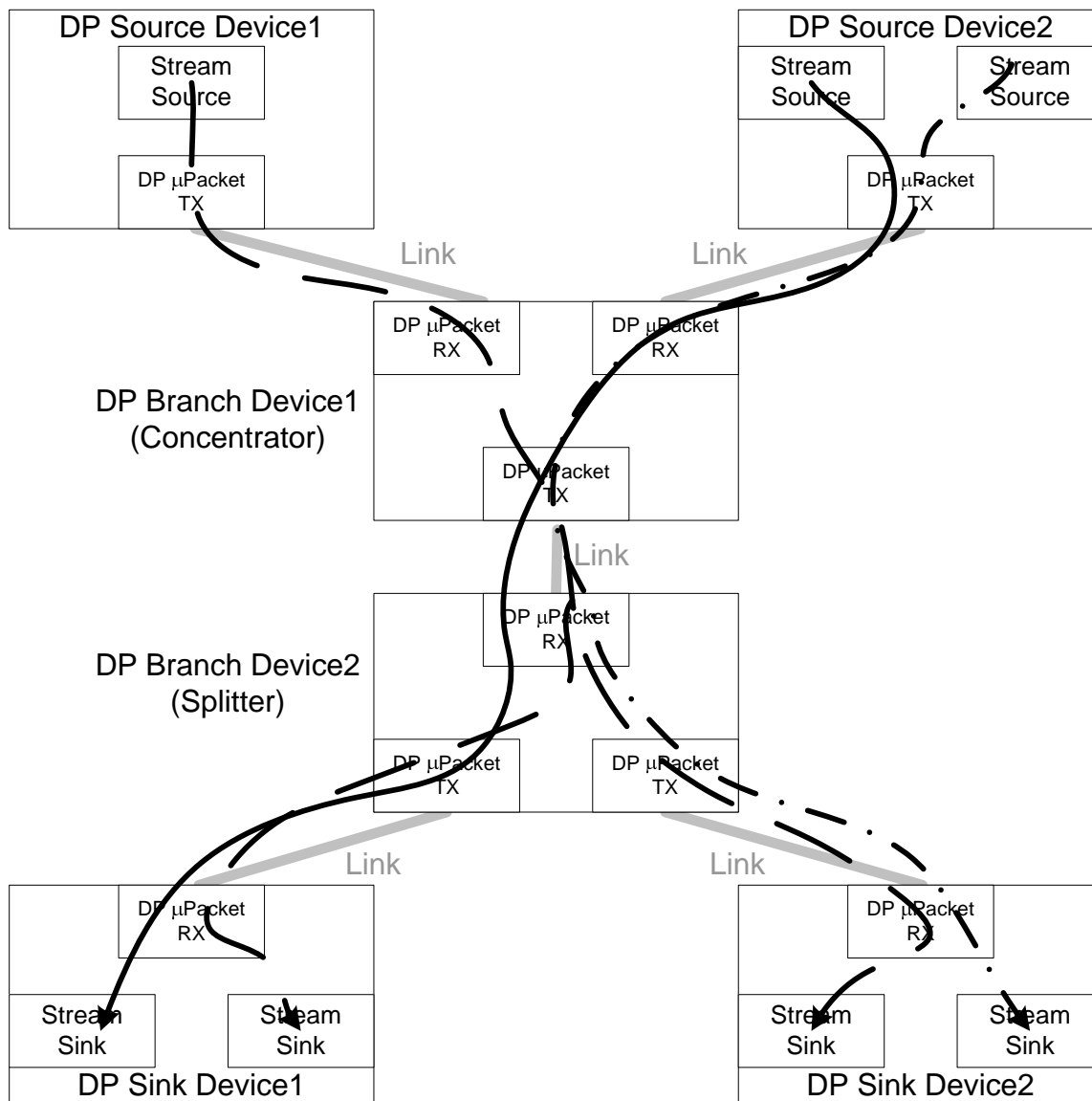
Figure 2-46: DP1.2 Multi-Stream Transport
