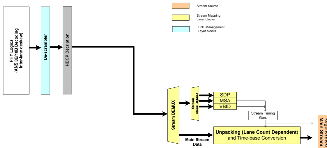
Figure 2-65: Logical Block Diagram of SST DP Sink Device
