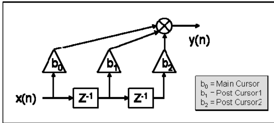
Figure 3-19: Feed-Forward Equalizer (FFE) Model
