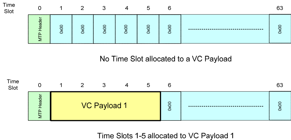
Figure 2-67: Time Slot Allocation to VC Payload
