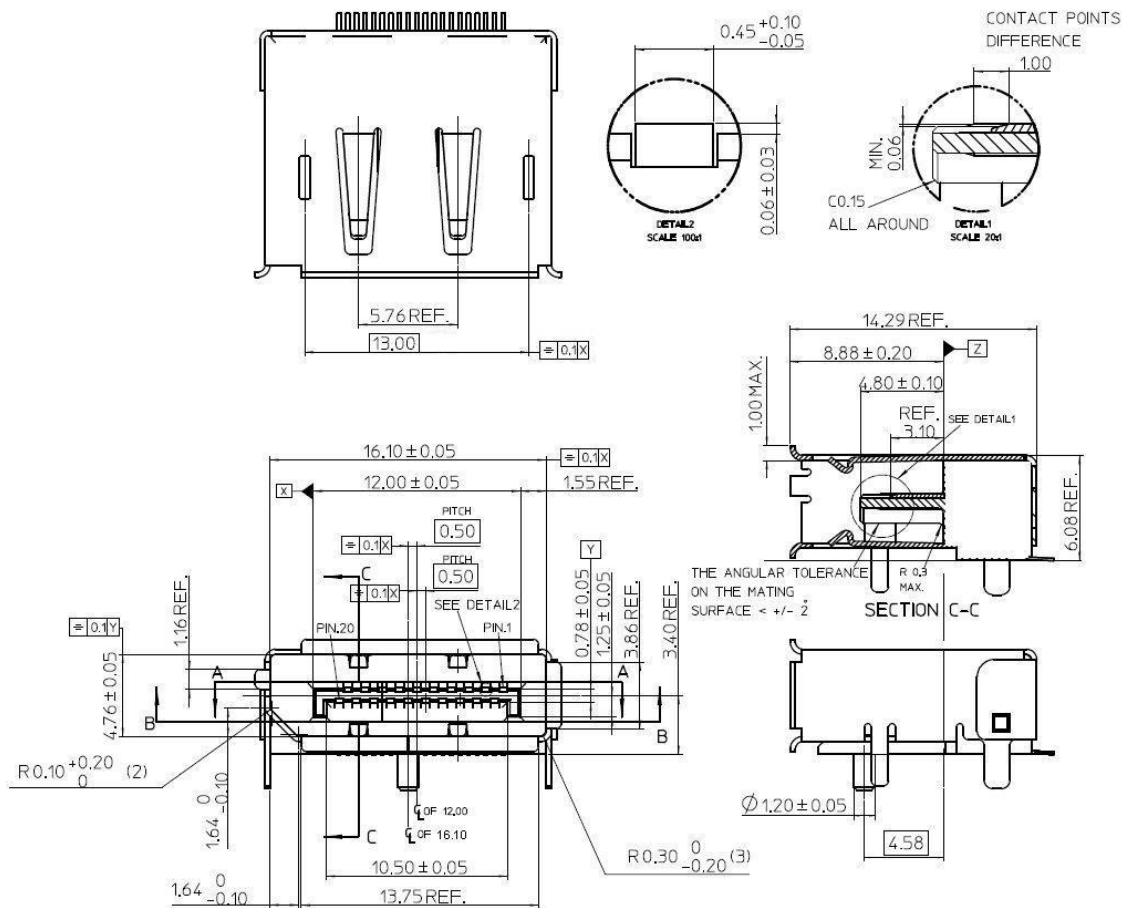
Figure 4-25: DisplayPort External Connector Drawings
