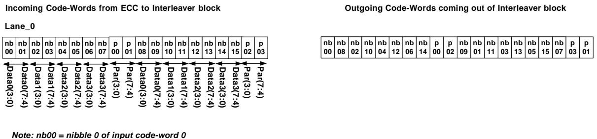
Figure 2-38: ECC Block Nibble-Interleaving for a 1-Lane Main Link
