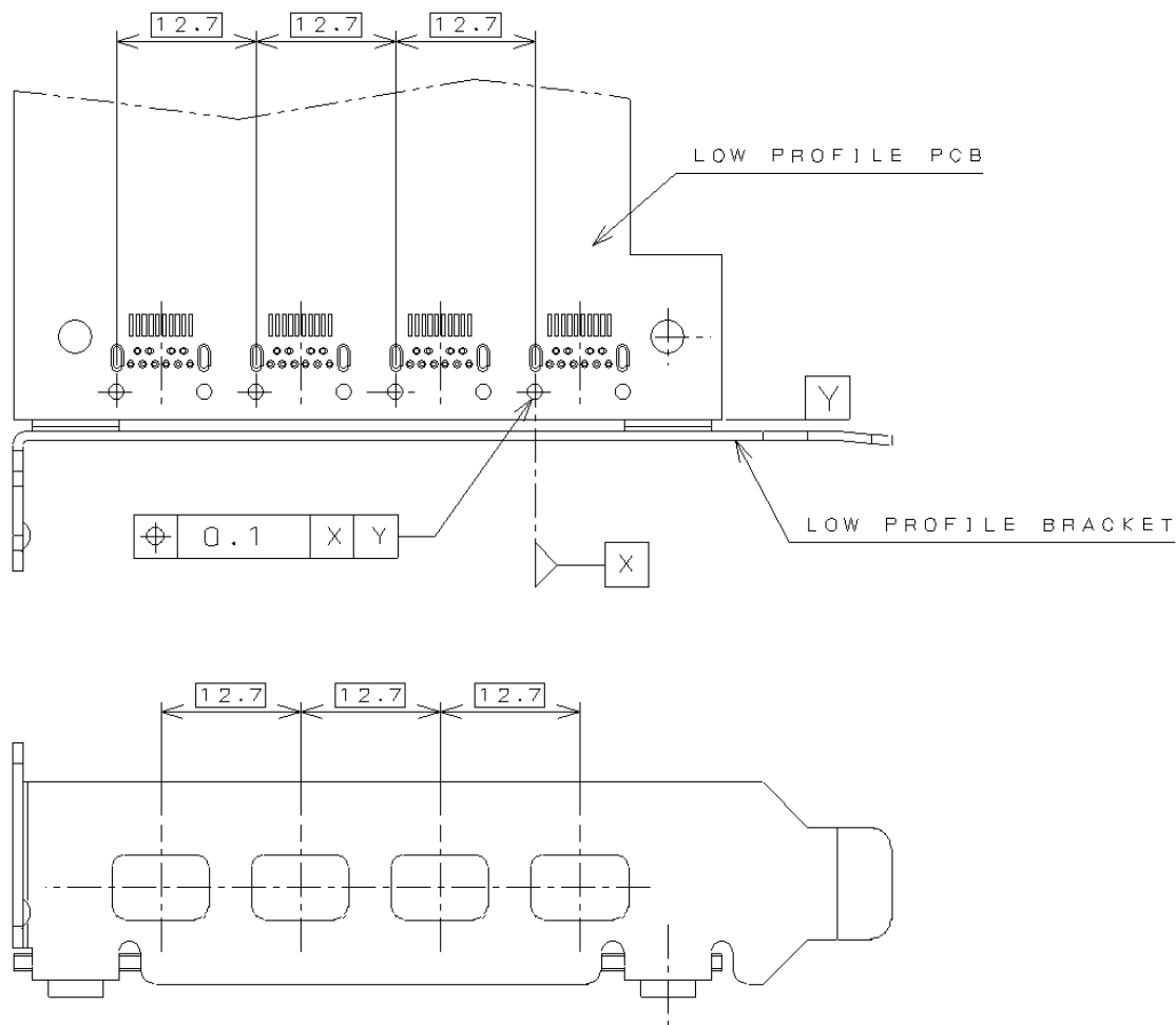
Figure 4-45: Reference Design for Four Mini DP Connectors on a Reduced Height PCI Card – 1
