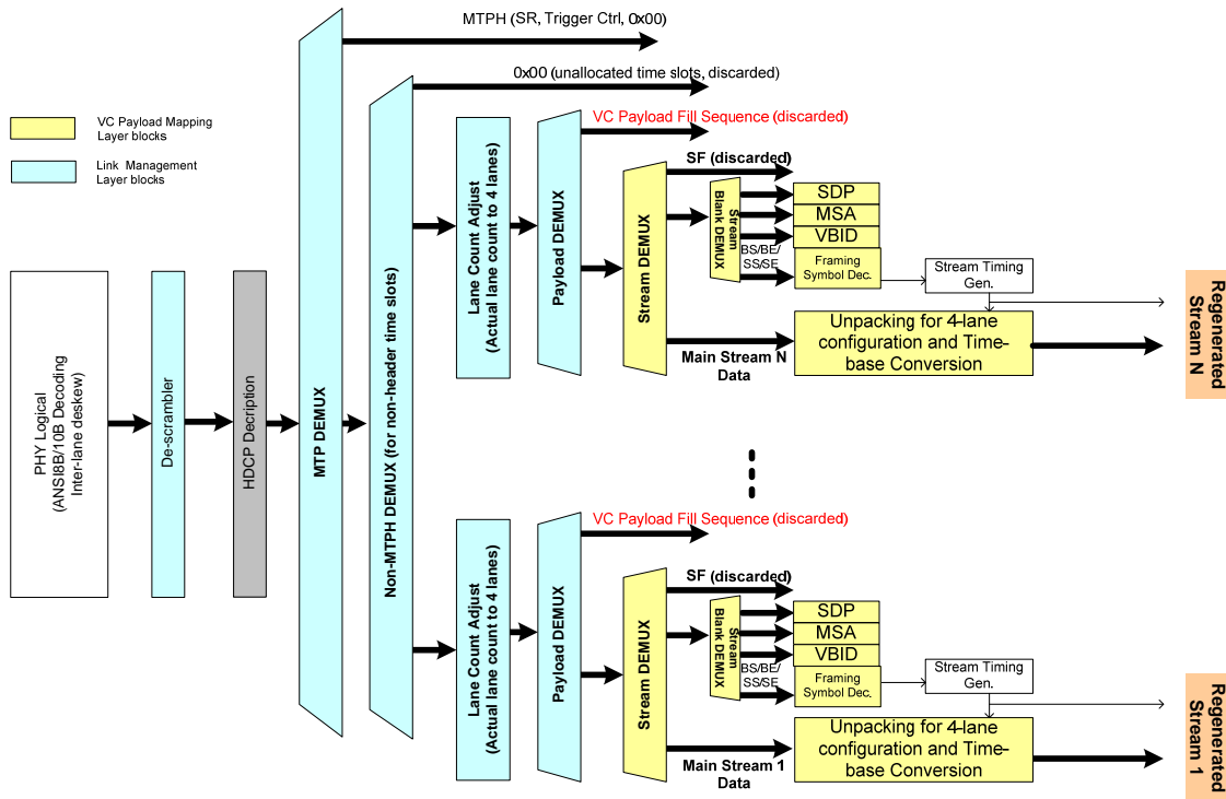
Figure 2-62: Logical Block Diagram of MST DP Sink Device
