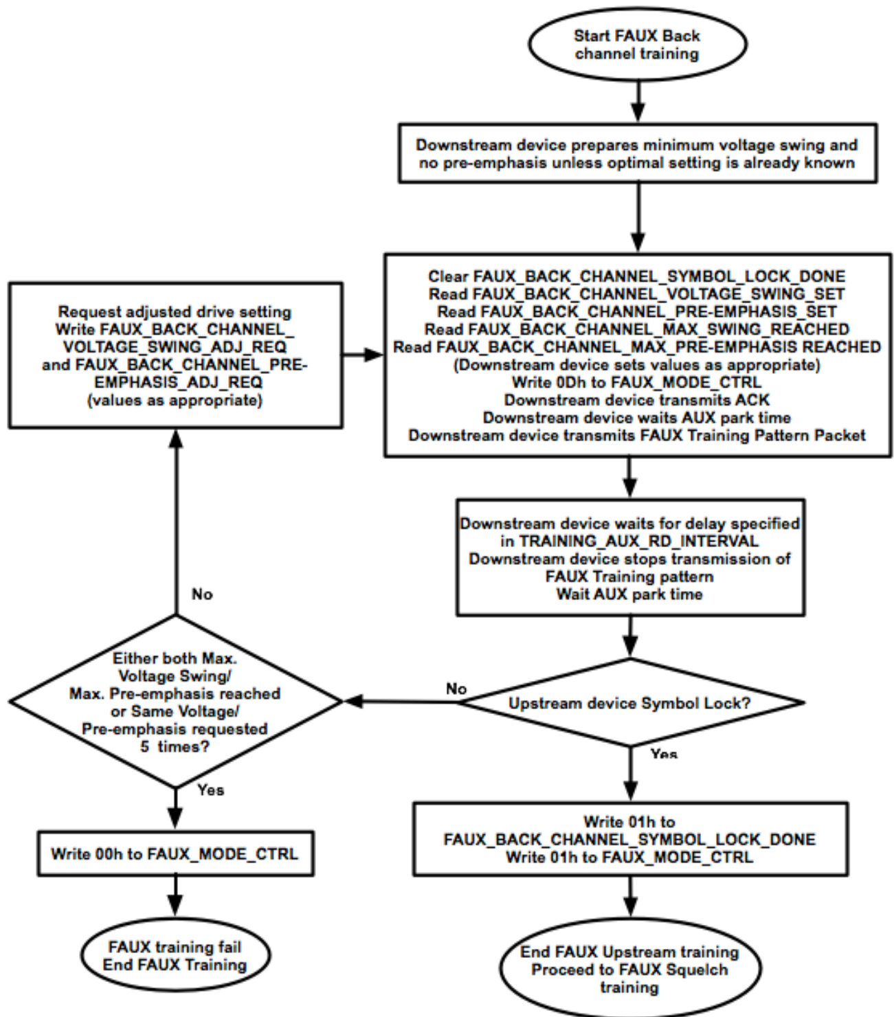
Figure 3-26: FAUX Back Channel Training
