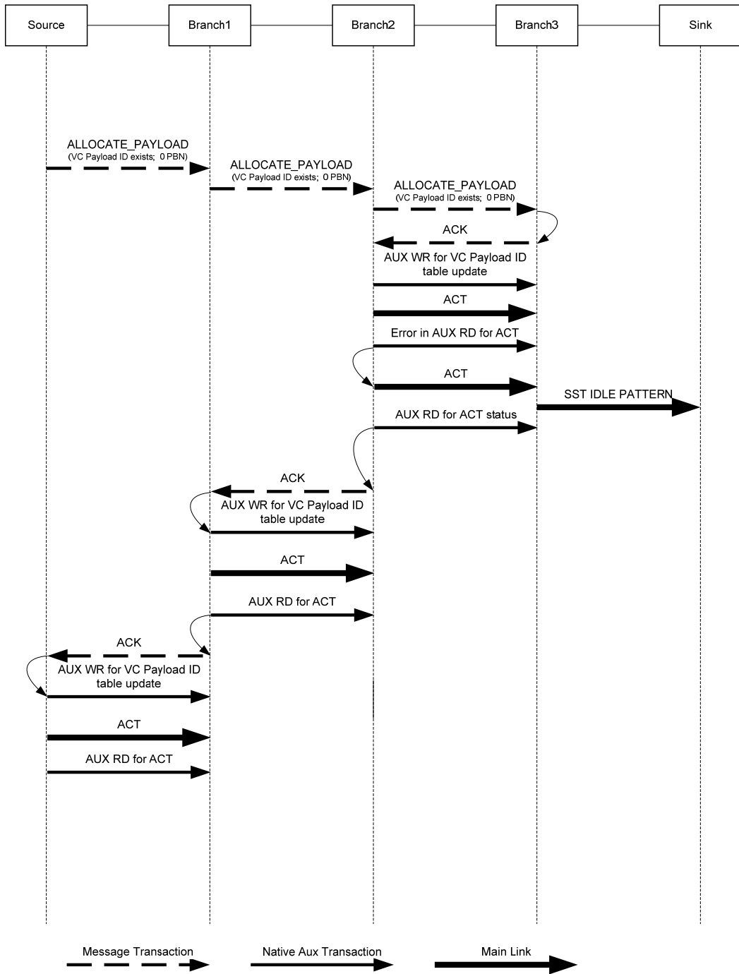
Figure 2-82: Timing Sequence for Deleting a Payload with an Error
