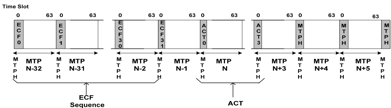
Figure 2-87: ECF Immediately Prior to ACT Sequence
