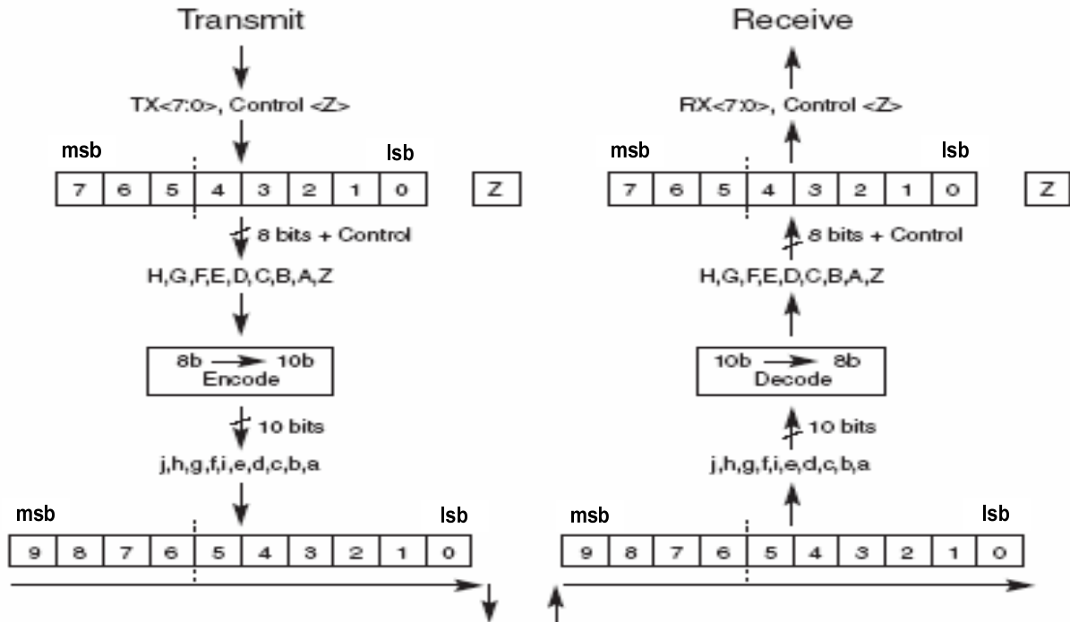
Figure 3-21: Character to Symbol Mapping
