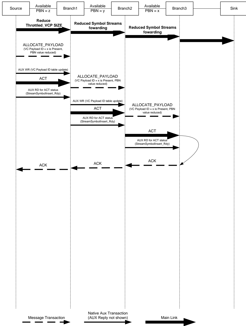
Figure 2-84: Timing Sequence for Reducing the VC Payload Allocation
