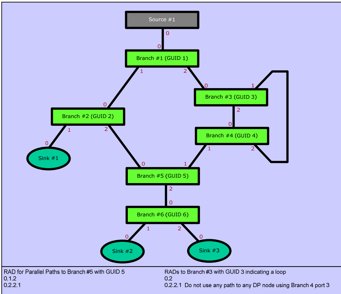
Figure 2-59: MST Topology with a Loop and a Parallel Path
