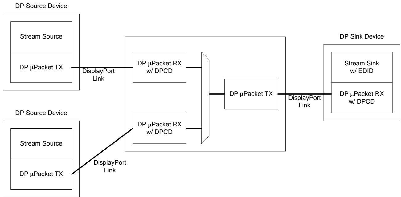
Figure 2-6: Multiple DisplayPort Source Devices to a DisplayPort Sink Device via an Input Switch
