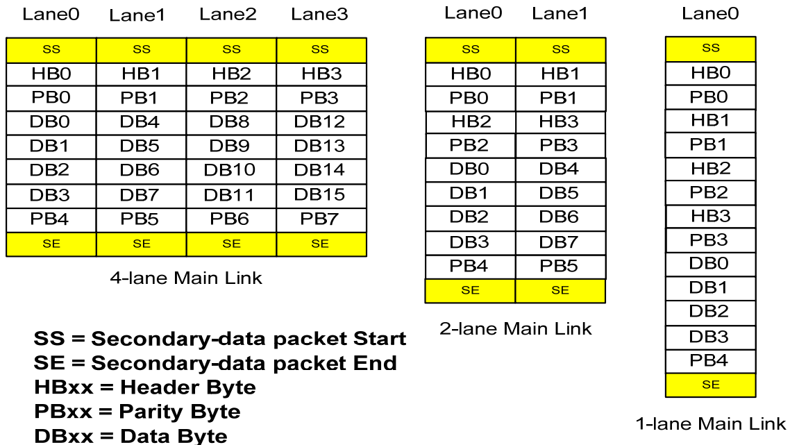
Figure 2-35: Extension Packet Mapping Over the Main Link
