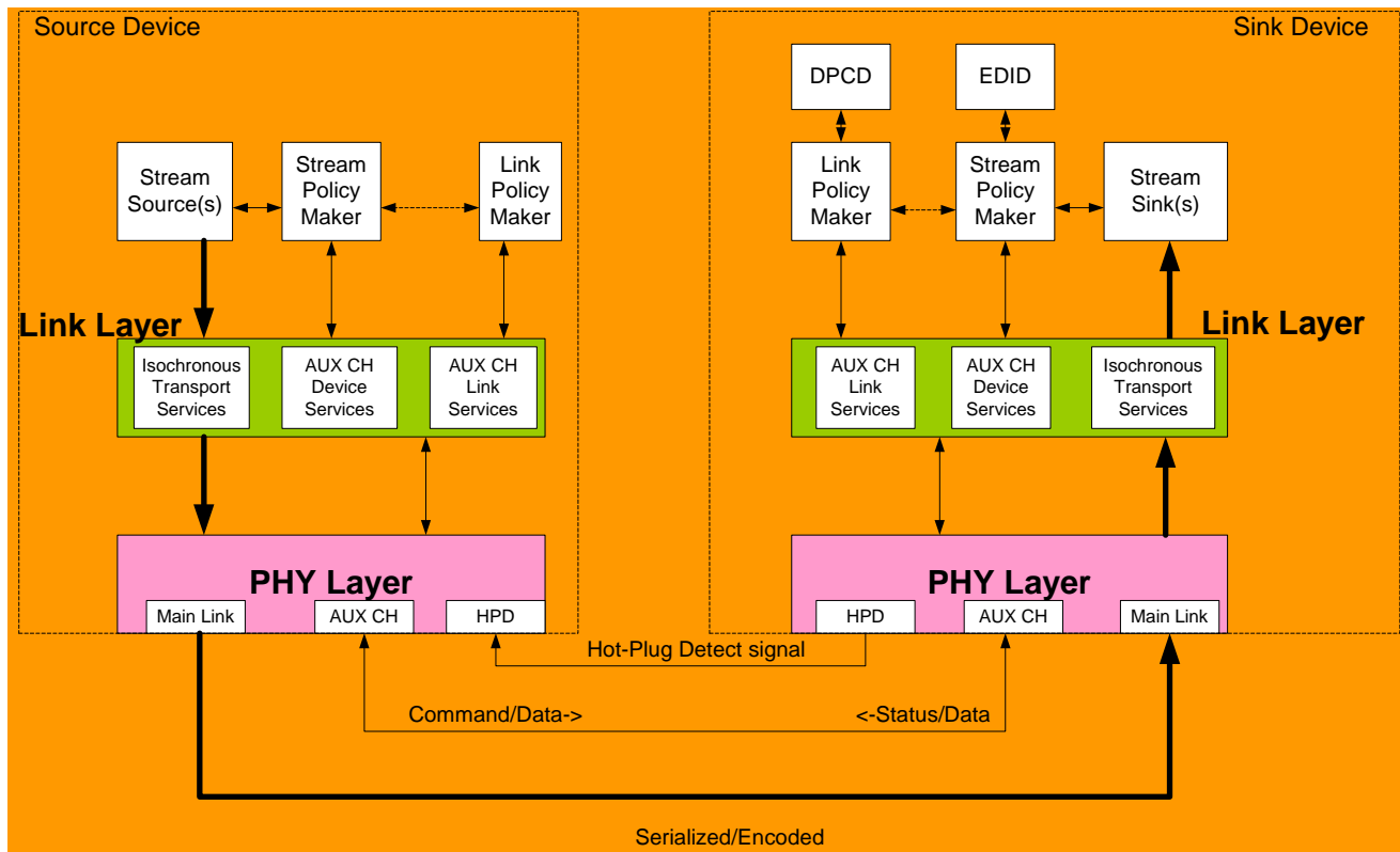
Figure 1-2: Layered Architecture
