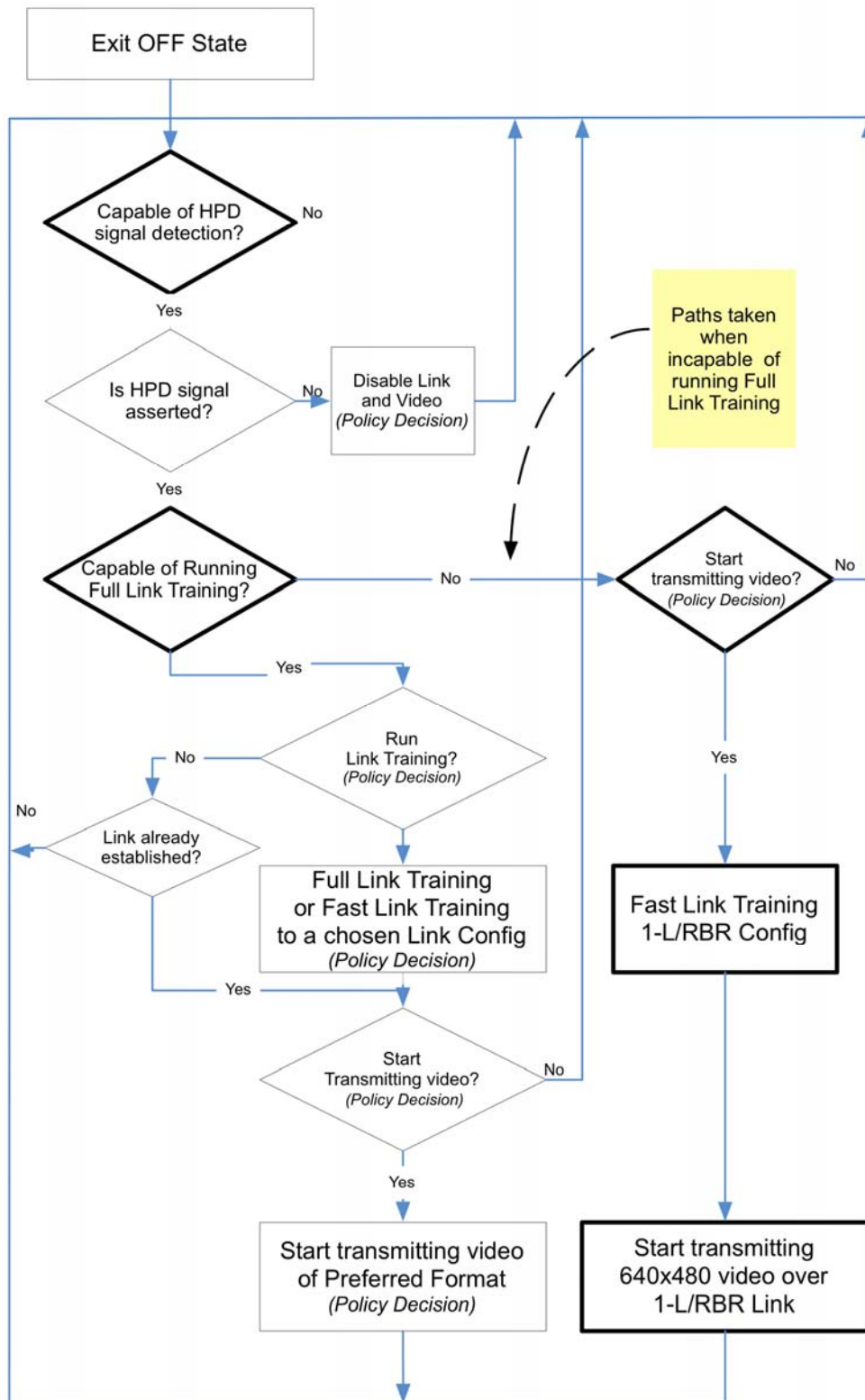
Figure 12-1: Link Quality Management with Fast Link Training
