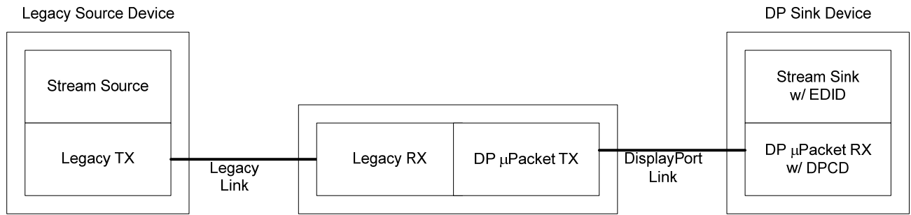
Figure 2-5: Legacy Source Device to DisplayPort Sink Device via a Legacy-to-DisplayPort Converter
