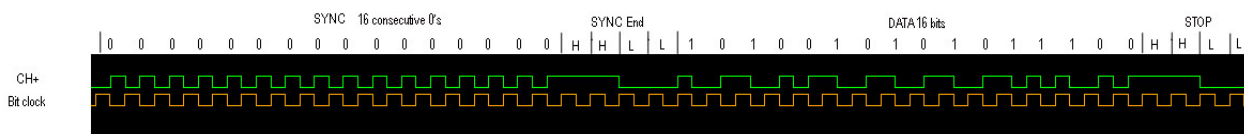
Figure 3-24: AUX CH SYNC Pattern and STOP Condition
