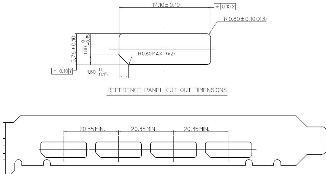
Figure 4-32: Panel Cut Out Reference Dimensions
