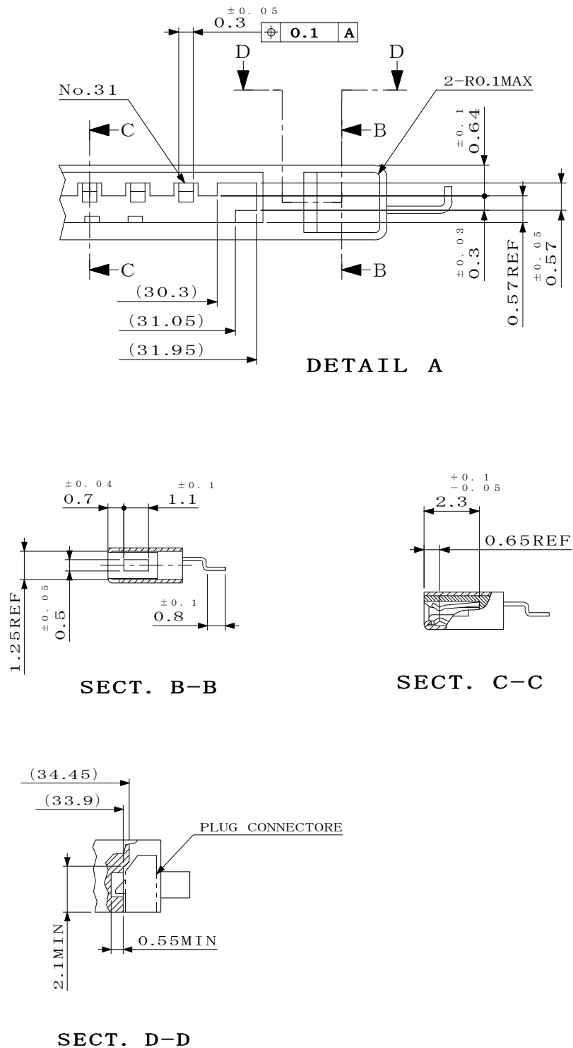
Figure 4-48: Panel-side Internal PCB Mount Receptacle Connector (in unit of mm)
