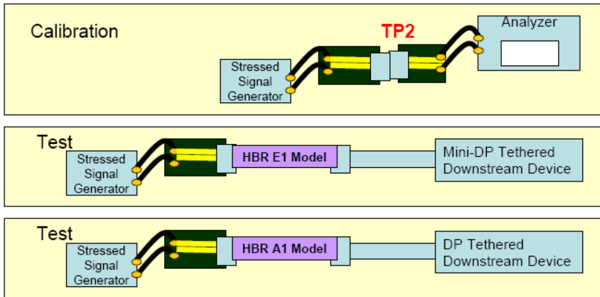
Figure 3-14: FAUX Forward Channel Tethered Receiver Compliance Test Configuration
