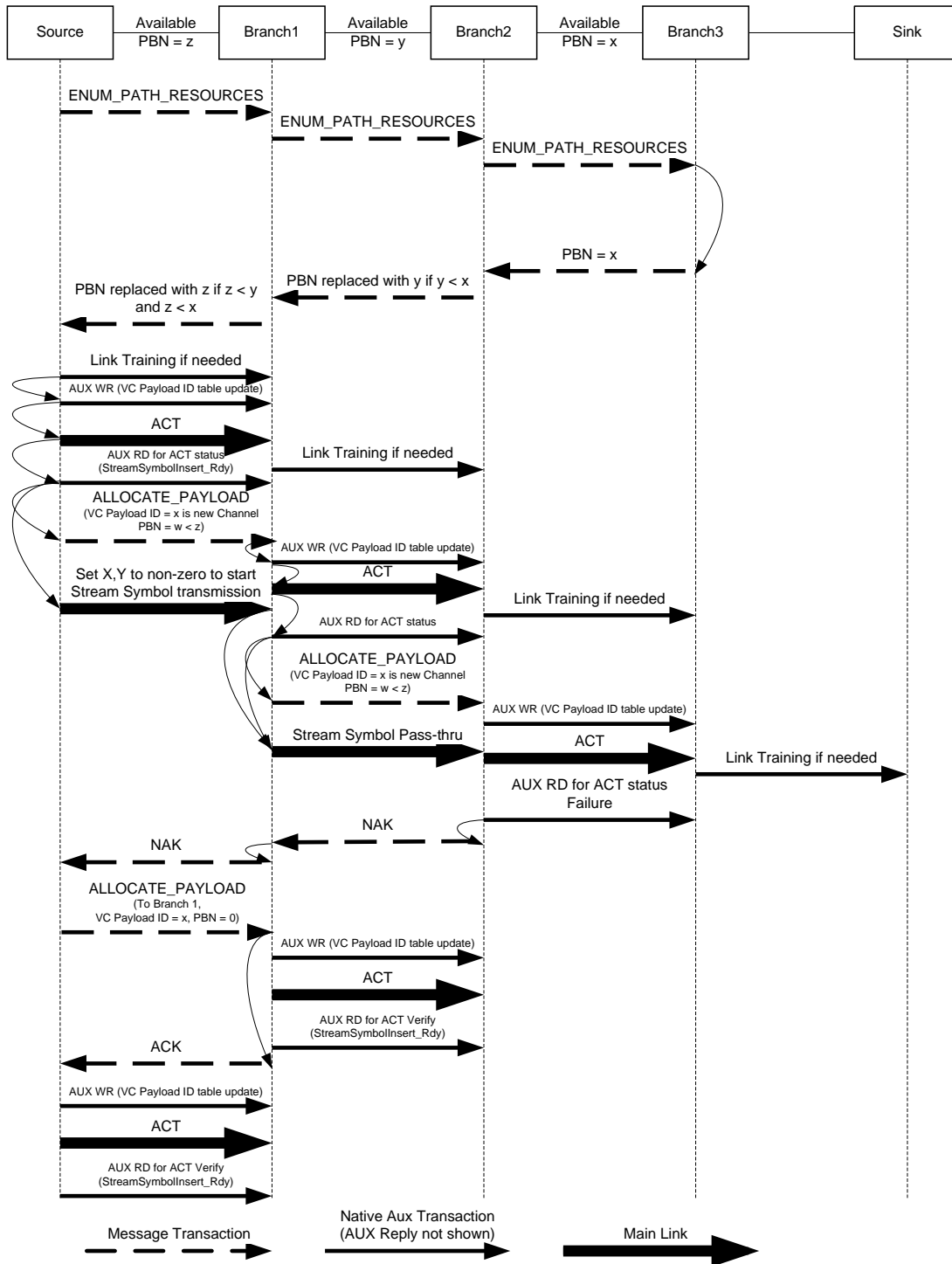
Figure 2-80: Timing Sequence for Adding a New Payload with Error
