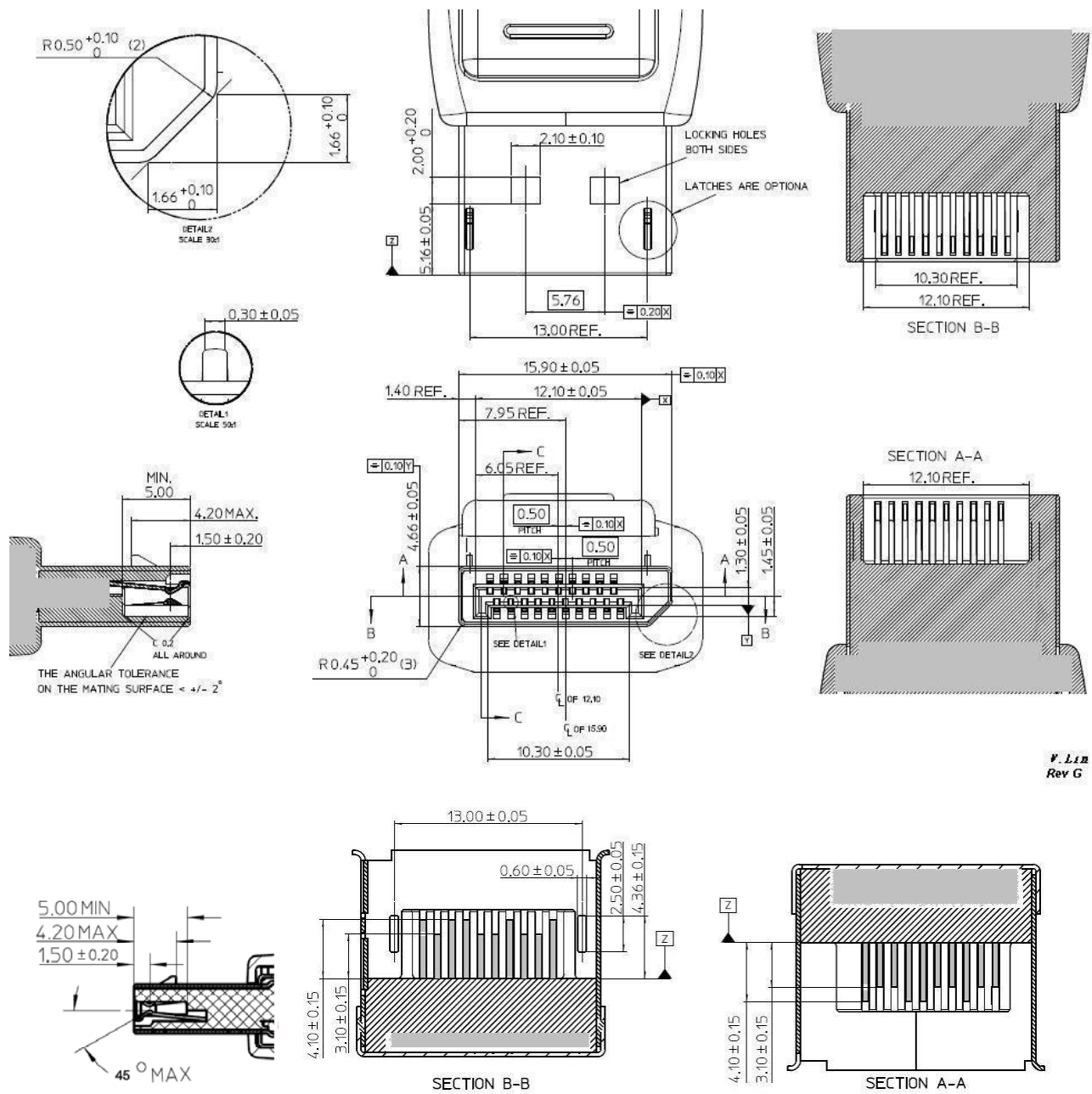
Figure 4-26: DisplayPort External Cable-Connector Assembly Drawings
