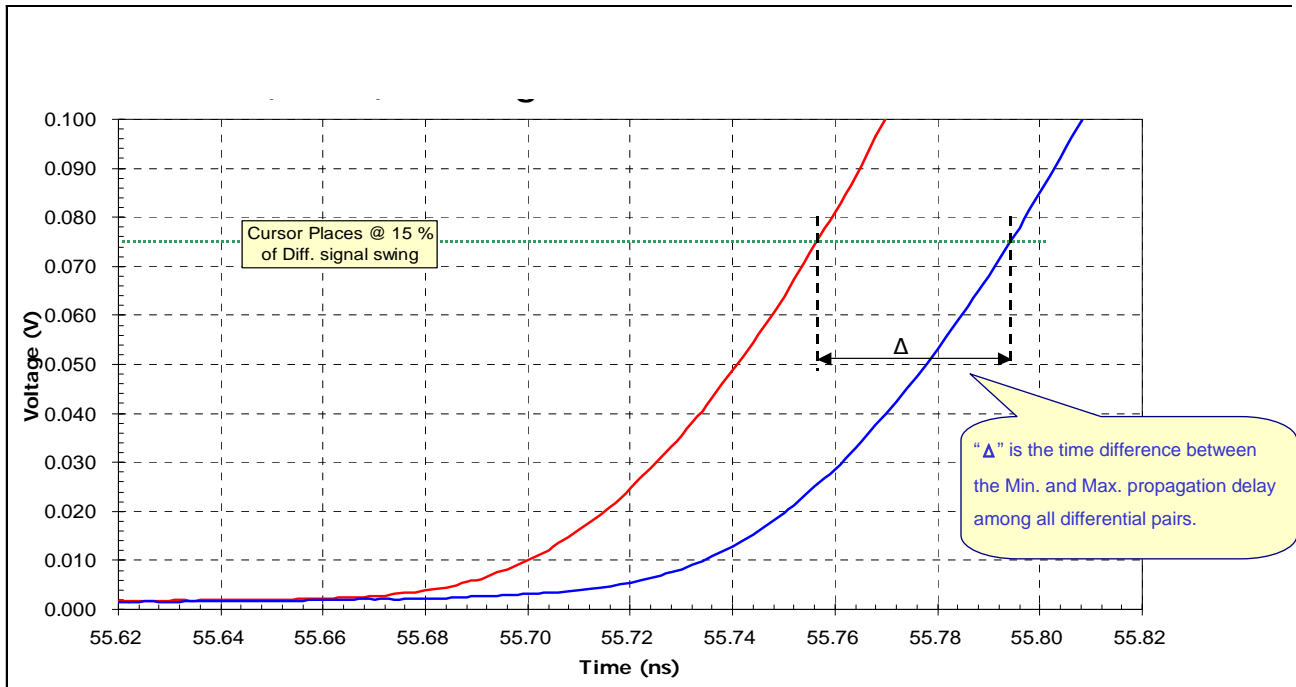
Figure 4-18: Inter-Pair Skew Measurement Method
