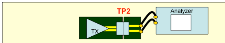
Figure 3-6: HBR Upstream Device Compliance Test Configuration
