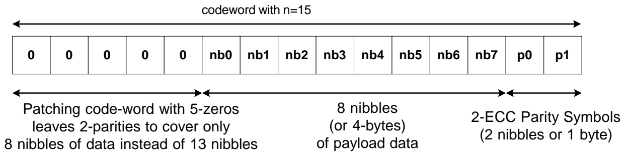
Figure 2-41: Makeup of 15 Nibble Code-Word for Packet Payload
