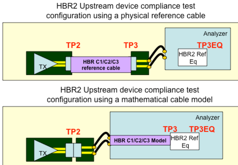
Figure 3-4: HBR2 Upstream Device Compliance Test Configuration
