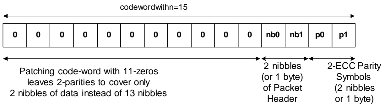
Figure 2-42: Makeup of 15 Nibble Code-Word for Packet Header
