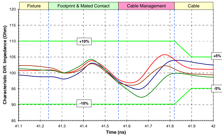
Figure 4-8: Differential Impedance Profile Measurement Data Example
