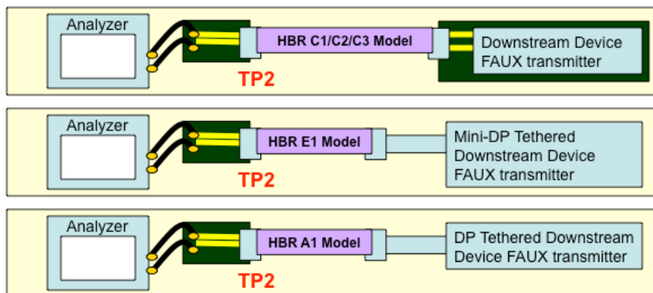
Figure 3-15: FAUX Back Channel Transmitter Compliance Test Configuration
