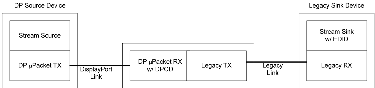
Figure 2-4: DisplayPort Source Device to Legacy Sink via DisplayPort-to-Legacy Converter
