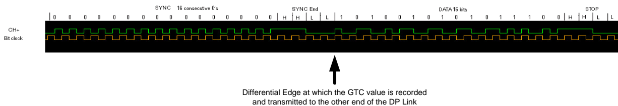
Figure 2-104: GTC Value Measurement Point by GTC Master When AUX CH Running in Manchester Transaction Format
